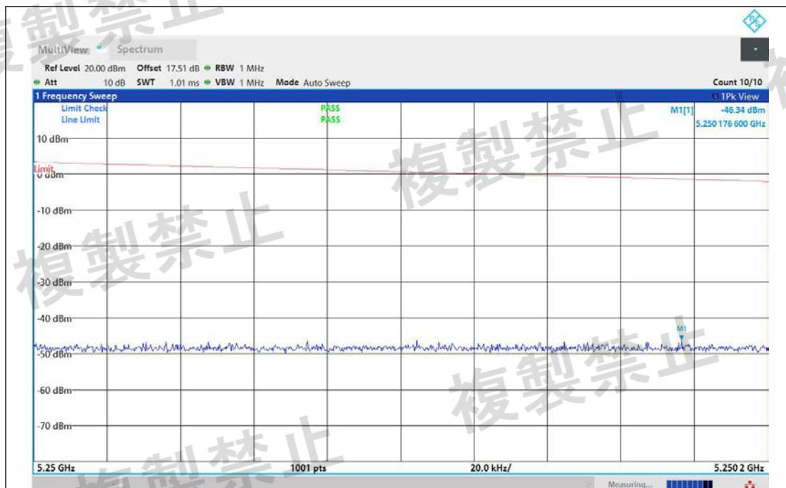
NTNV-11AX20MIMO-Ant1-5180-5250~5250.2-PASS
