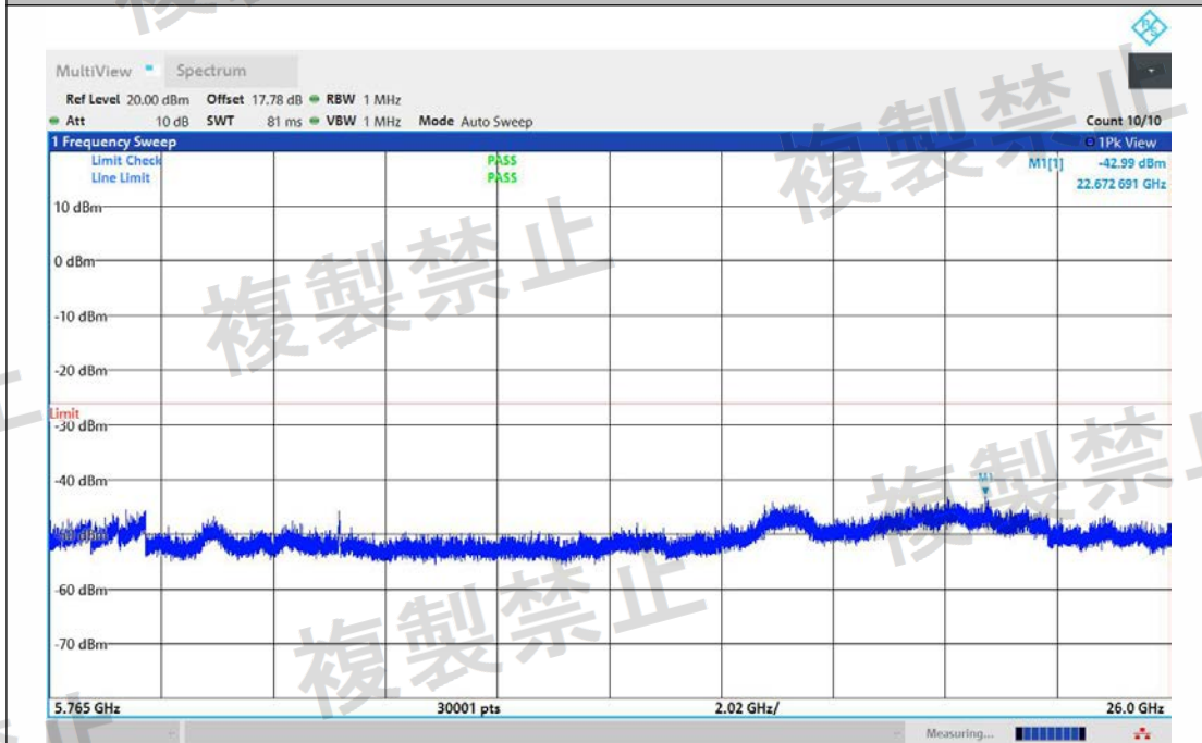
NTNV-11AC20MIMO-Ant2-5500-5765~26000-PASS
