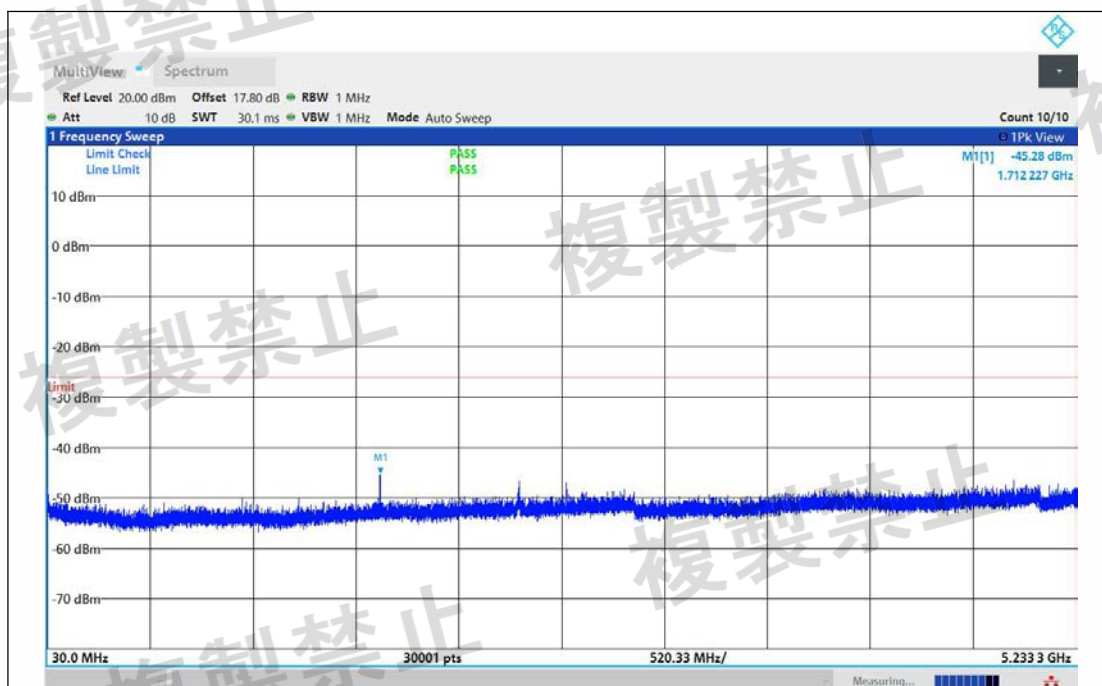
NTNV-11AC20MIMO-Ant1-5280-30~5233.3-PASS
