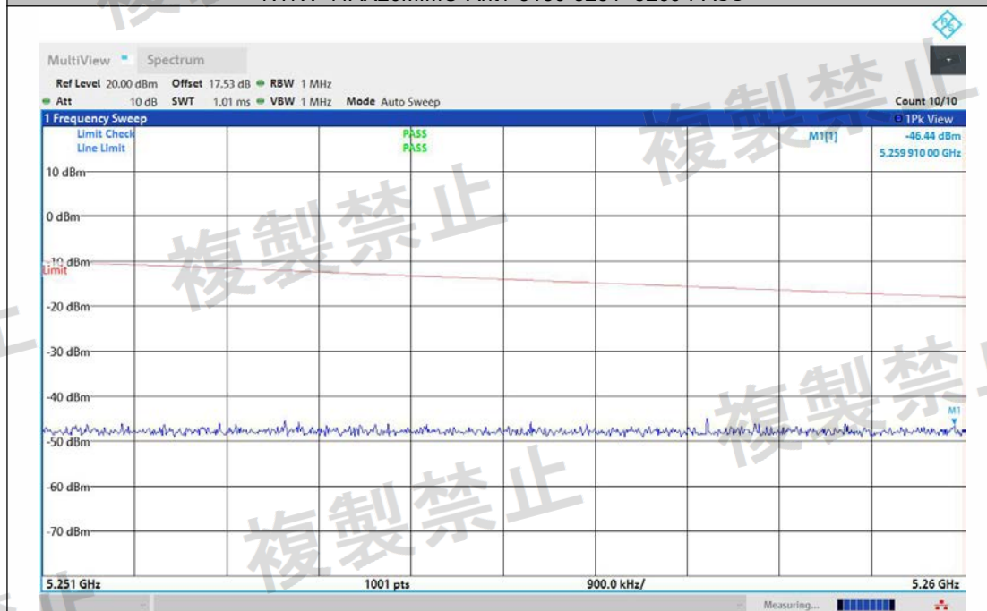
NTNV-11AX20MIMO-Ant2-5180-5251~5260-PASS
