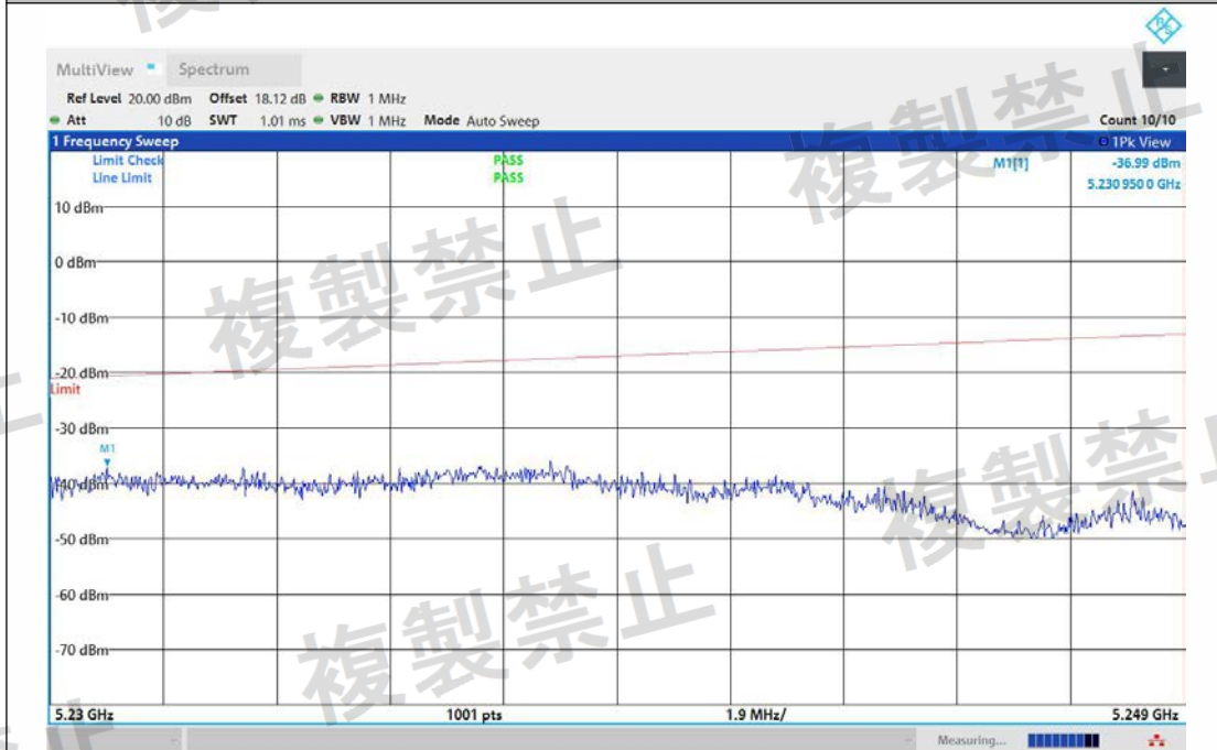
NTNV-11AC40MIMO-Ant2-5310-5230~5249-PASS
