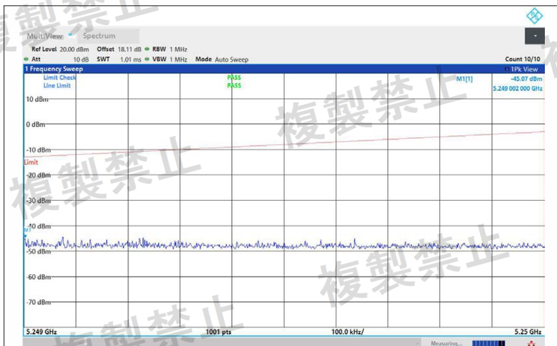
NTNV-11AC40MIMO-Ant1-5310-5249~5250-PASS
