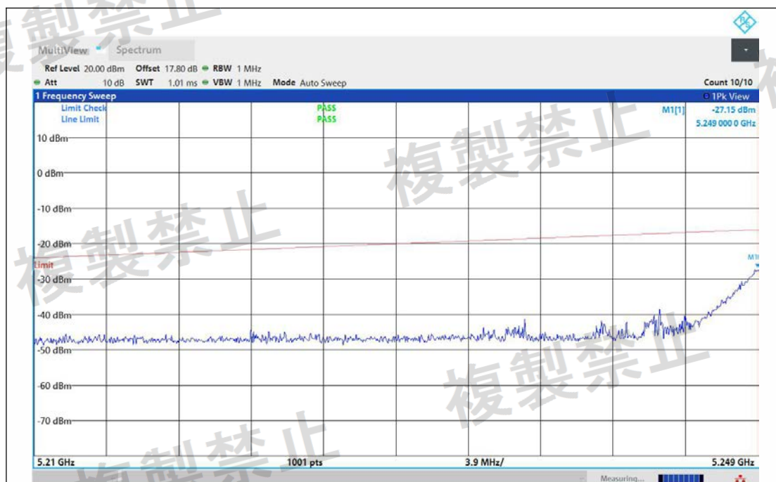
NTNV-11AC80MIMO-Ant1-5290-5210~5249-PASS
