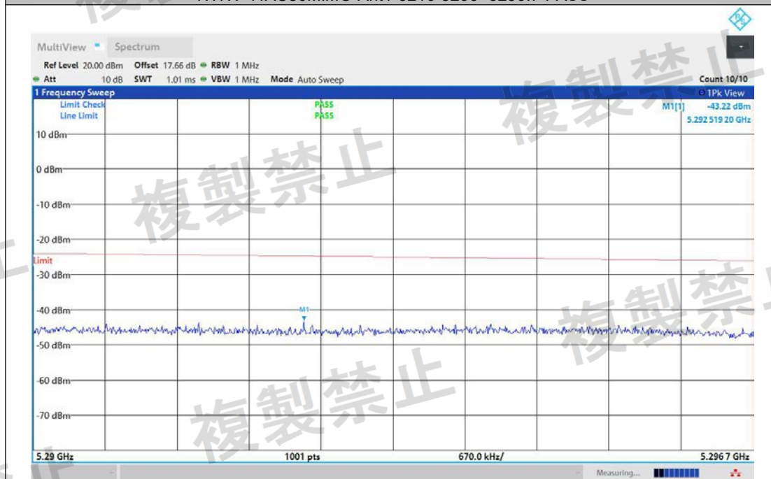
NTNV-11AC80MIMO-Ant2-5210-5290~5296.7-PASS
