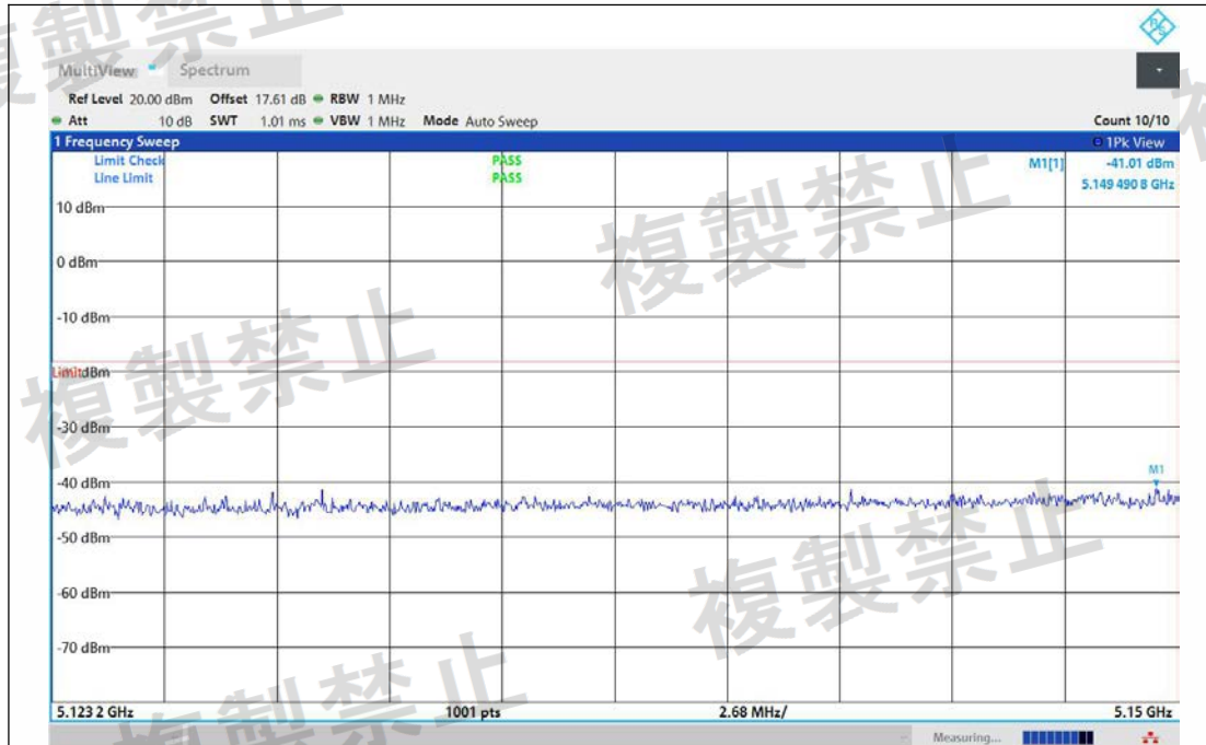
NTNV-11AC80MIMO-Ant1-5210-5123.2~5150-PASS
