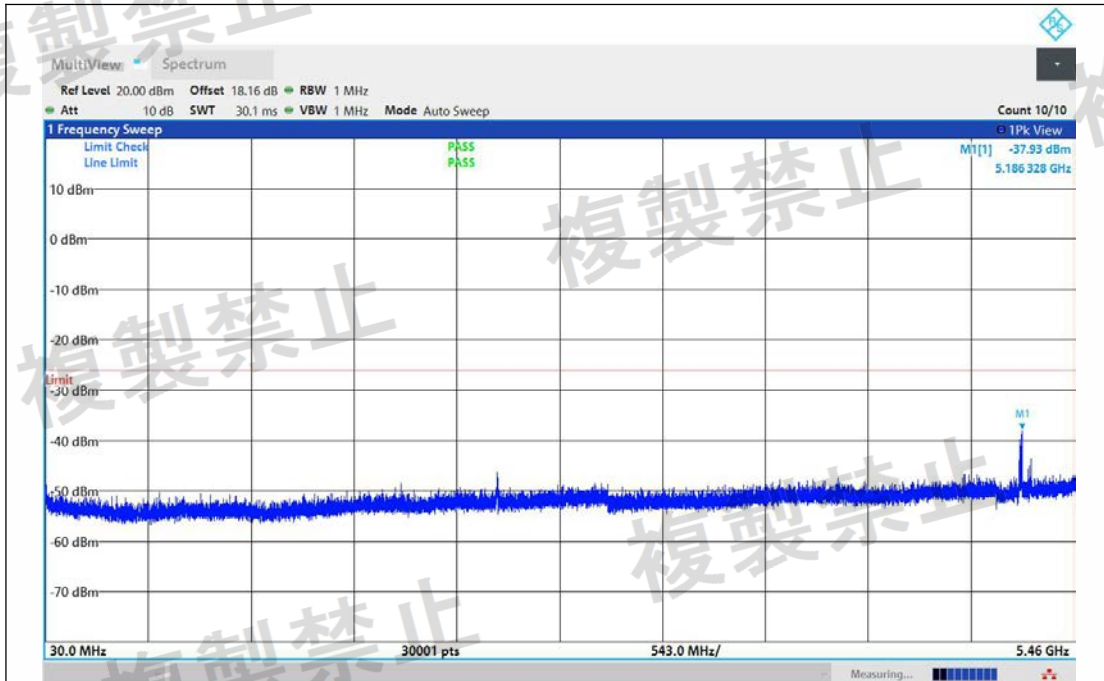
NTNV-11AC20MIMO-Ant1-5580-30~5460-PASS
