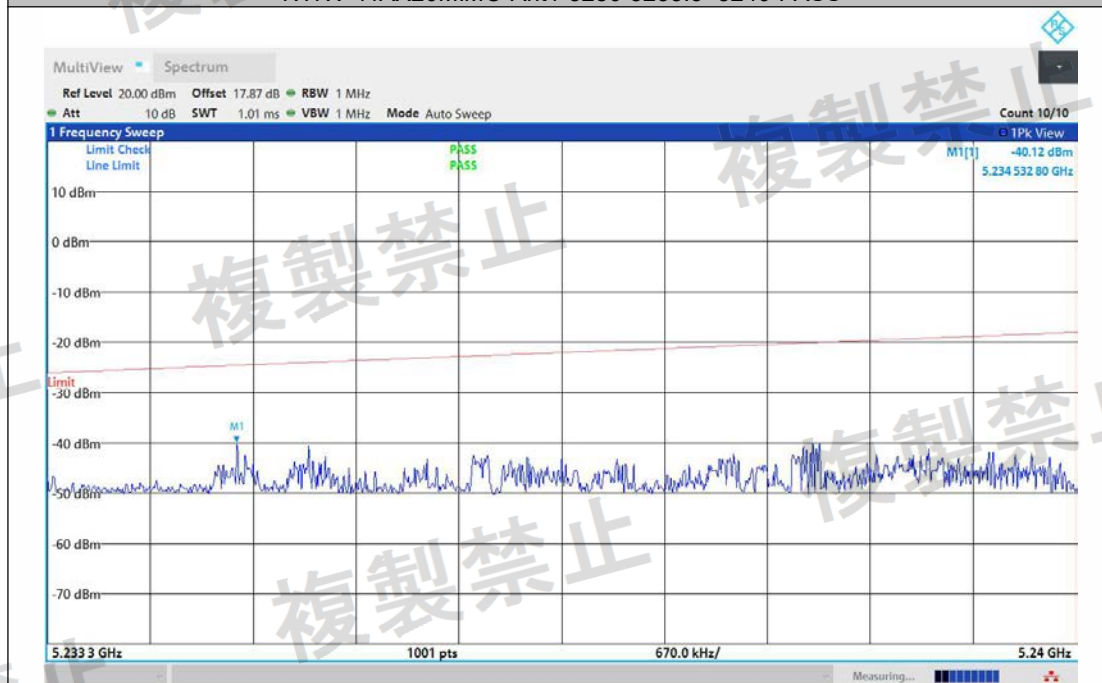
NTNV-11AX20MIMO-Ant2-5280-5233.3~5240-PASS
