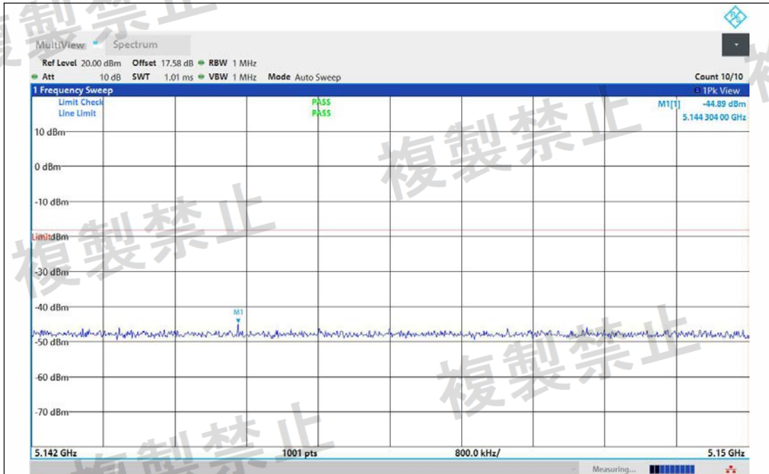
NTNV-11AX20MIMO-Ant1-5240-5142~5150-PASS
