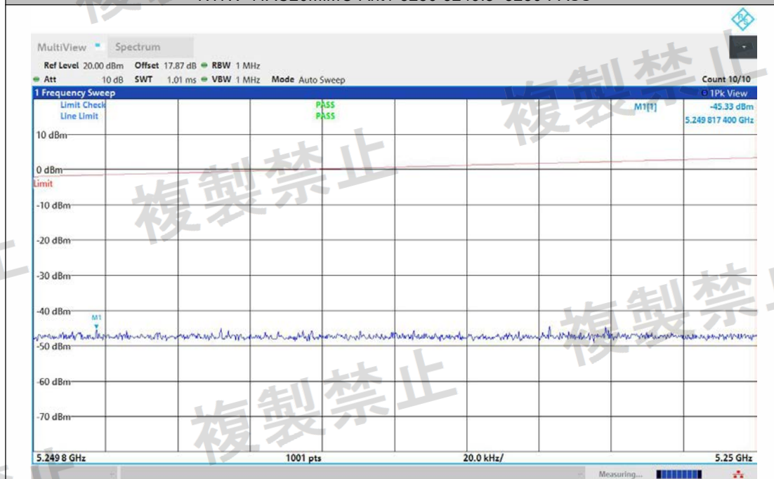
NTNV-11AC20MIMO-Ant2-5280-5249.8~5250-PASS
