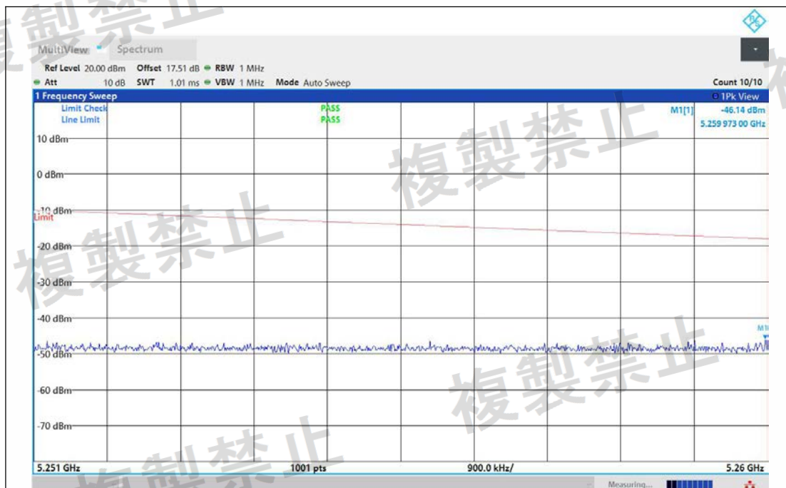
NTNV-11AX20MIMO-Ant1-5180-5251~5260-PASS
