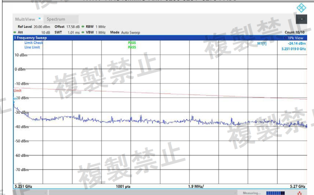
NTNV-11AC40MIMO-Ant2-5230-5251~5270-PASS
