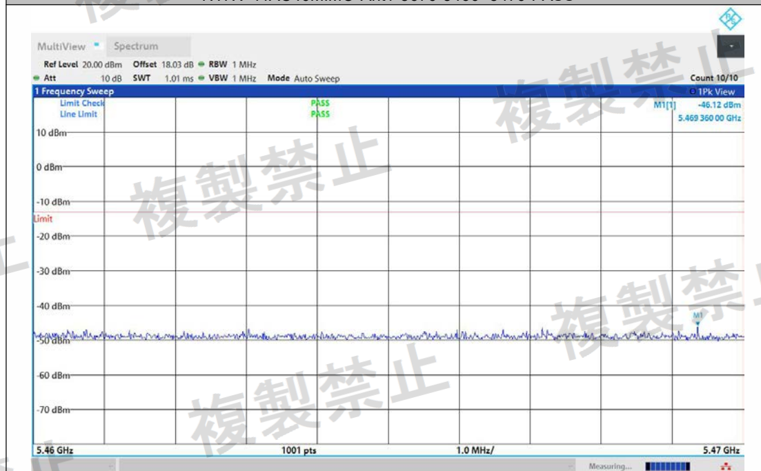
NTNV-11AC40MIMO-Ant2-5670-5460~5470-PASS
