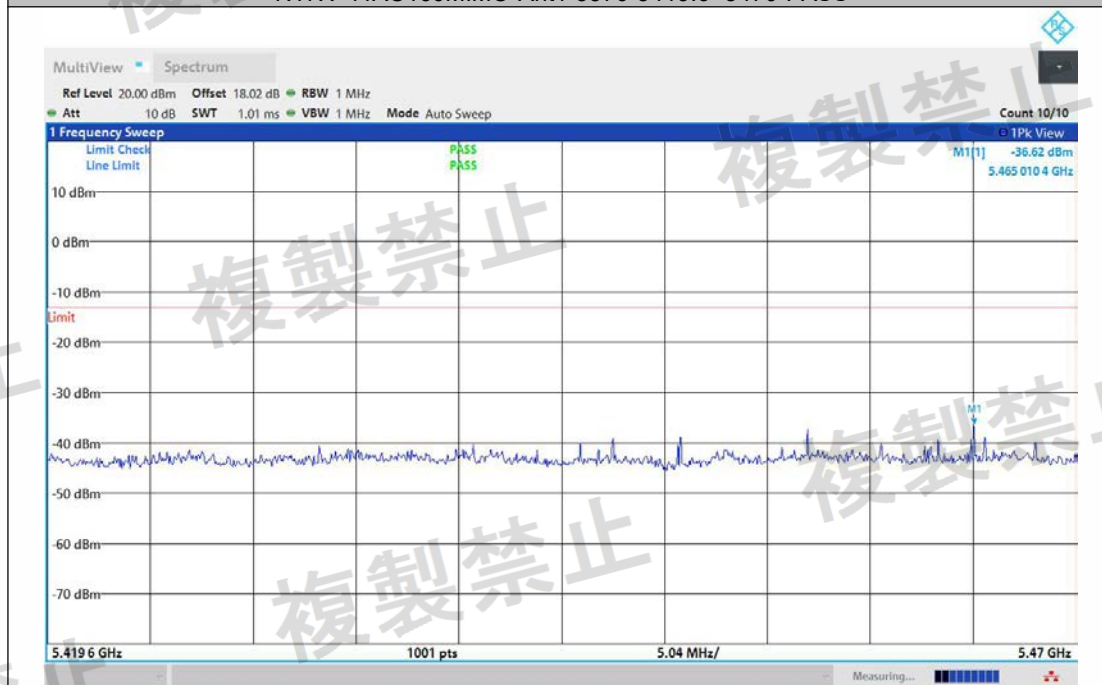
NTNV-11AC160MIMO-Ant2-5570-5419.6~5470-PASS
