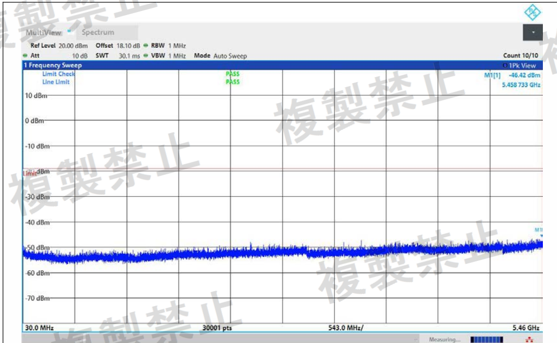
NTVN-11AC40MIMO-Ant1-5670-30~5460-PASS
