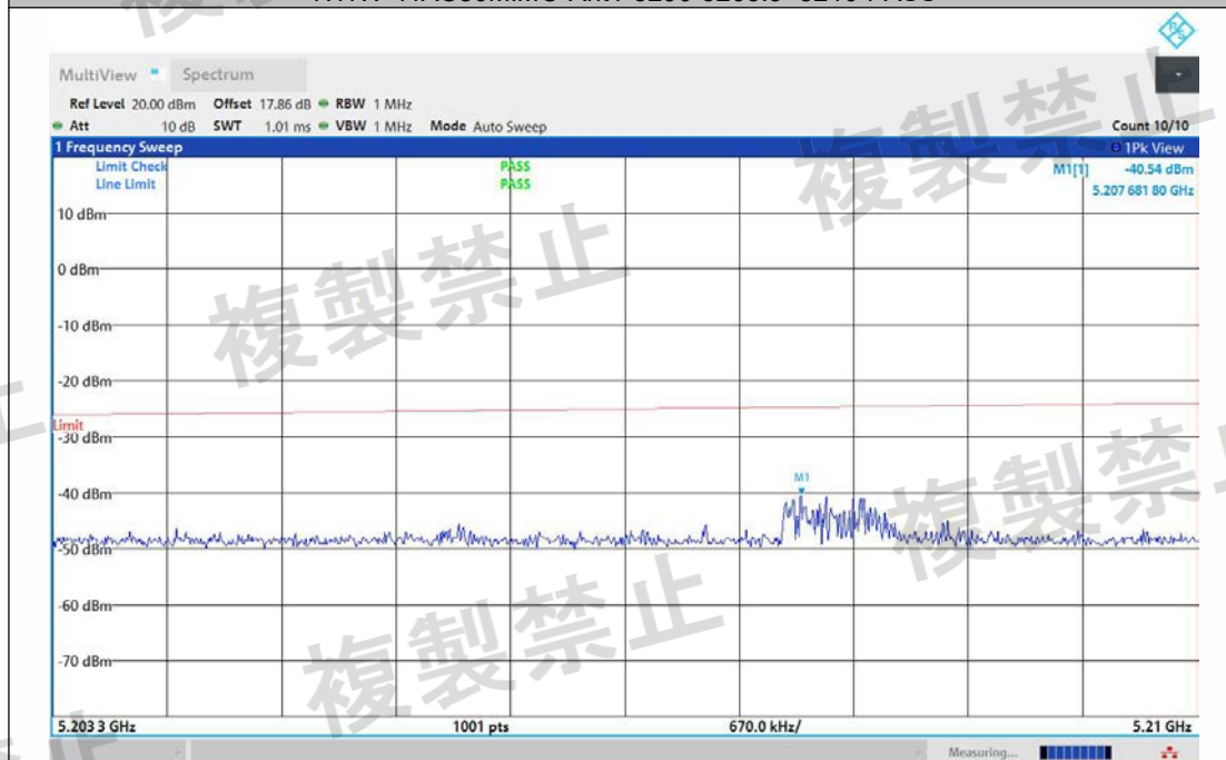
NTNV-11AC80MIMO-Ant2-5290-5203.3~5210-PASS
