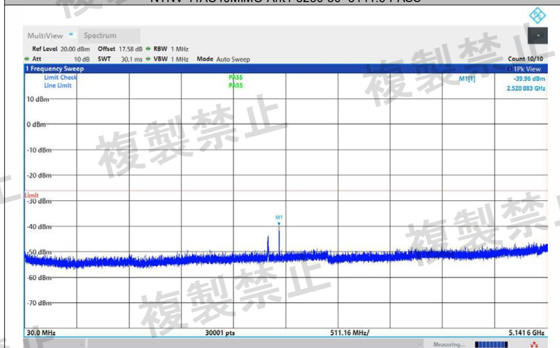
NTNV-11AC40MIMO-Ant2-5230-30~5141.6-PASS
