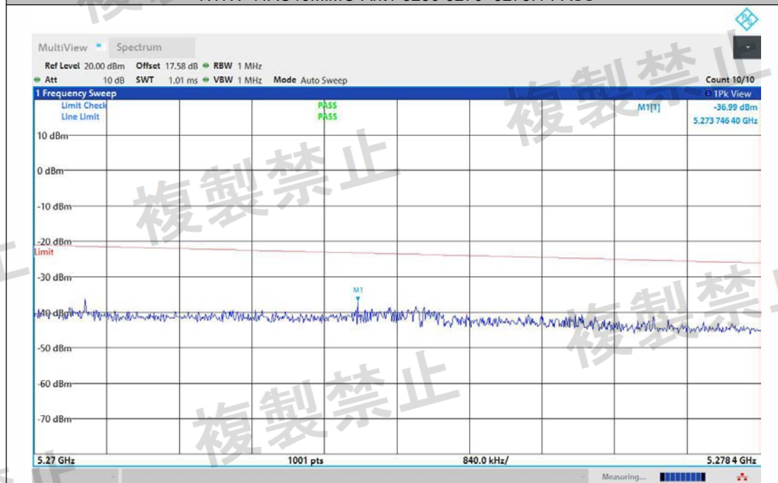
NTNV-11AC40MIMO-Ant2-5230-5270~5278.4-PASS
