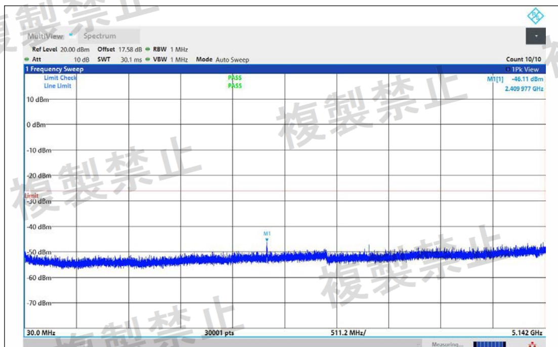
NTNV-11AX20MIMO-Ant1-5200-30~5142-PASS
