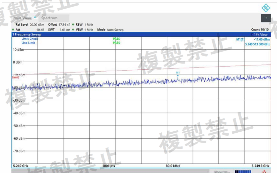
NTNV-11AX20MIMO-Ant1-5260-5249~5249.8-See table below
