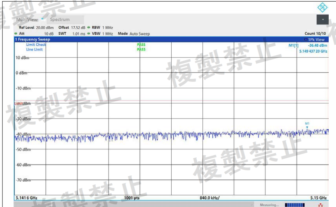
NTNV-11AC40MIMO-Ant1-5190-5141.6~5150-PASS
