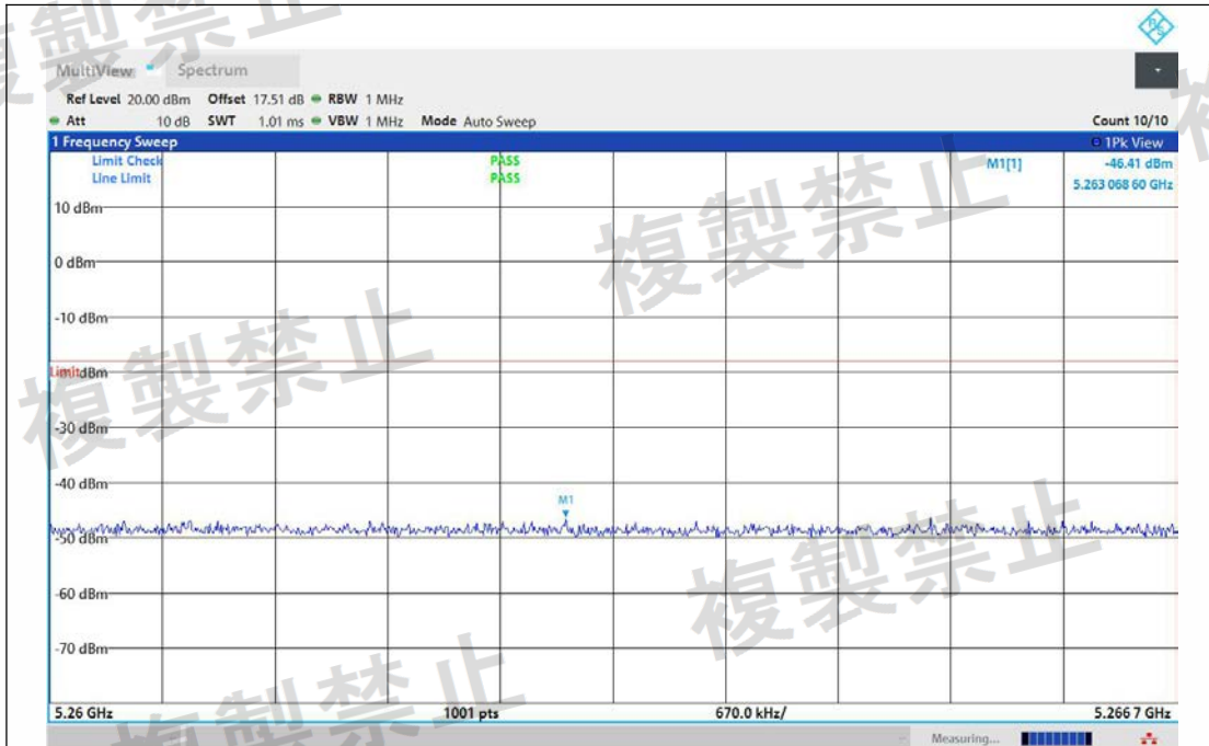
NTNV-11AX20MIMO-Ant1-5180-5260~5266.7-PASS
