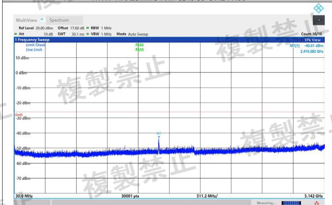
NTNV-11AX20MIMO-Ant2-5240-30~5142-PASS
