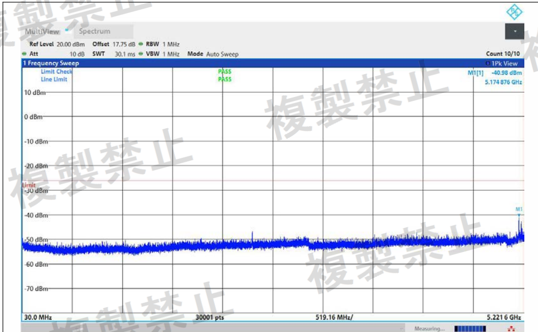
NTNV-11AC40MIMO-Ant1-5270-30~5221.6-PASS
