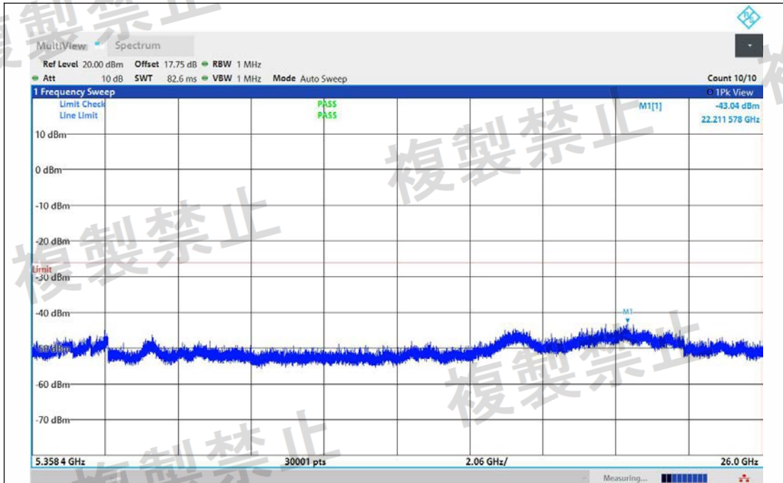
NTNV-11AC40MIMO-Ant1-5270-5358.4~26000-PASS
