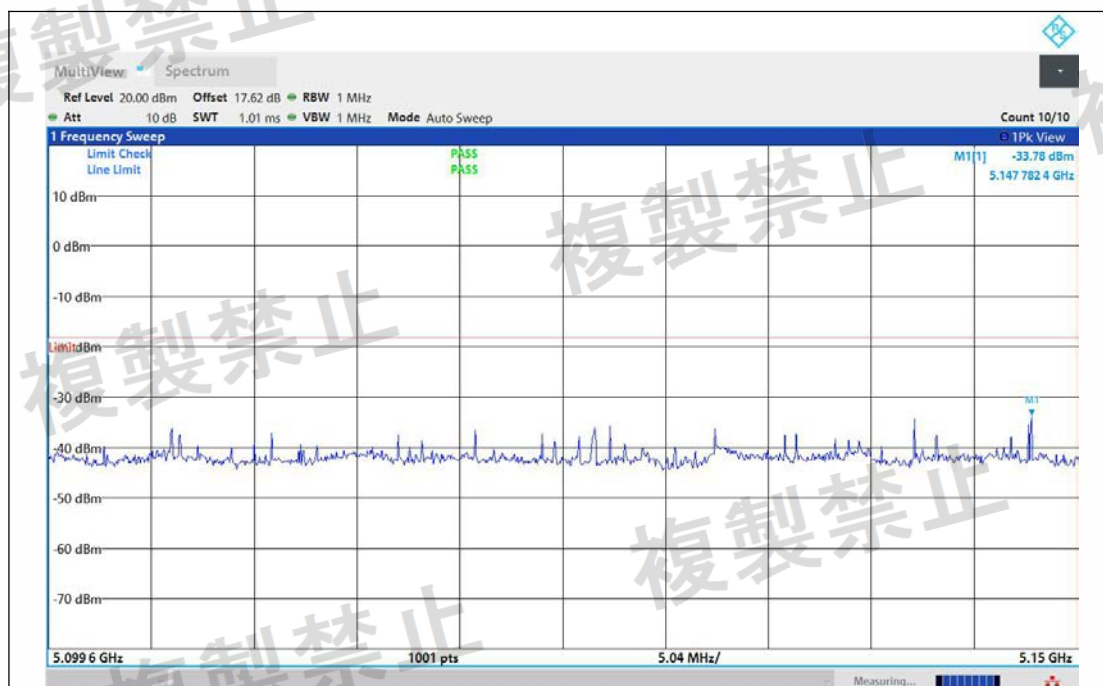
NTNV-11AC160MIMO-Ant1-5250-5099.6~5150-PASS
