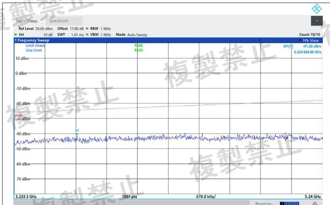
NTNV-11AX20MIMO-Ant1-5280-5233.3~5240-PASS
