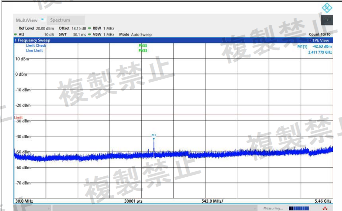
NTNV-11AC20MIMO-Ant2-5580-30~5460-PASS
