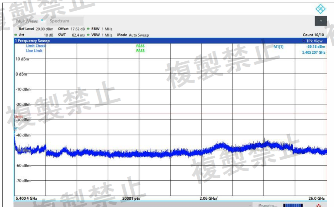
NTNV-11AC160MIMO-Ant1-5250-5400.4~26000-PASS
