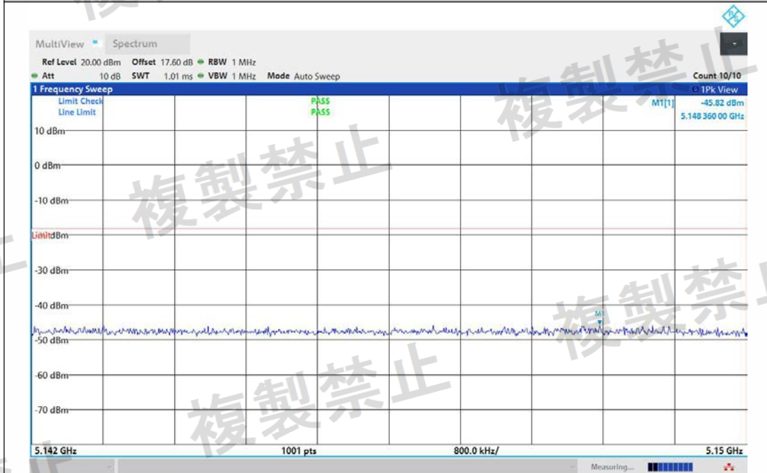
NTNV-11AX20MIMO-Ant2-5240-5142~5150-PASS
