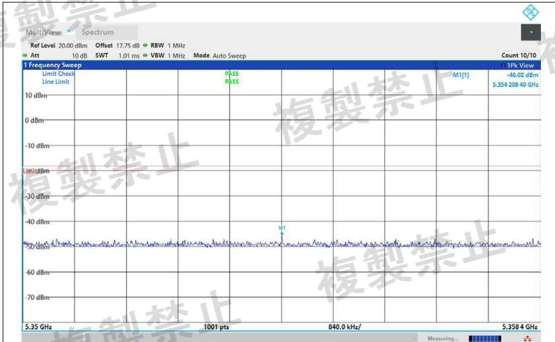
NTNV-11AC40MIMO-Ant1-5270-5350~5358.4-PASS
