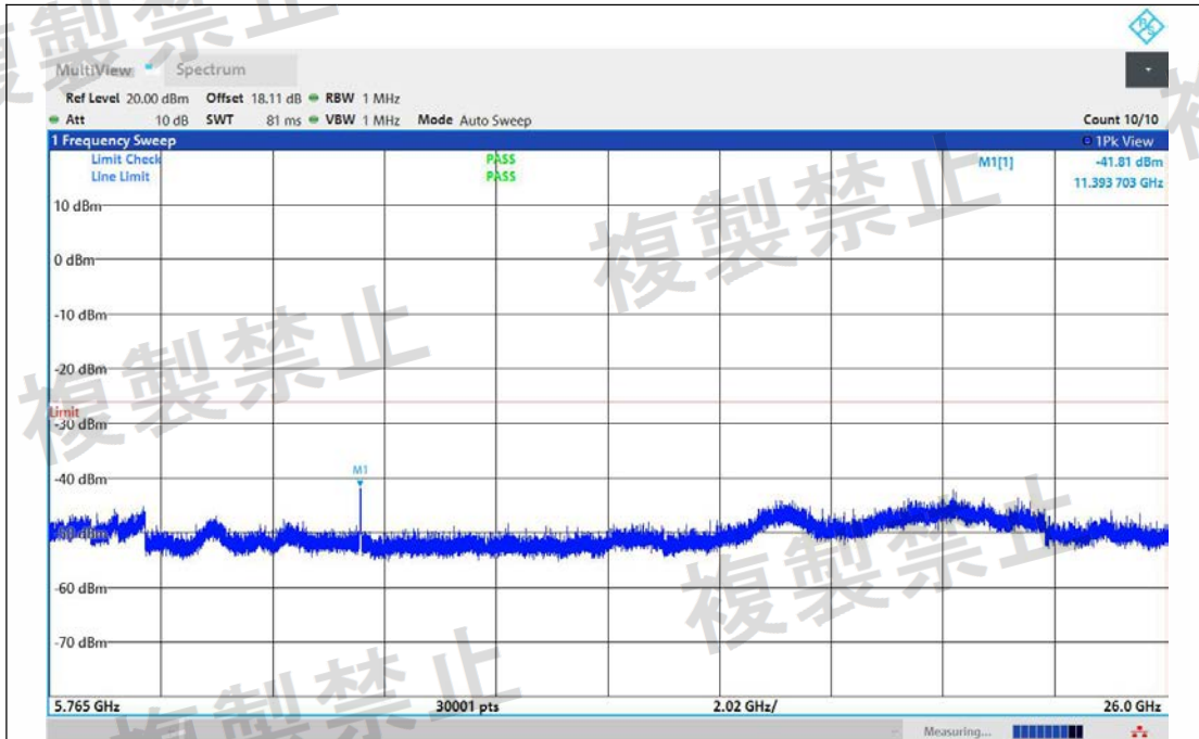
NTNV-11AC20MIMO-Ant1-5700-5765~26000-PASS
