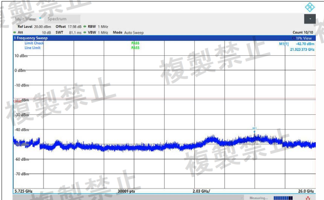
NTNV-11AC160MIMO-Ant1-5570-5725~26000-PASS
