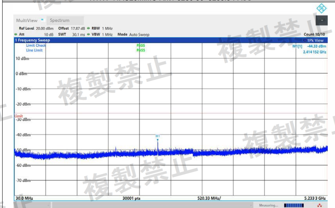
NTNV-11AC20MIMO-Ant2-5280-30~5233.3-PASS
