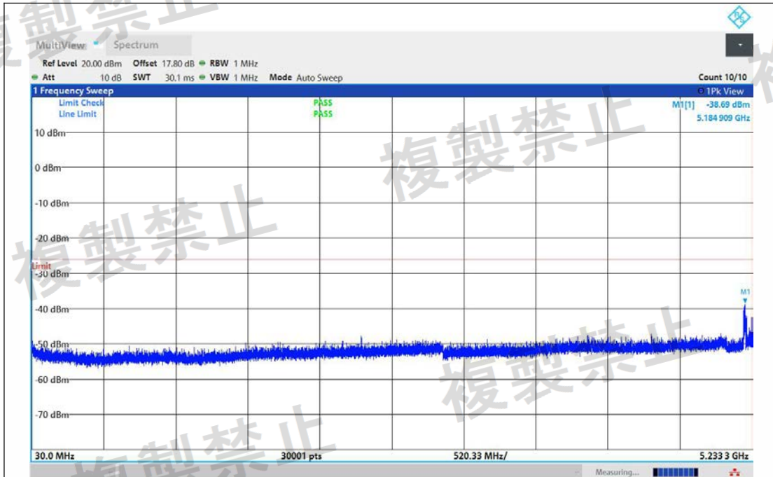
NTNV-11AX20MIMO-Ant1-5280-30~5233.3-PASS
