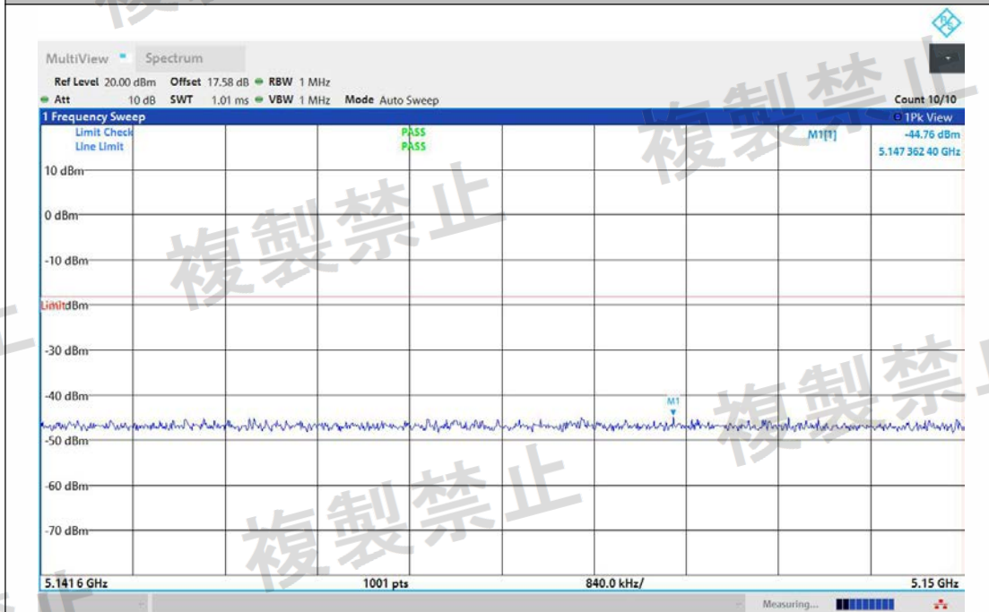
NTNV-11AC40MIMO-Ant2-5230-5141.6~5150-PASS
