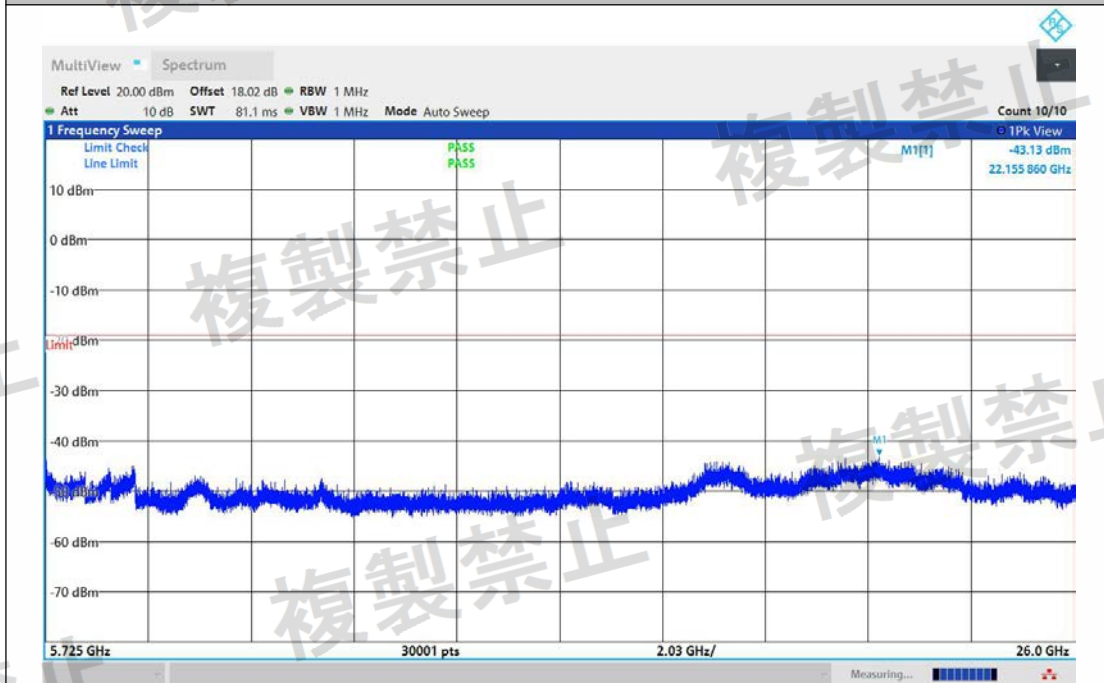
NTNV-11AC160MIMO-Ant2-5570-5725~26000-PASS
