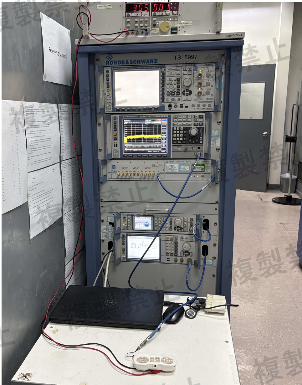
Test Setup
