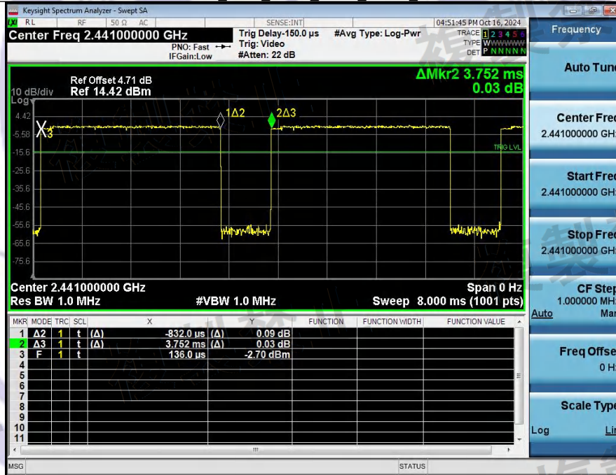
Dwell Time_NVNT_ANT1_2-DH5_2441
