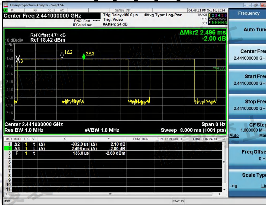
Dwell Time_NVNT_ANT1_1-DH3_2441
