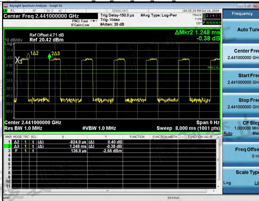
Dwell Time_NVNT_ANT1_3-DH1_2441
