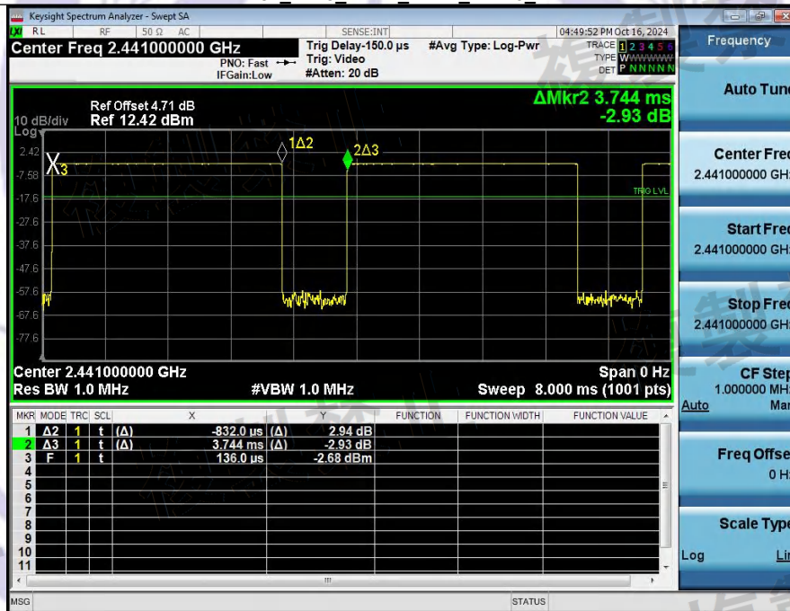
Dwell Time_NVNT_ANT1_1-DH5_2441
