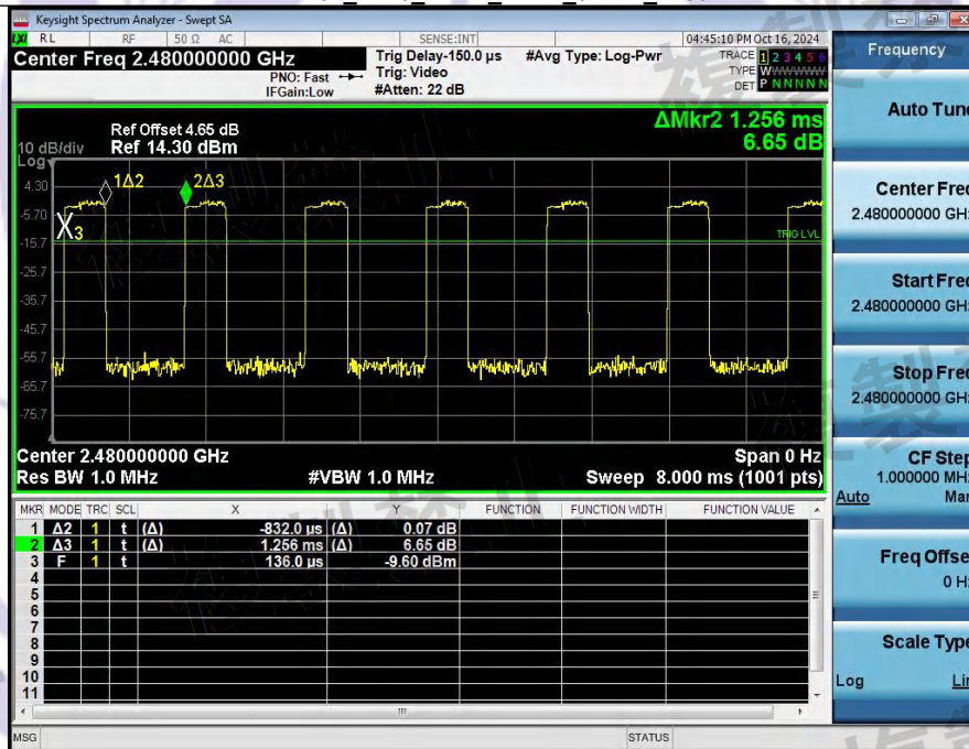
Dwell Time_NVNT_ANT1_3-DH1_2480
