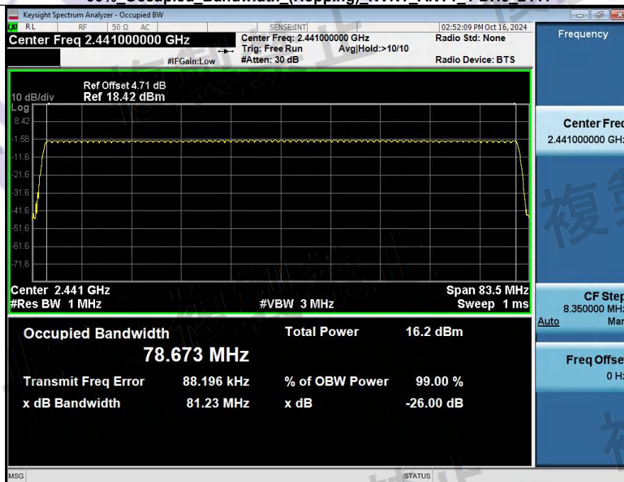
99% Occupied Bandwidth (Hopping) NVNT_ANT1_1-DH3 2441
