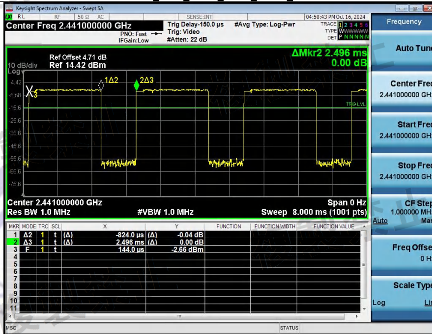
Dwell Time_NVNT_ANT1_2-DH3_2441
