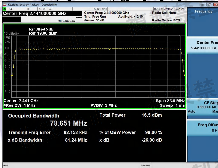
99% Occupied Bandwidth (Hopping) NVNT_ANT1_1-DH1 2441
