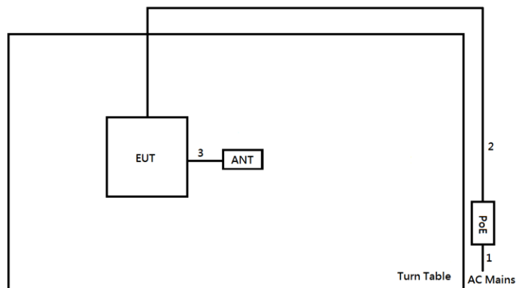
Test Setup Diagram - Radiated Test (Sample 2_Panel 1 Antenna) - TX
