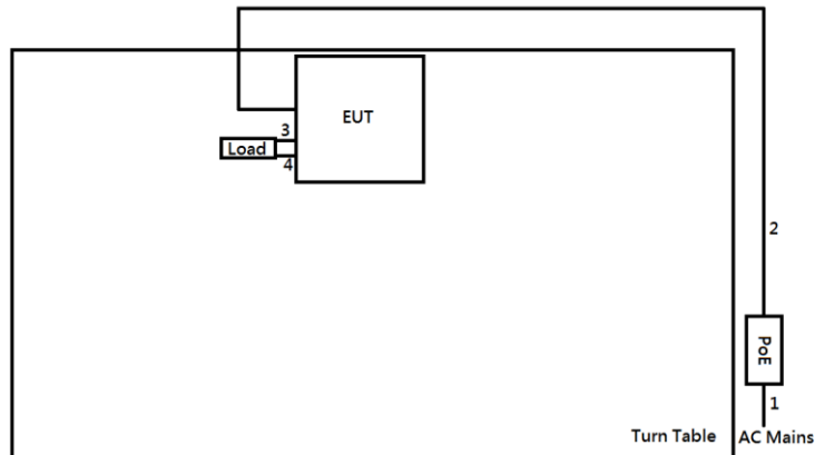
Test Setup Diagram - Radiated Test (Sample 1) - RX
