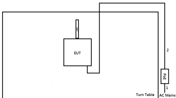
Test Setup Diagram - Radiated Test (Sample 2_Dipole Antenna) - TX
