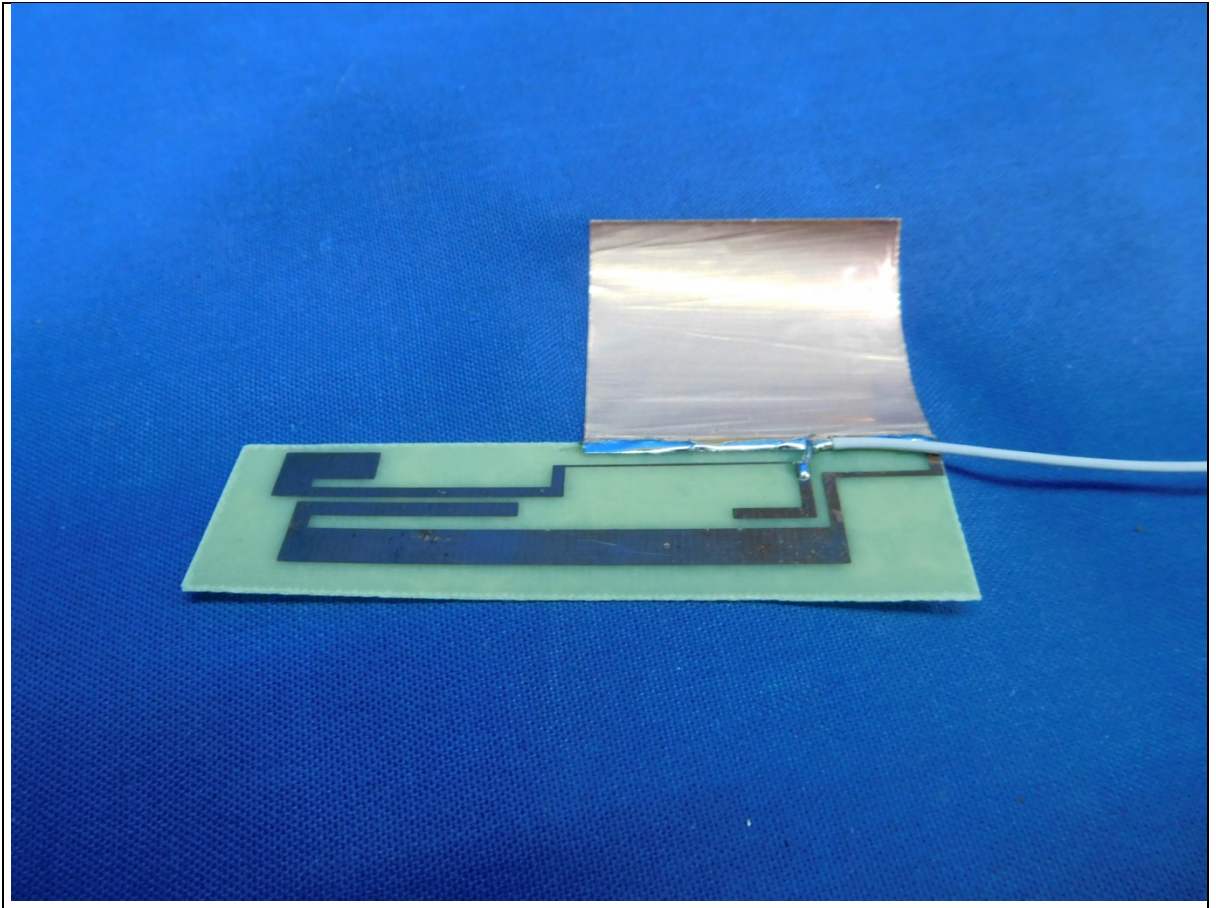
Antenna No. 1
