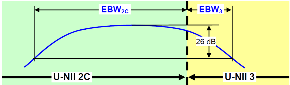
Figure 3. Emission Bandwidth (EBW) within a Band for Band-Crossing Signals
