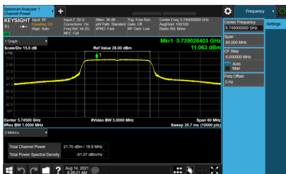
Antenna D
