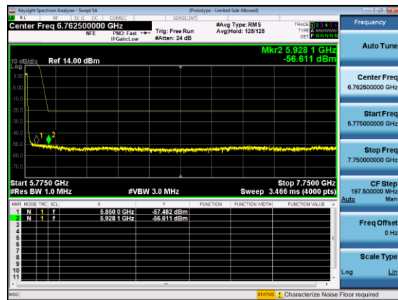
Antenna D
