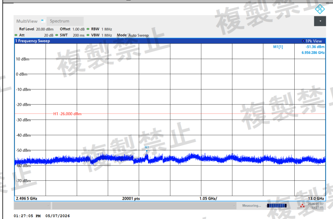
NTNV-BLE_1M-Ant1-2496.5~13000-PASS
