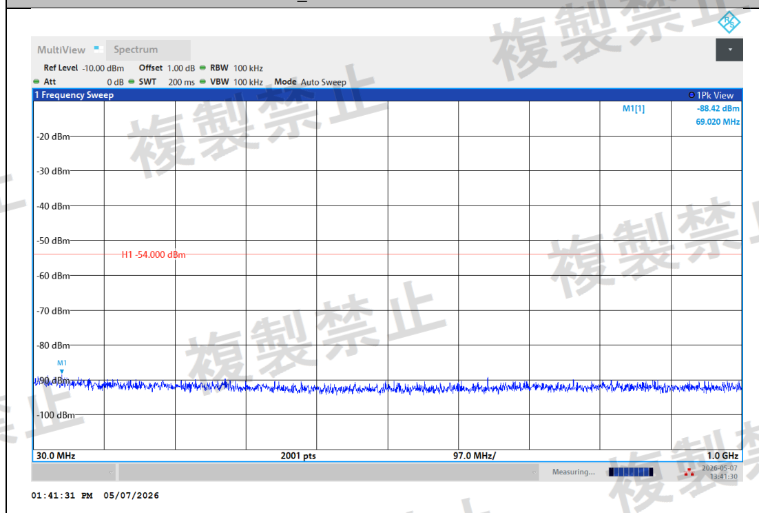
NTNV-BLE_1M-Ant1-2480-30~1000-PASS
