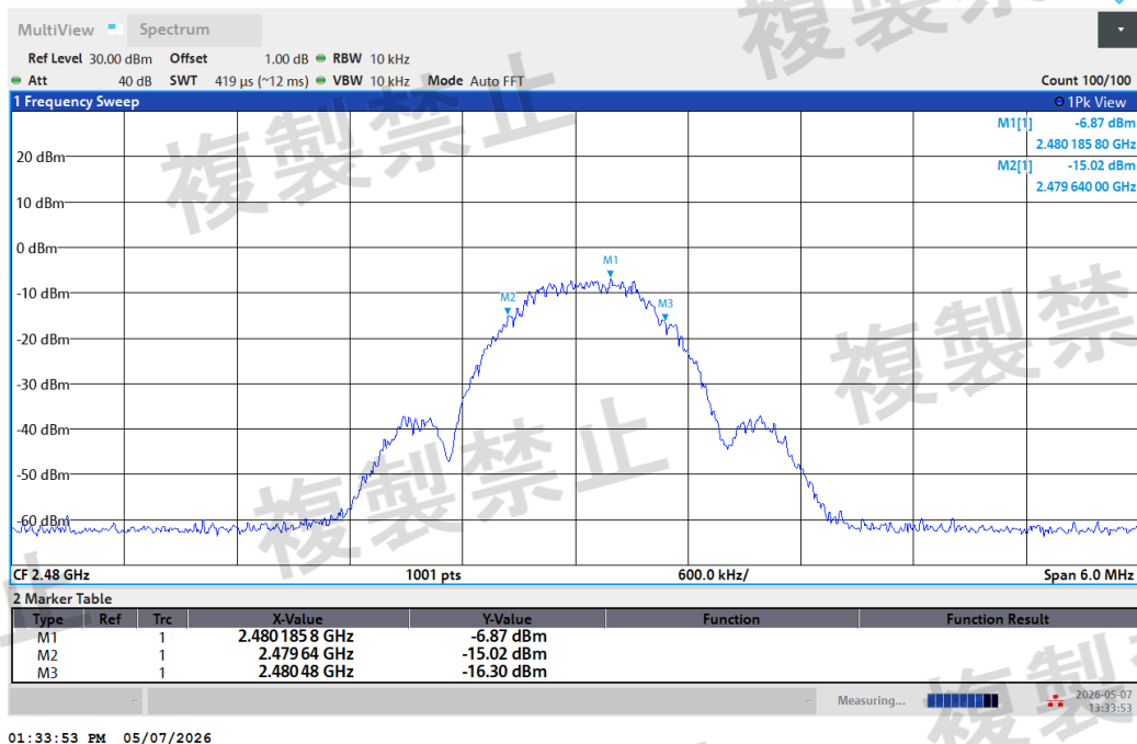
NTNV-BLE_1M-Ant1-2480-PASS
