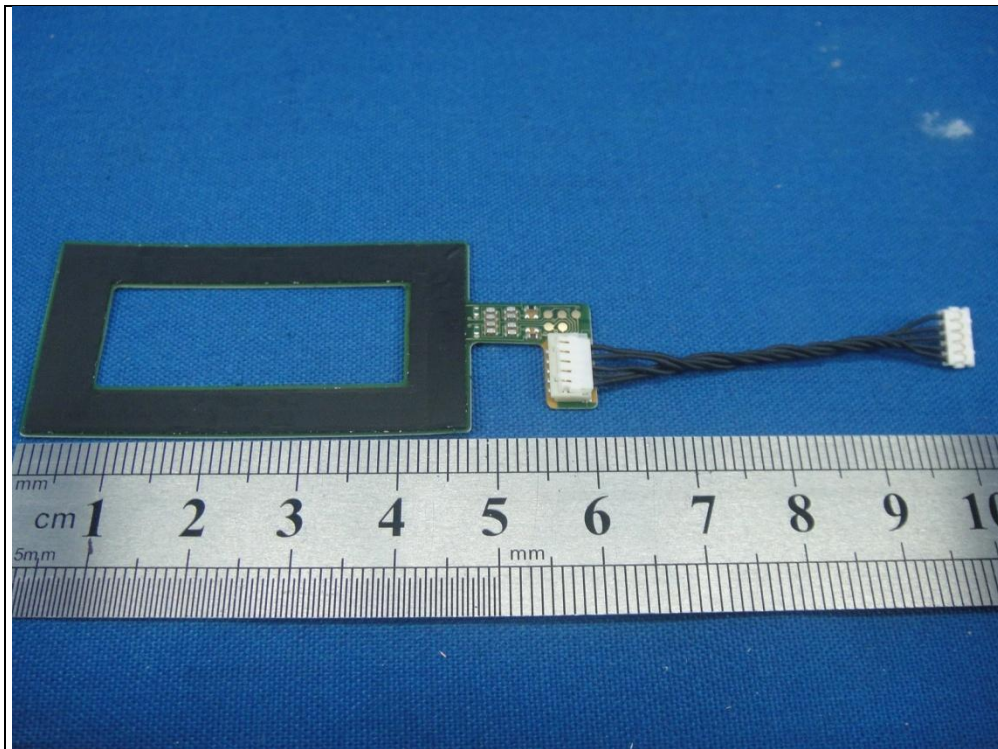
Antenna 7(Brand : Dexerials / Model : ANT-M041B)
