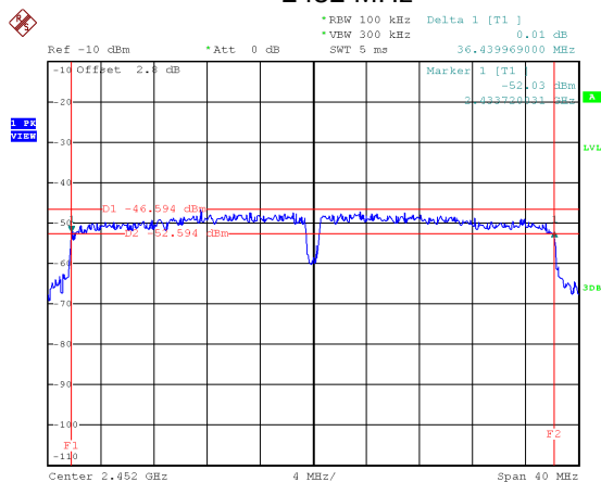
2452 MHz
