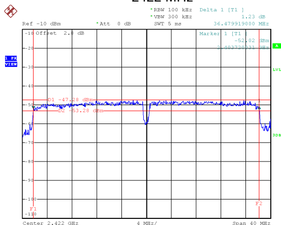
2422 MHz
