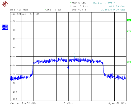
2452 MHz
