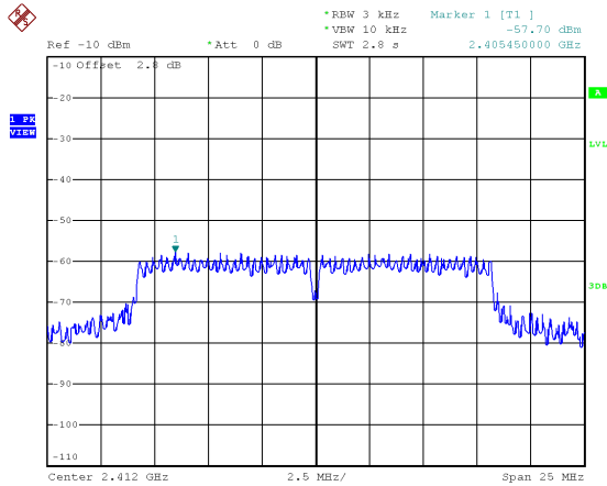
2412 MHz
