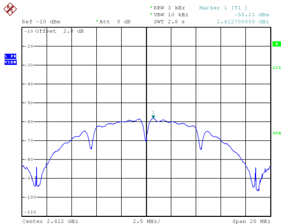
2412 MHz
