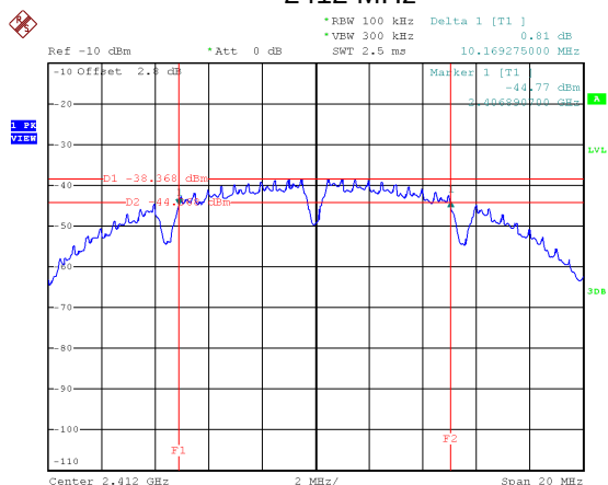
2412 MHz
