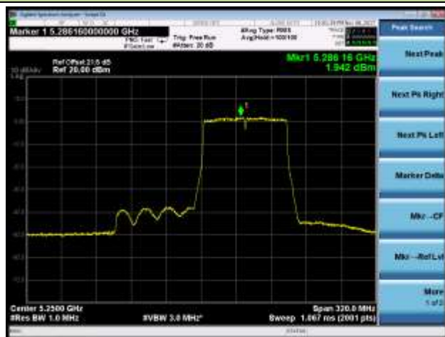
Channel 58 (5290MHz)
