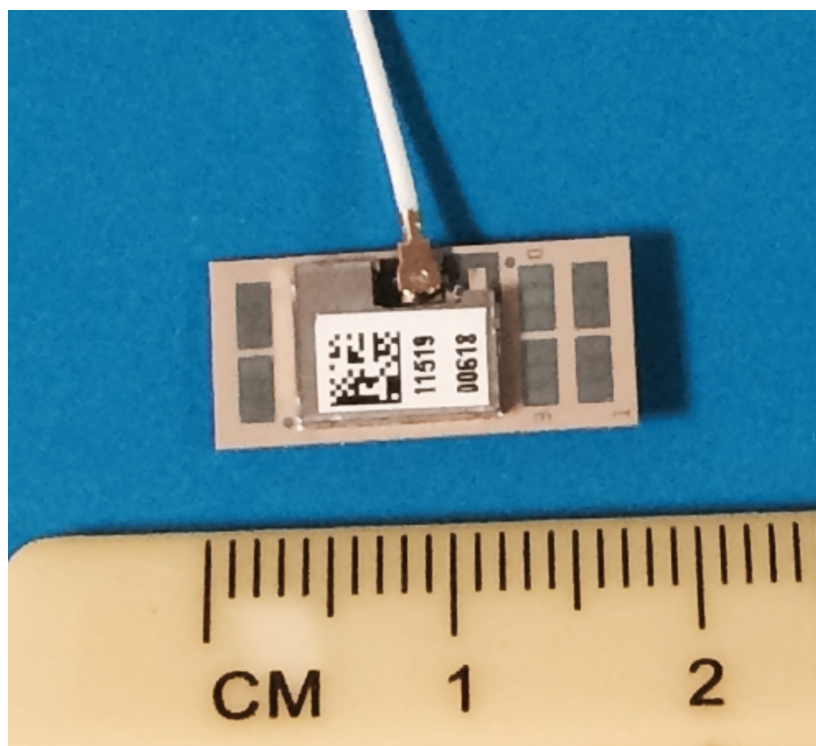
FRONT VIEW (60GHz WiGig RF+ Integral patch antenna array board)
