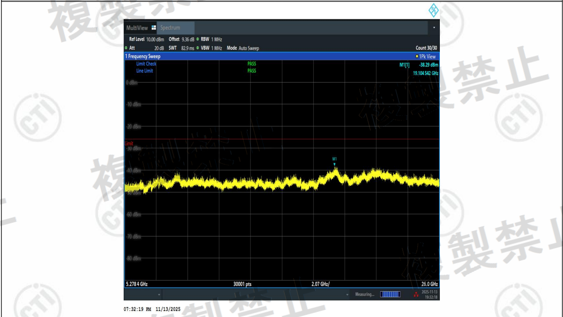
NTNV-11BE40MIMO-Ant1-5230-5278.4~26000-PASS
