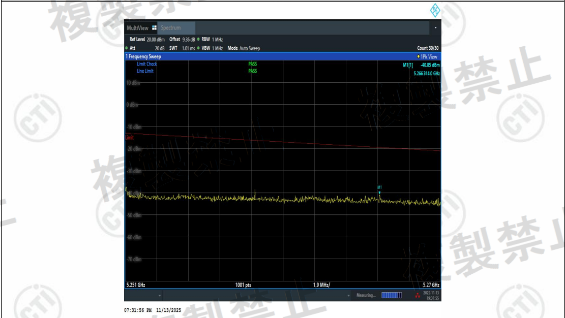
NTNV-11BE40MIMO-Ant1-5230-5251~5270-PASS
