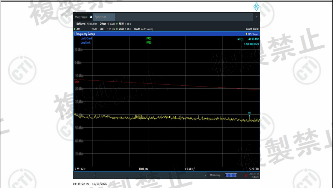
NTNV-11AX40MIMO-Ant1-5230-5251~5270-PASS
