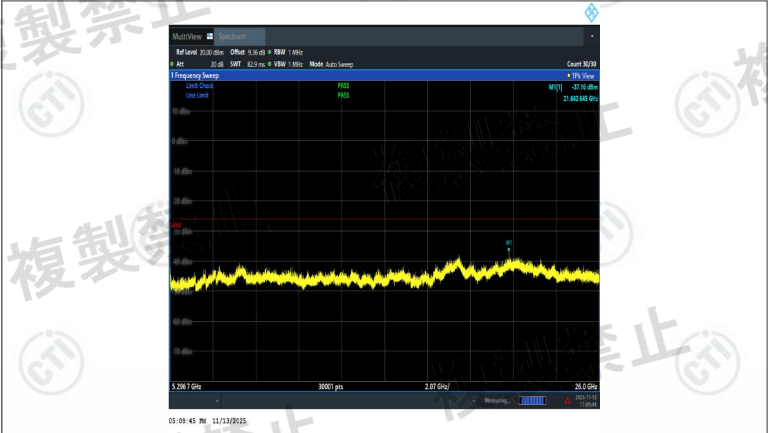
NTNV-11AX80MIMO-Ant1-5210-5296.7~26000-PASS
