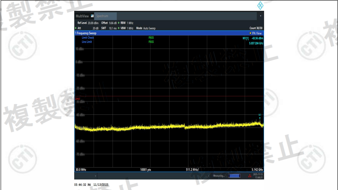
NTNV-11BE20MIMO-Ant3-5200-30~5142-PASS
