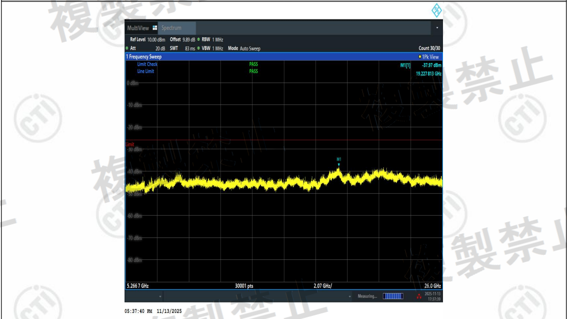
NTVN-11BE20MIMO-Ant1-5200-5266.7~26000-PASS
