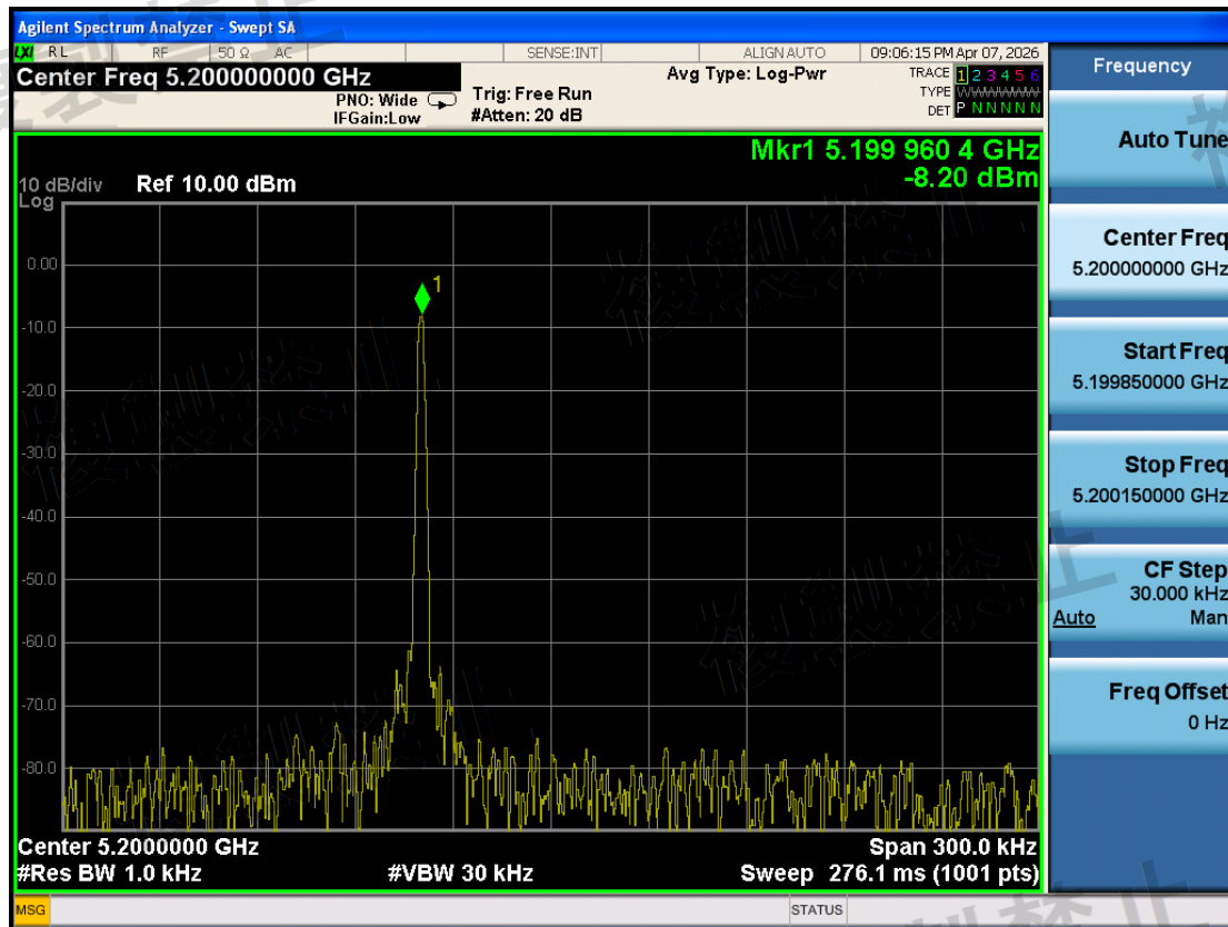
W52\Frequency Error Measurement\802.11a\5200-TX1-N
