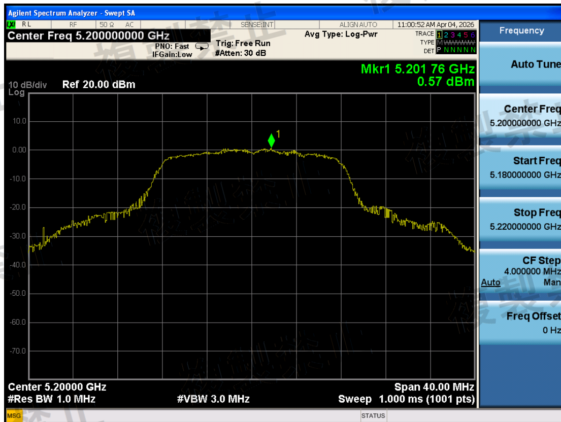
W52\Antenna Power Error\802.11a\1-5200-TX1-N
