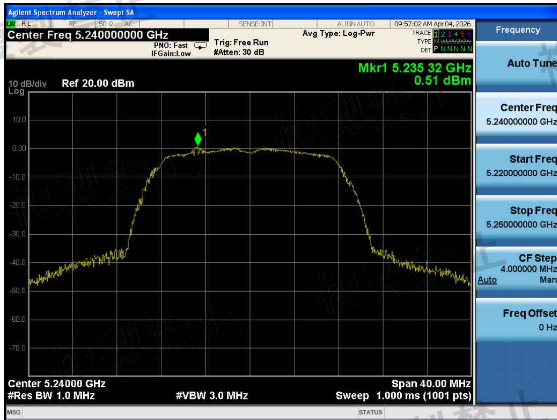
W52\Antenna Power Error\802.11a\1-5240-TX0-N
