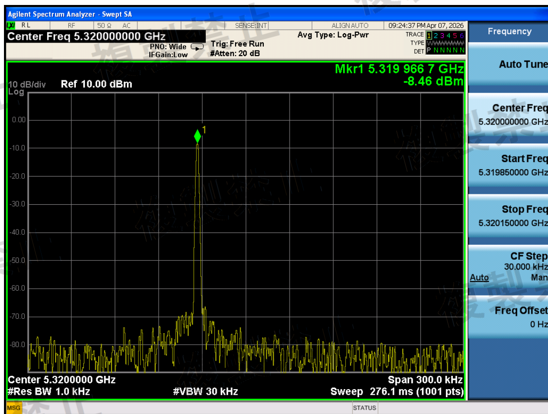
W53\Frequency Error Measurement\802.11ax HE20\5320-TX0-N
