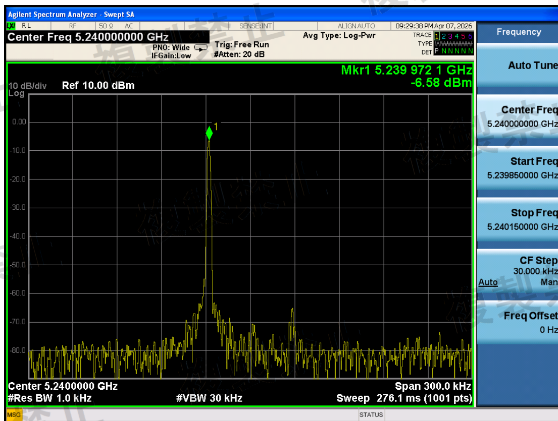
W52\Frequency Error Measurement\802.11ax HE20\5240-TX0-N
