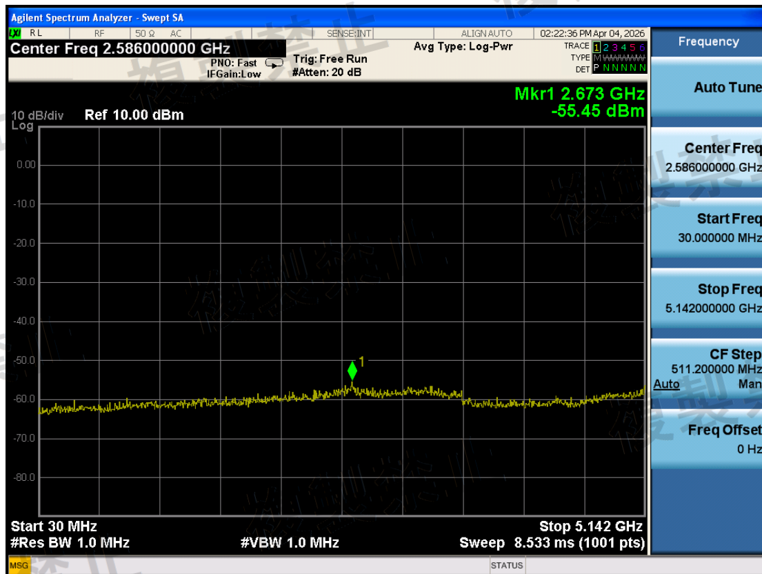
W52\Unwanted Emission Strength\802.11a\TX0\30.00~5142.00-5180-TX0-N
