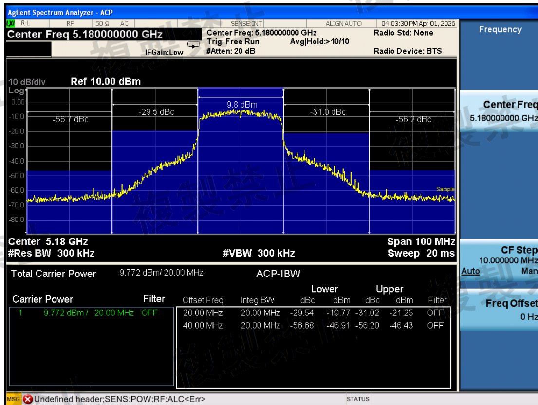
W52\Adjacent Channel Leakage Power\802.11ax HE20\5180-TX1-N
