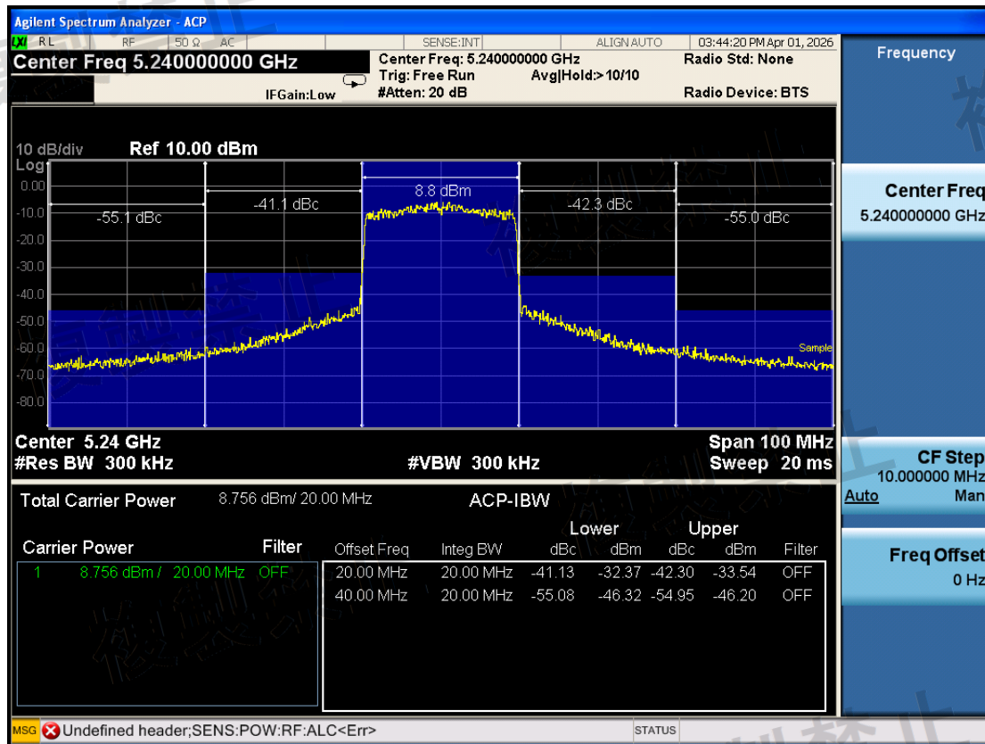
W52\Adjacent Channel Leakage Power\802.11ax HE20\5240-TX0-N
