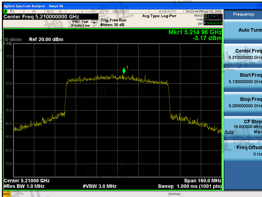
W52\Antenna Power Error\802.11ax HE80\1-5210-TX1-N
