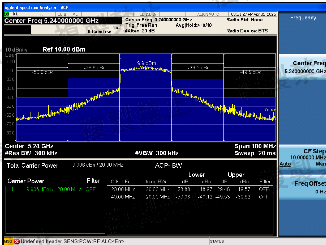
W52\Adjacent Channel Leakage Power\802.11ax HE20\5240-TX1-N
