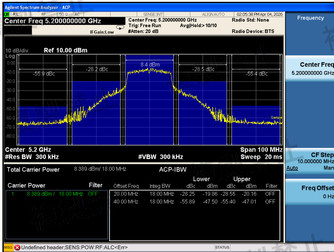
W52\Adjacent Channel Leakage Power\802.11a\5200-TX1-N
