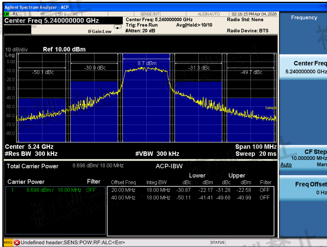
W52\Adjacent Channel Leakage Power\802.11a\5240-TX0-N
