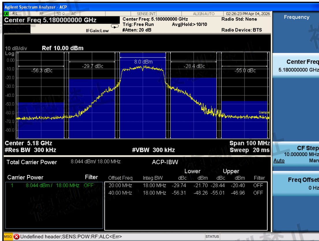
W52\Adjacent Channel Leakage Power\802.11a\5180-TX0-N
