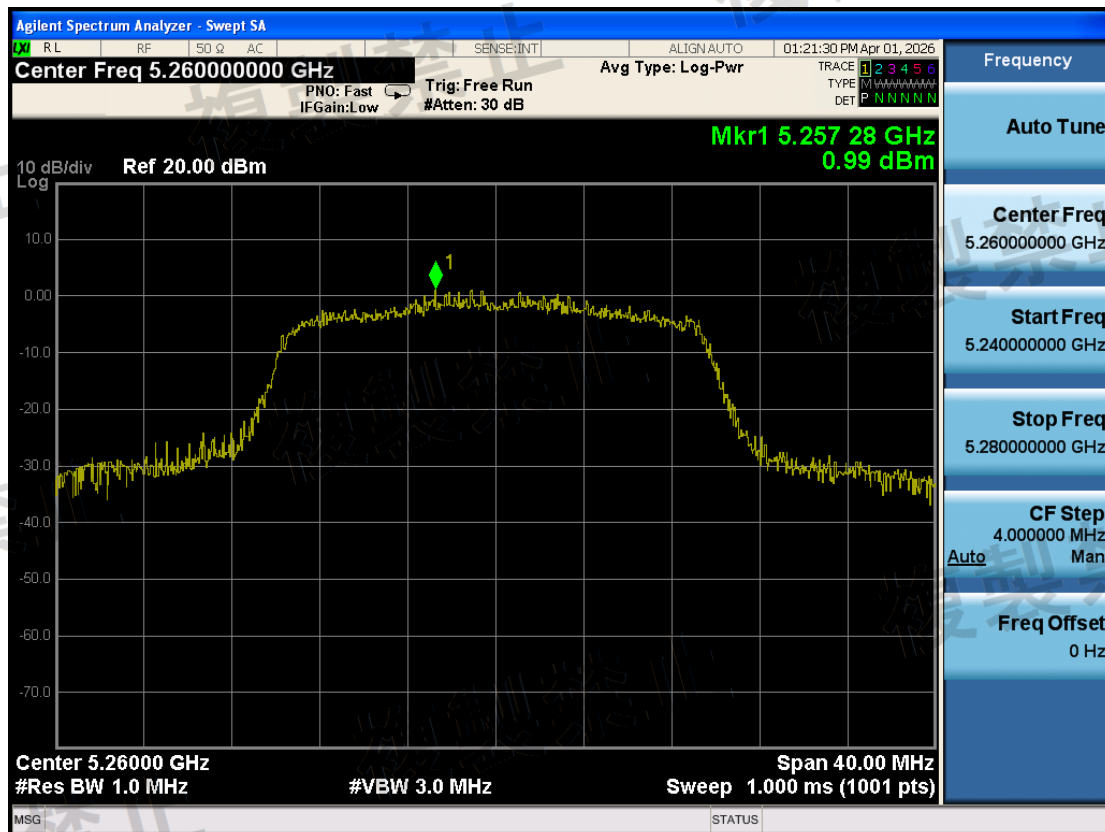
W53\Antenna Power Error\802.11ax HE20\1-5260-TX1-N
