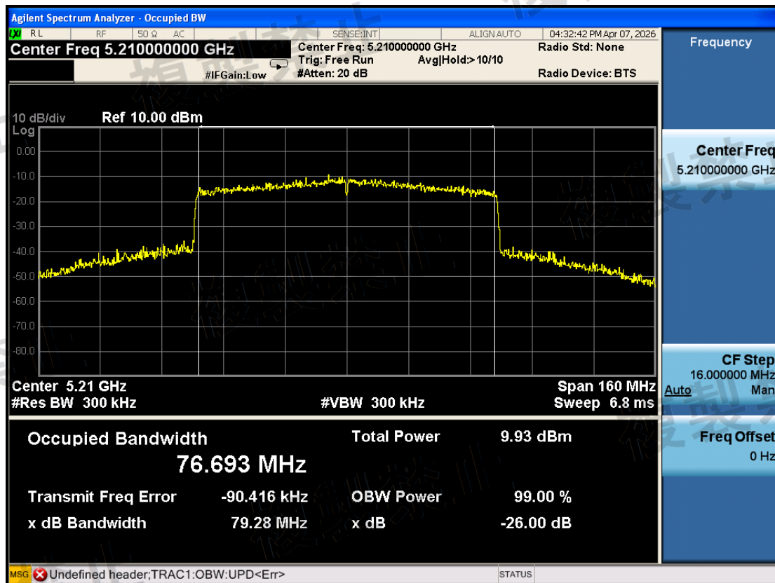
W52\Occupied Bandwidth\802.11ax HE80\5210-TX0-N
