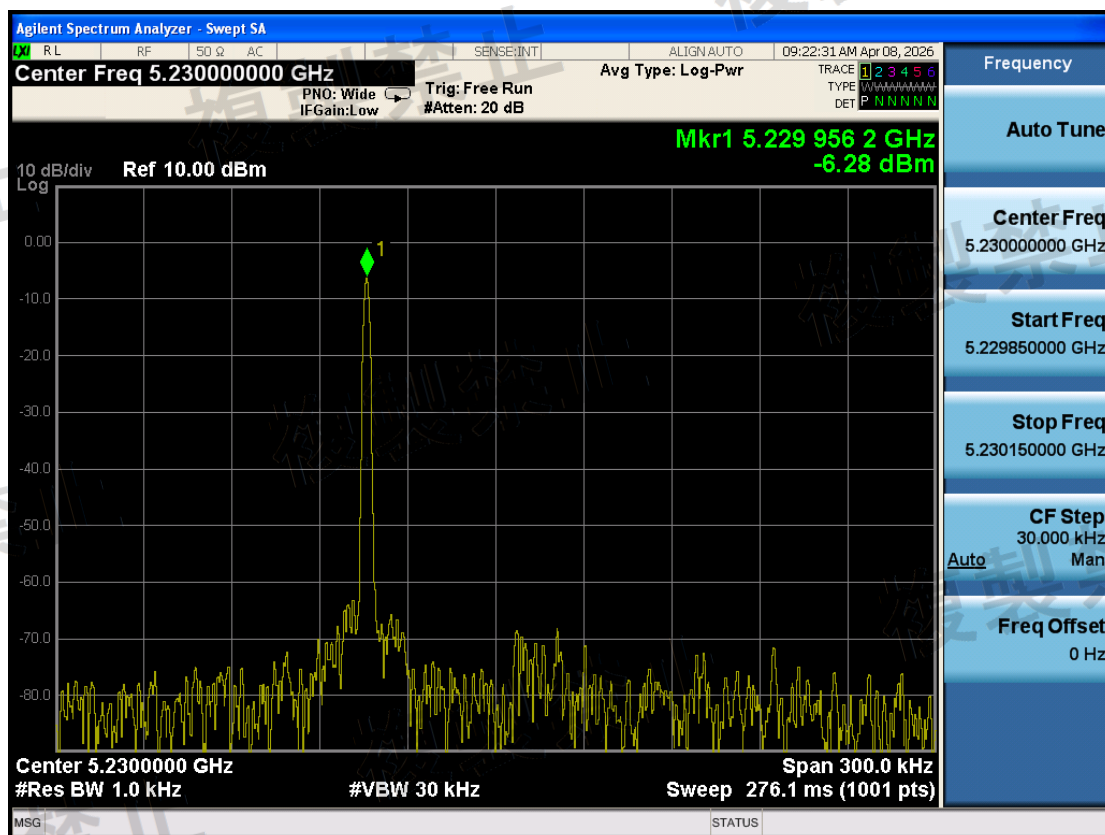
W52\Frequency Error Measurement\802.11ax HE40\5230-TX1-N
