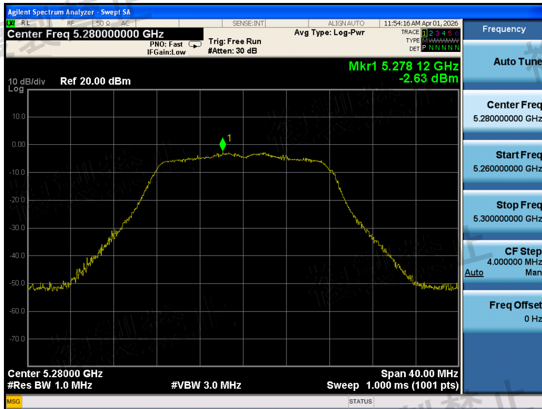
W53\Antenna Power Error\802.11a\1-5280-TX1-N
