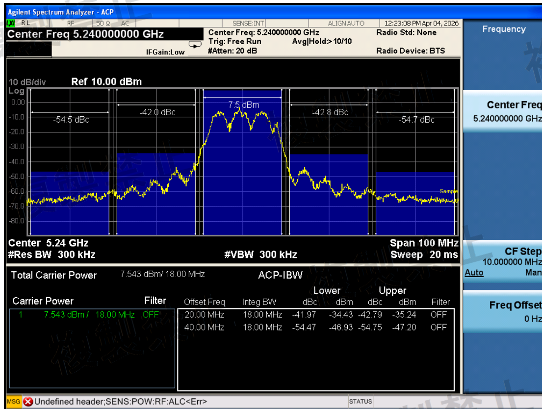
W52\Adjacent Channel Leakage Power\802.11a\5240-X-N
