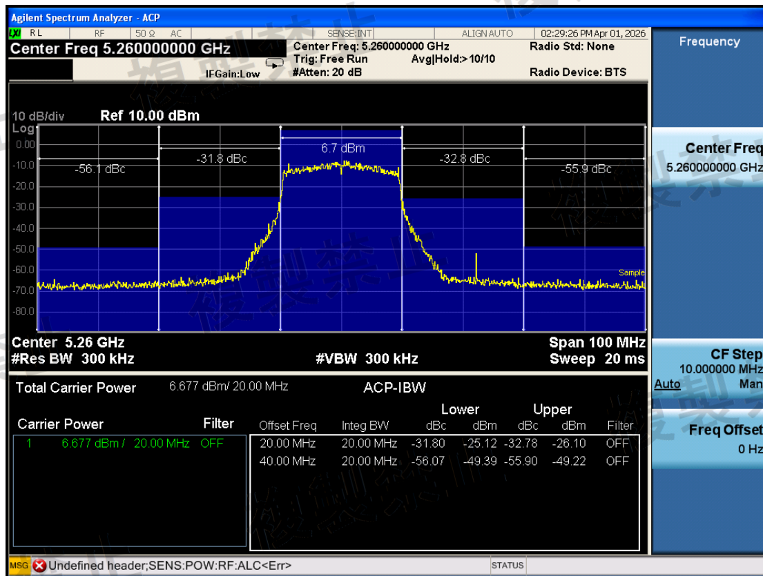
W53\Adjacent Channel Leakage Power\802.11ax HE20\5260-TX1-N
