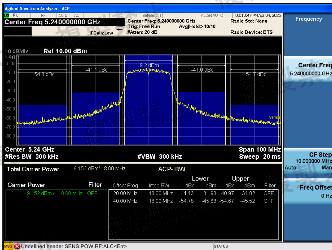
W52\Adjacent Channel Leakage Power\802.11a\5240-TX1-N
