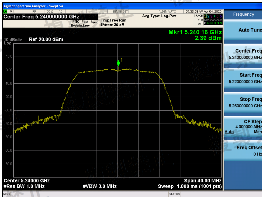
W52\Antenna Power Error\802.11a\1-5240-TX1-N
