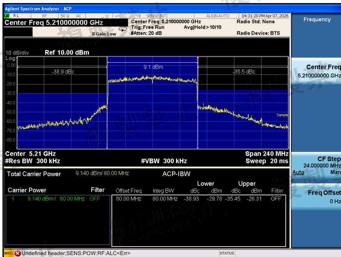
W52\Adjacent Channel Leakage Power\802.11ax HE80\5210-TX1-N
