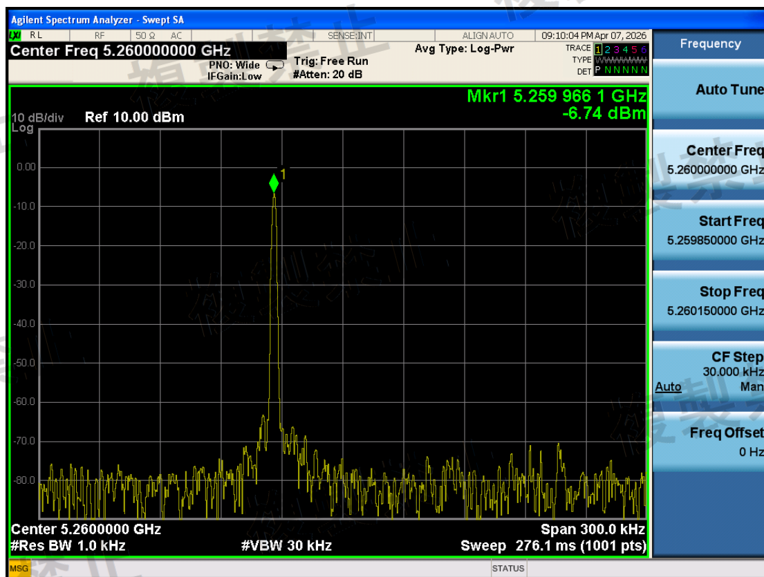
W53\Frequency Error Measurement\802.11a\5260-TX1-N
