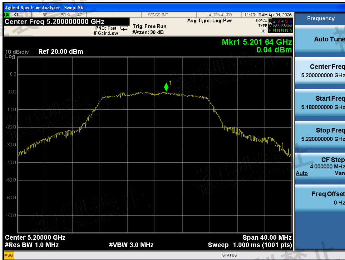
W52\Antenna Power Error\802.11a\1-5200-TX0-N
