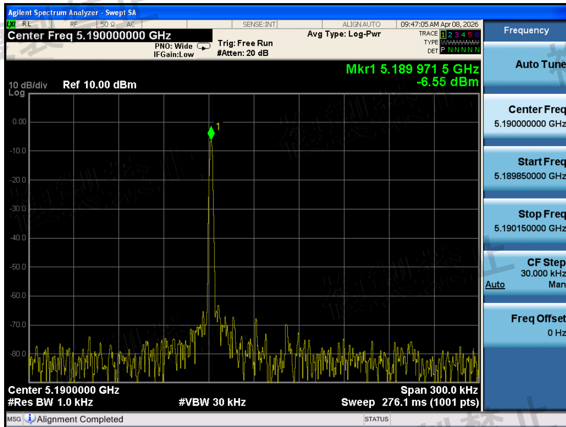
W52\Frequency Error Measurement\802.11ax HE40\5190-TX0-N
