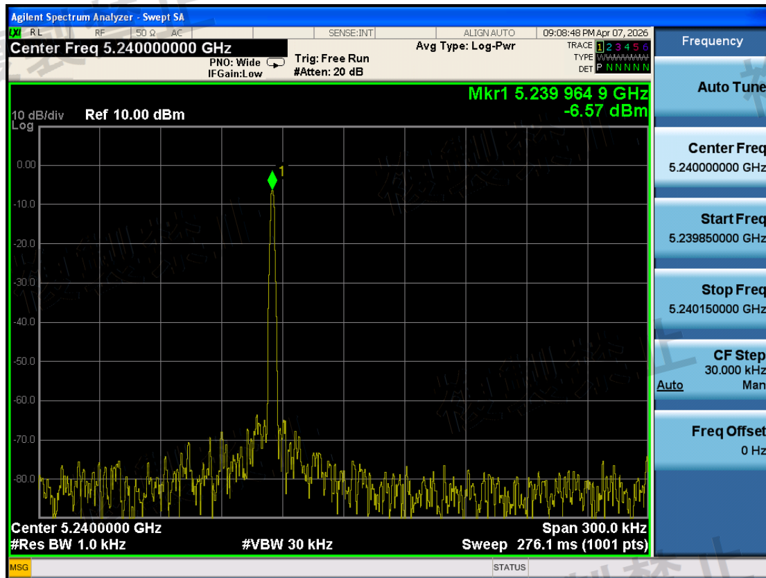
W52\Frequency Error Measurement\802.11a\5240-TX1-N
