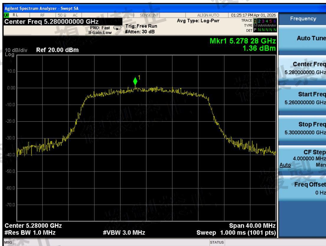
W53\Antenna Power Error\802.11ax HE20\1-5280-TX1-N
