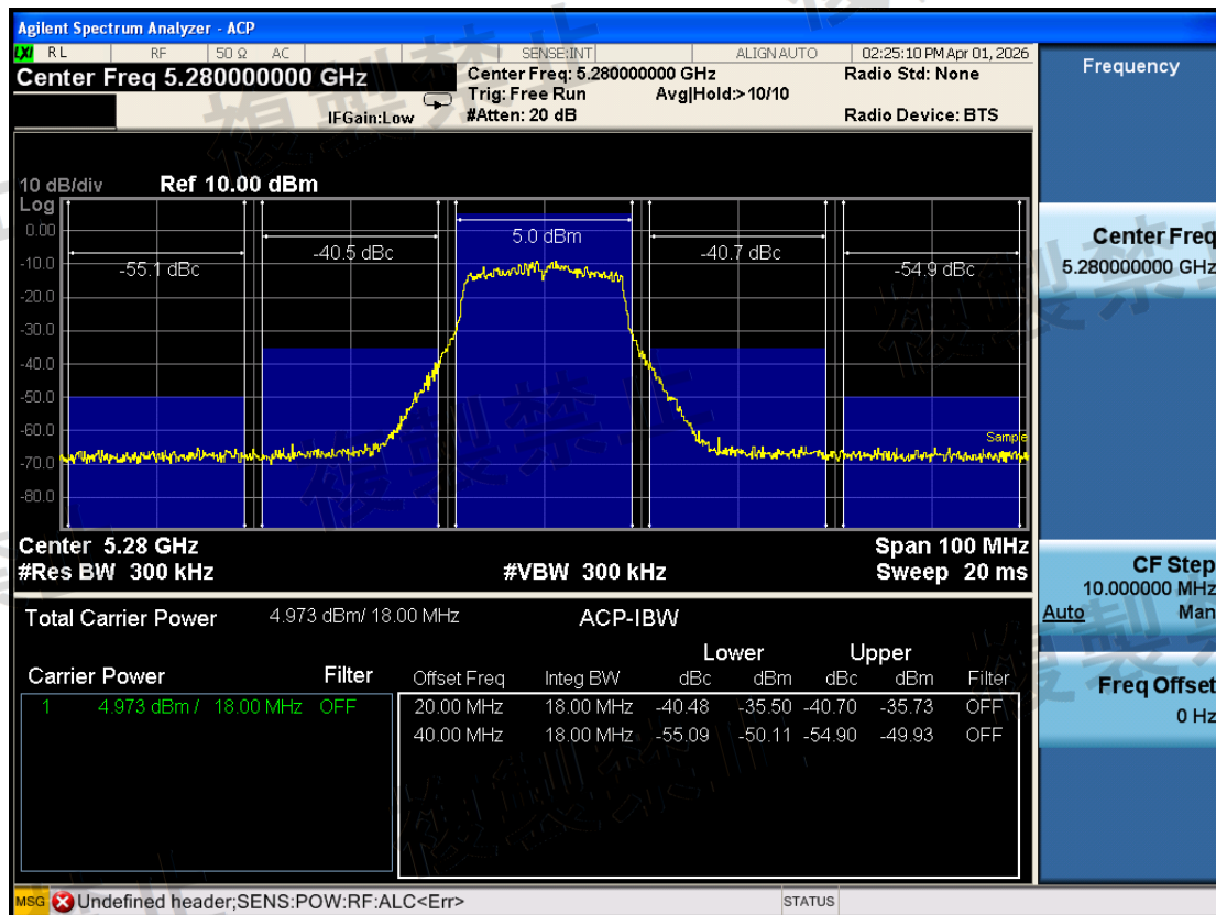
W53\Adjacent Channel Leakage Power\802.11a\5280-TX1-N
