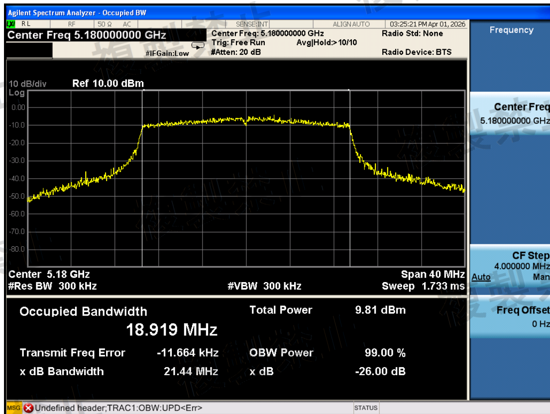
W52\Occupied Bandwidth\802.11ax HE20\5180-TX0-N
