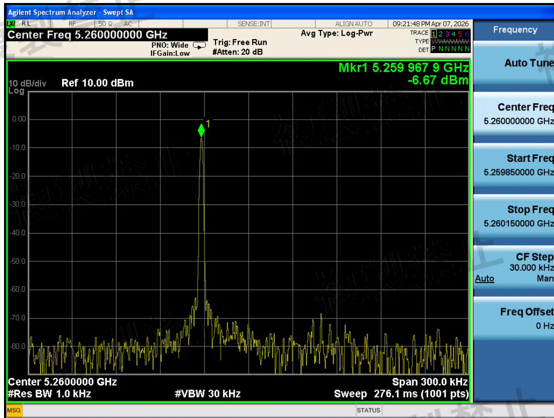
W53\Frequency Error Measurement\802.11a\5260-TX0-N
