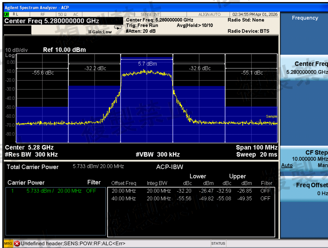
W53\Adjacent Channel Leakage Power\802.11ax HE20\5280-TX0-N
