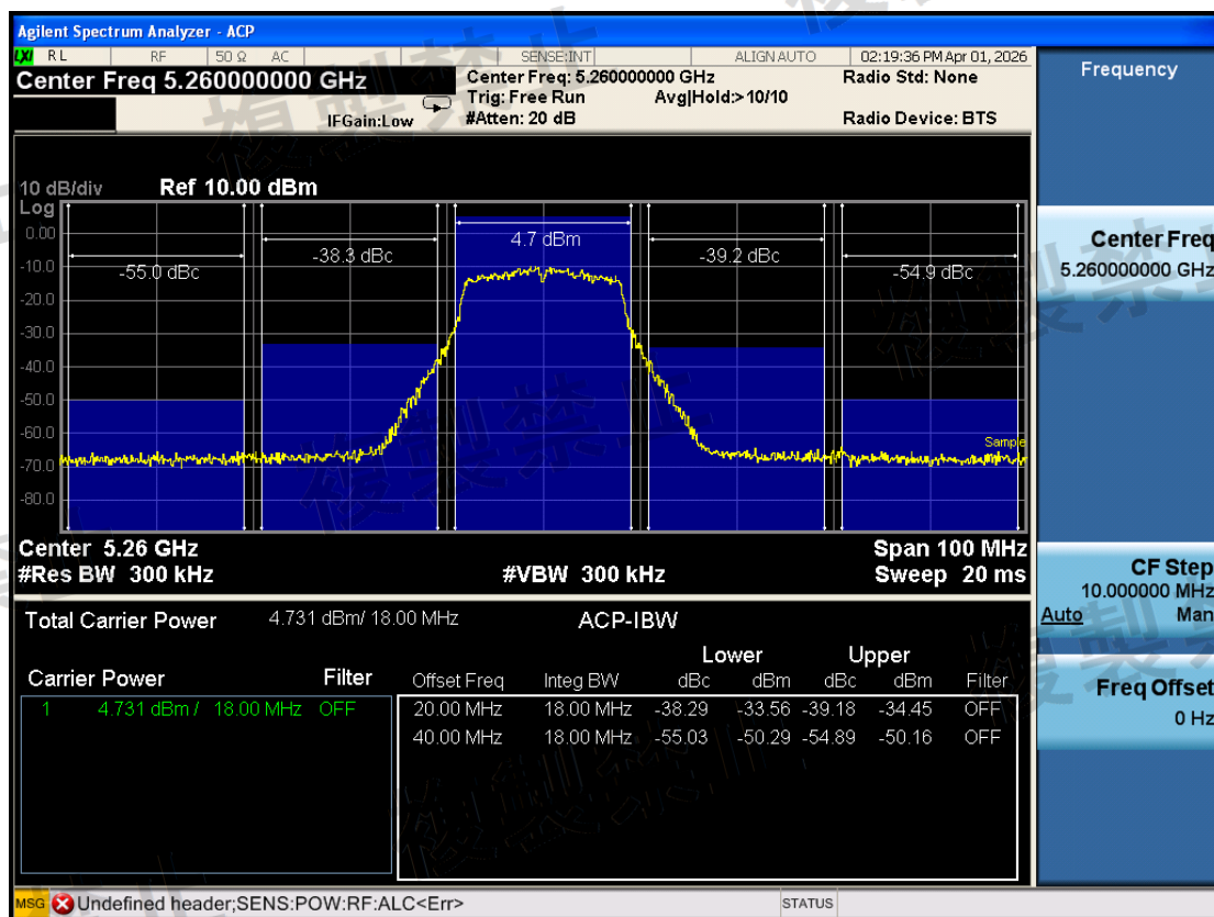
W53\Adjacent Channel Leakage Power\802.11a\5260-TX0-N
