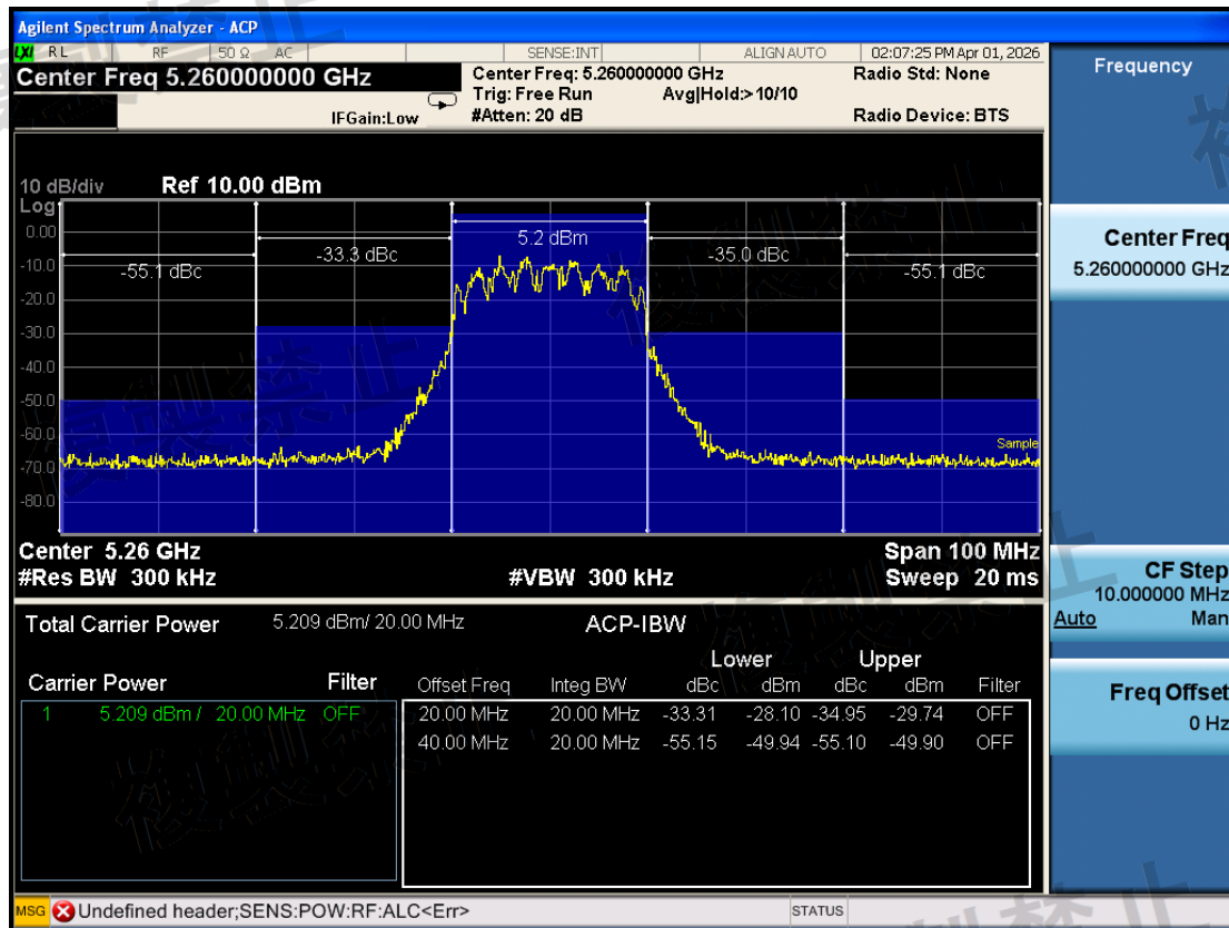
W53\Adjacent Channel Leakage Power\802.11ax HE20\5260-X-N
