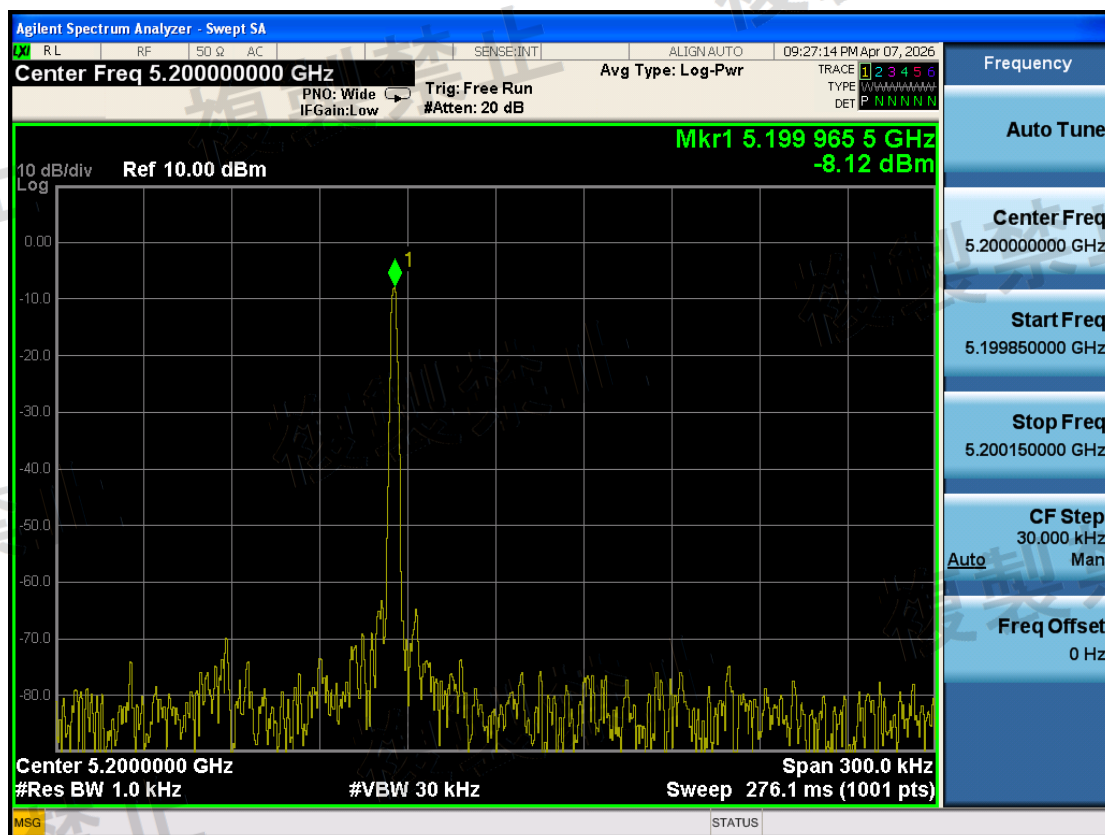
W52\Frequency Error Measurement\802.11a\5200-TX0-N
