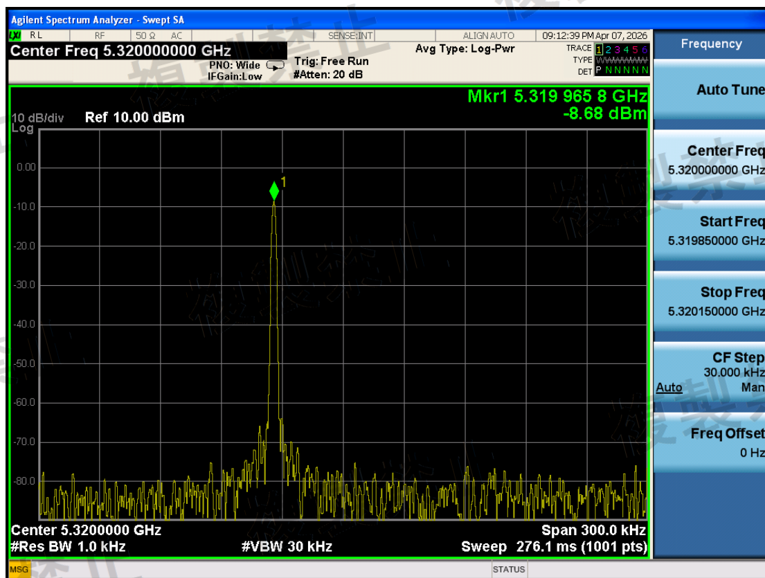
W53\Frequency Error Measurement\802.11a\5320-TX1-N
