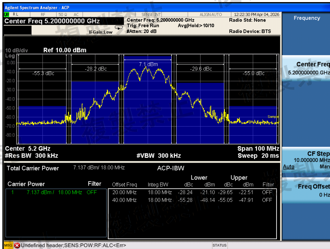
W52\Adjacent Channel Leakage Power\802.11a\5200-X-N
