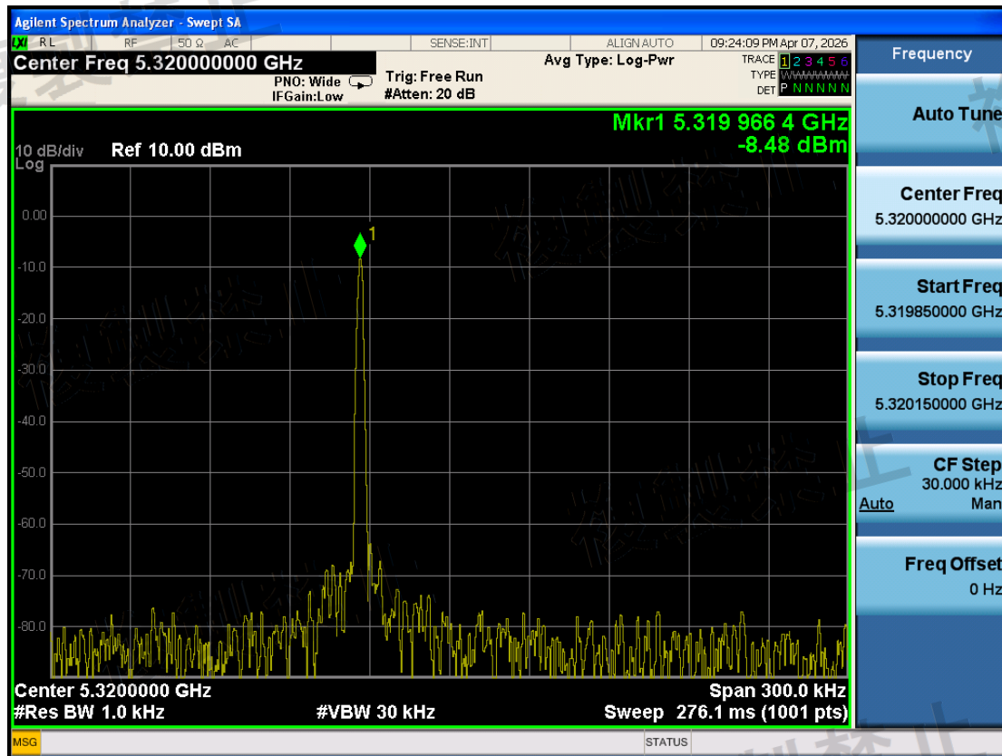
W53\Frequency Error Measurement\802.11a\5320-TX0-N
