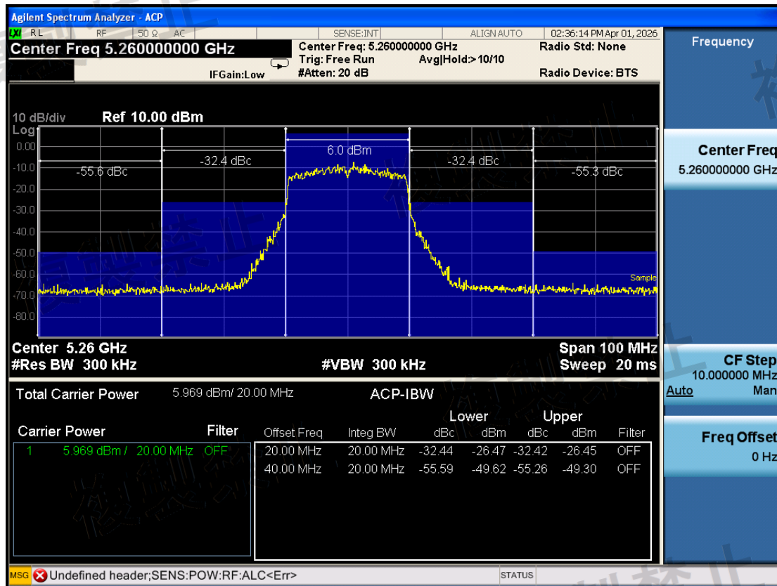
W53\Adjacent Channel Leakage Power\802.11ax HE20\5260-TX0-N
