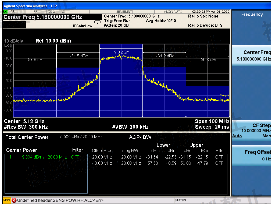
W52\Adjacent Channel Leakage Power\802.11ax HE20\5180-TX0-N
