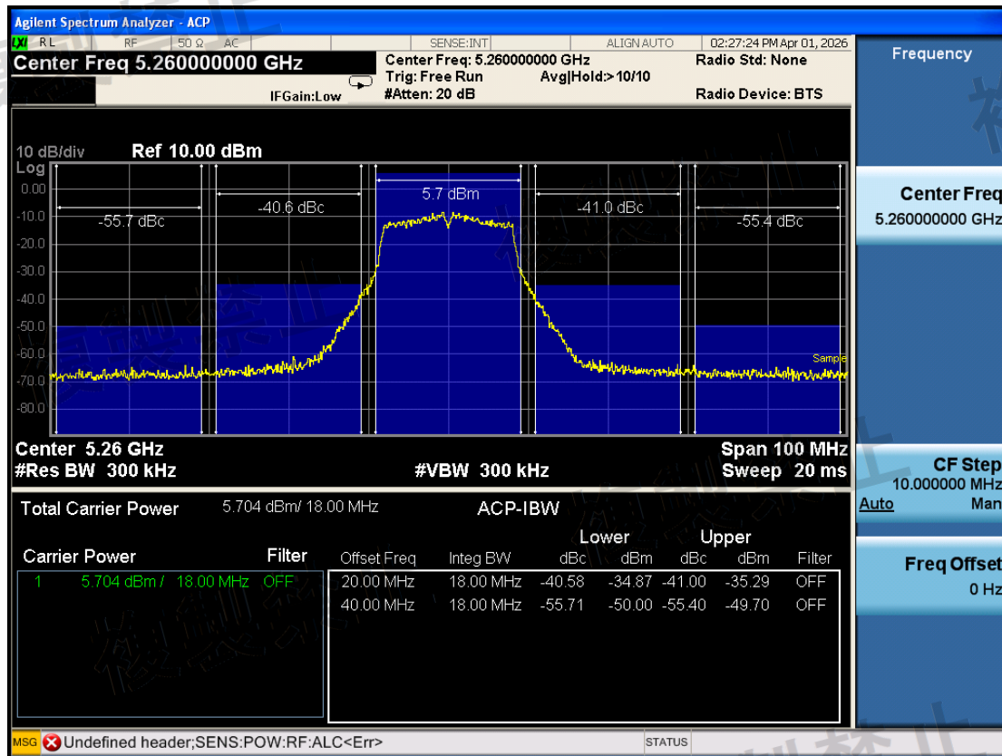
W53\Adjacent Channel Leakage Power\802.11a\5260-TX1-N
