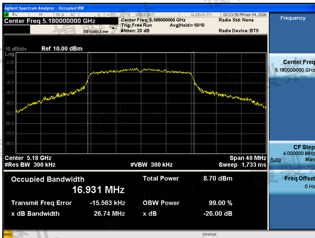
W52\Occupied Bandwidth\802.11a\5180-TX0-N
