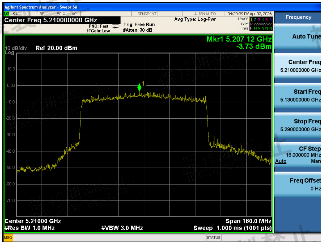
W52\Antenna Power Error\802.11ax HE80\1-5210-TX0-N
