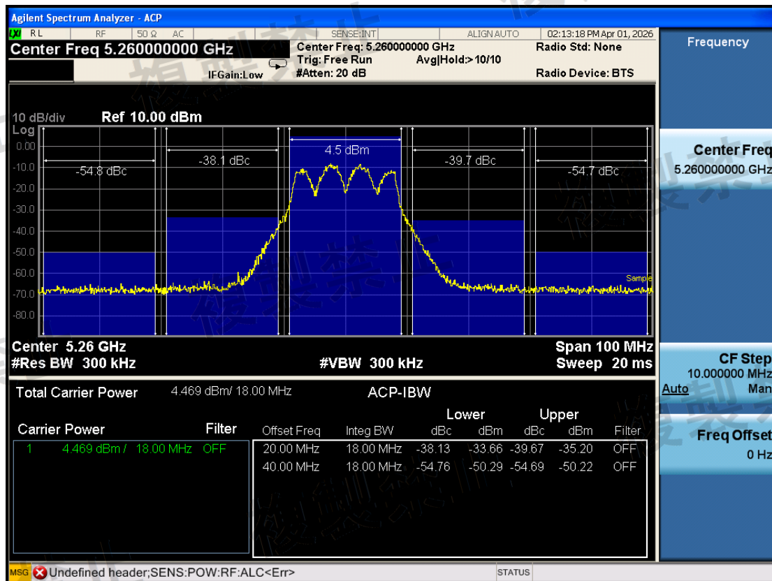
W53\Adjacent Channel Leakage Power\802.11a\5260-X-N
