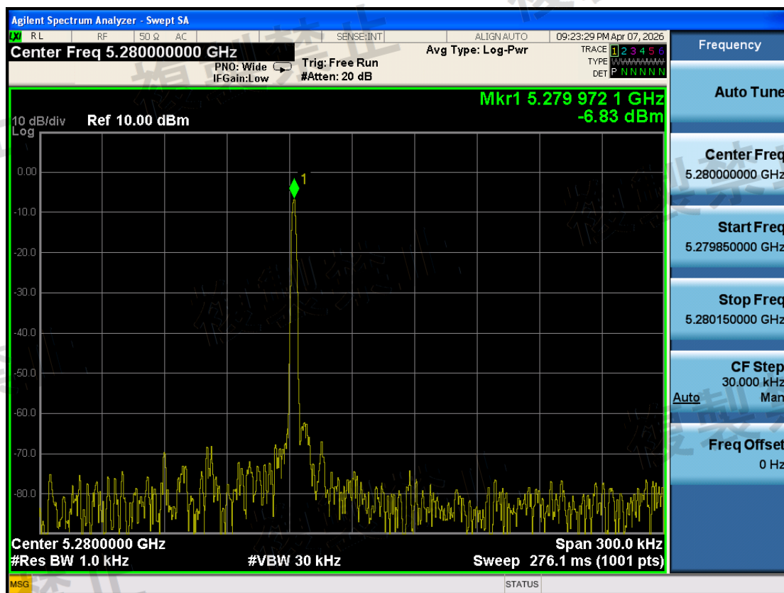
W53\Frequency Error Measurement\802.11ax HE20\5280-TX0-N
