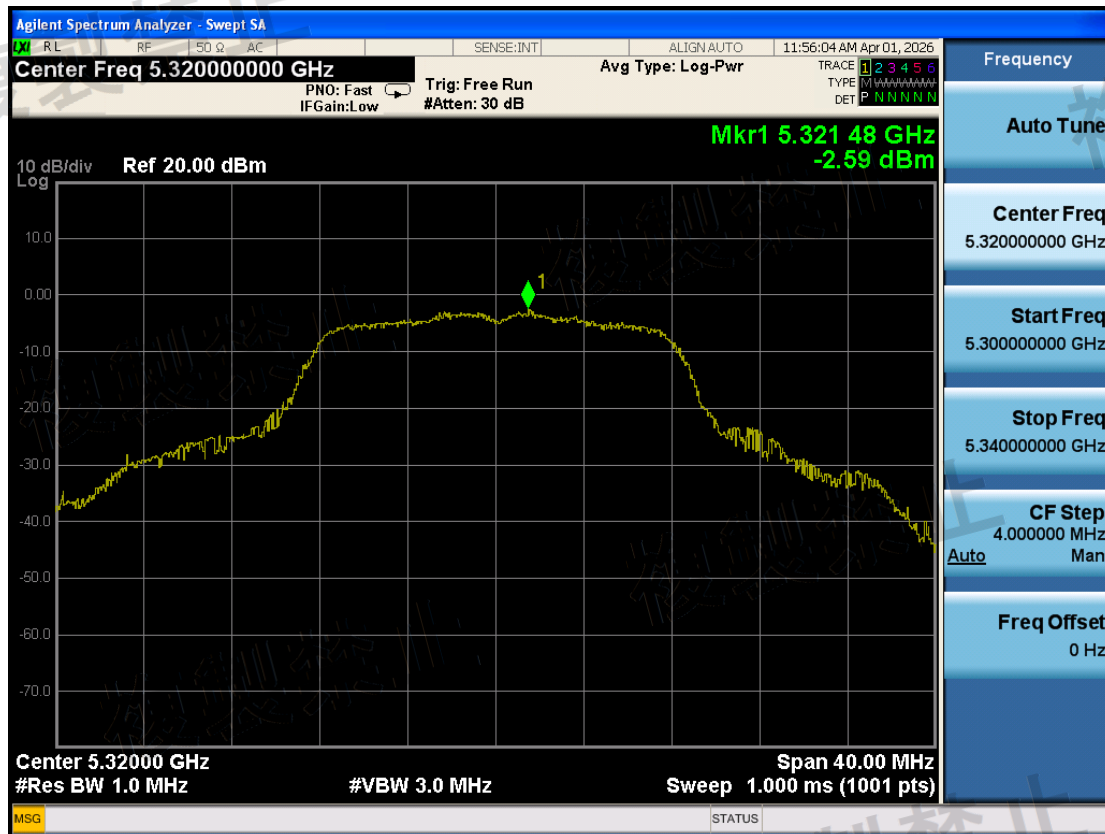
W53\Antenna Power Error\802.11a\1-5320-TX1-N
