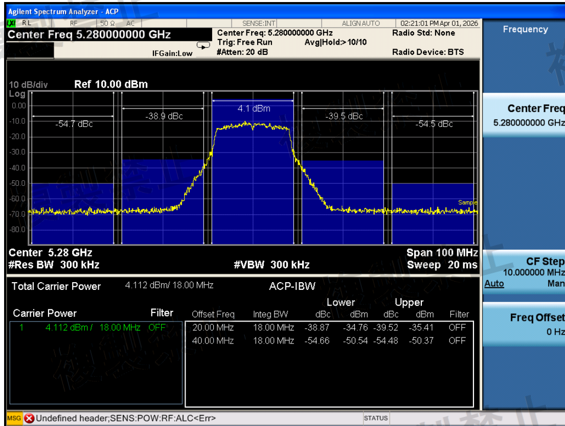
W53\Adjacent Channel Leakage Power\802.11a\5280-TX0-N
