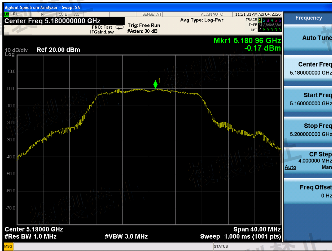
W52\Antenna Power Error\802.11a\1-5180-TX0-N
