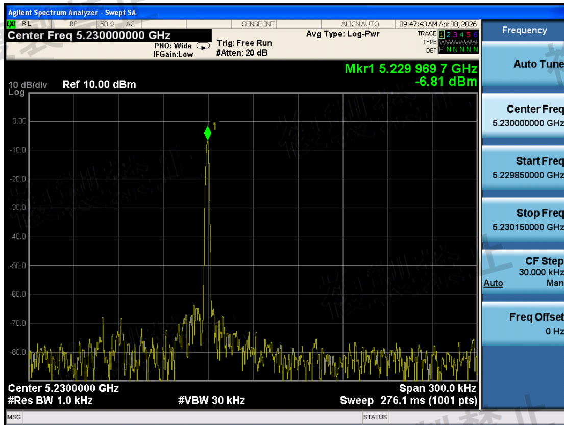
W52\Frequency Error Measurement\802.11ax HE40\5230-TX0-N
