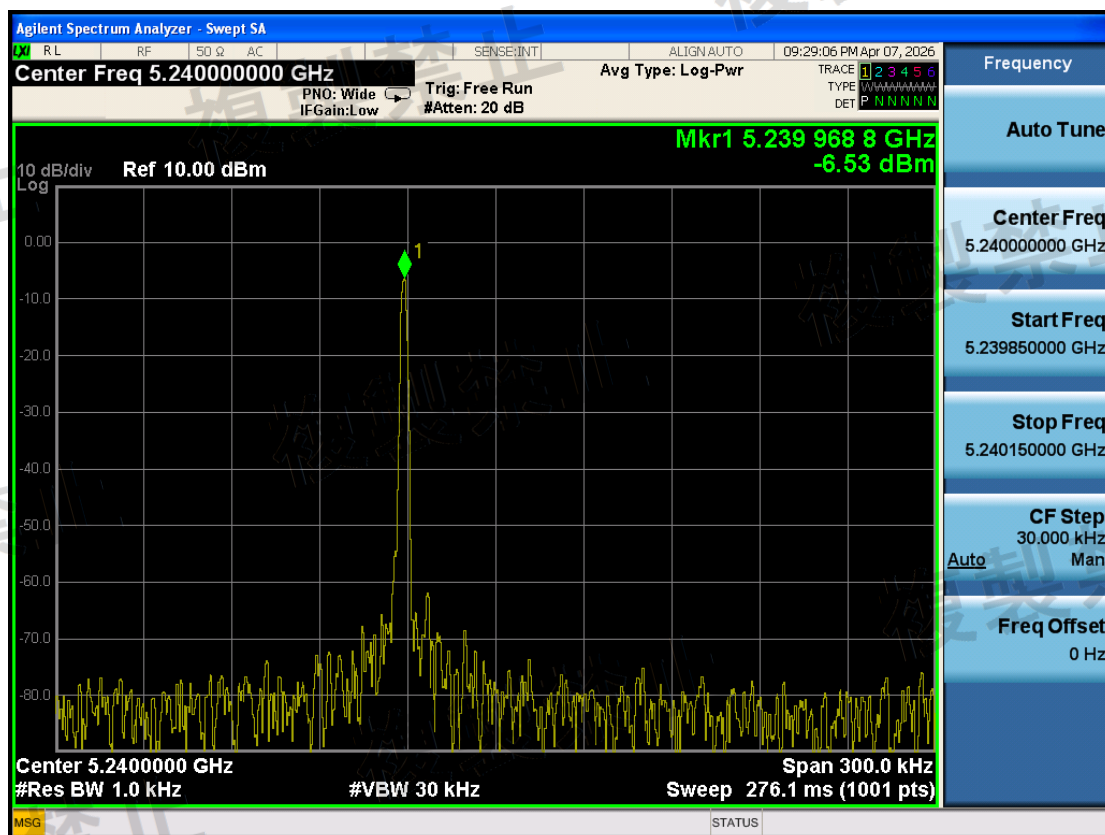
W52\Frequency Error Measurement\802.11a\5240-TX0-N
