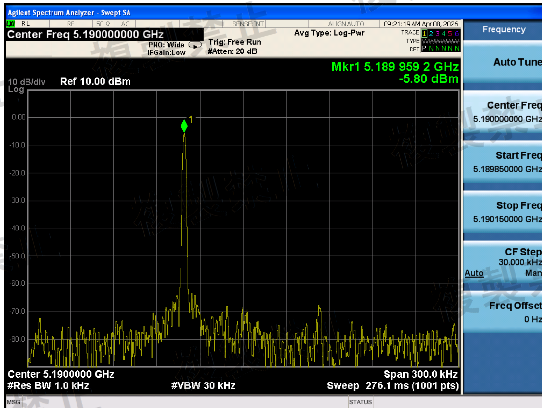
W52\Frequency Error Measurement\802.11ax HE40\5190-TX1-N
