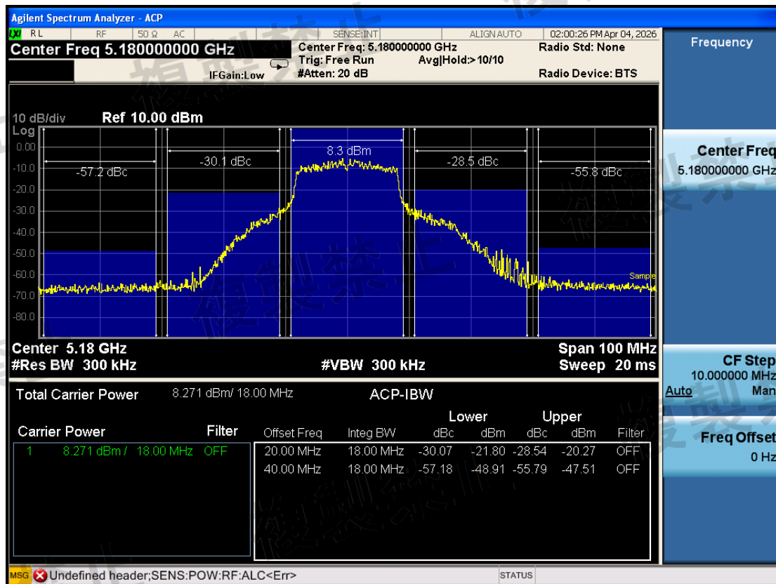
W52\Adjacent Channel Leakage Power\802.11a\5180-TX1-N
