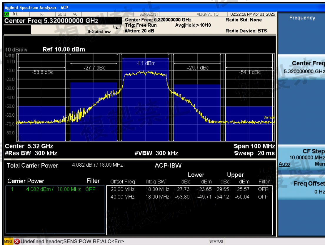
W53\Adjacent Channel Leakage Power\802.11a\5320-TX0-N
