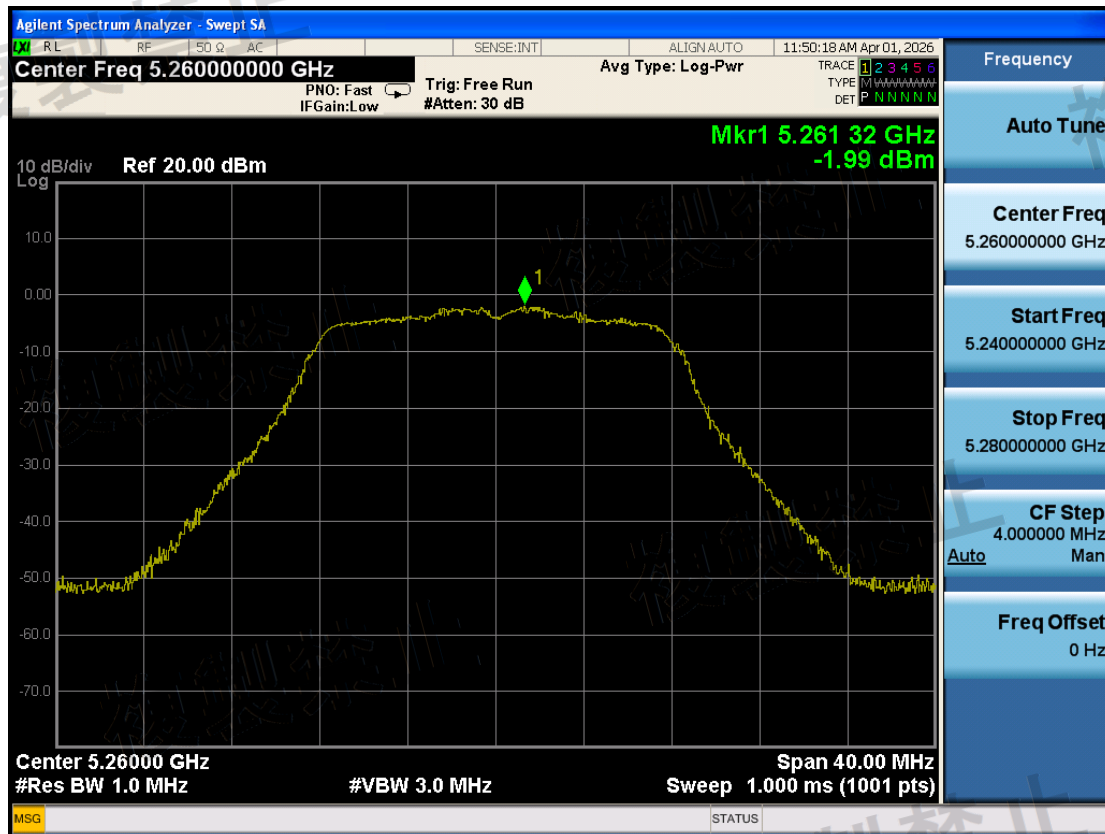
W53\Antenna Power Error\802.11a\1-5260-TX1-N
