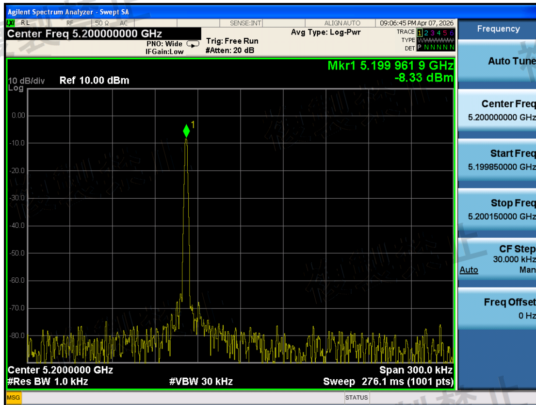
W52\Frequency Error Measurement\802.11ax HE20\5200-TX1-N
