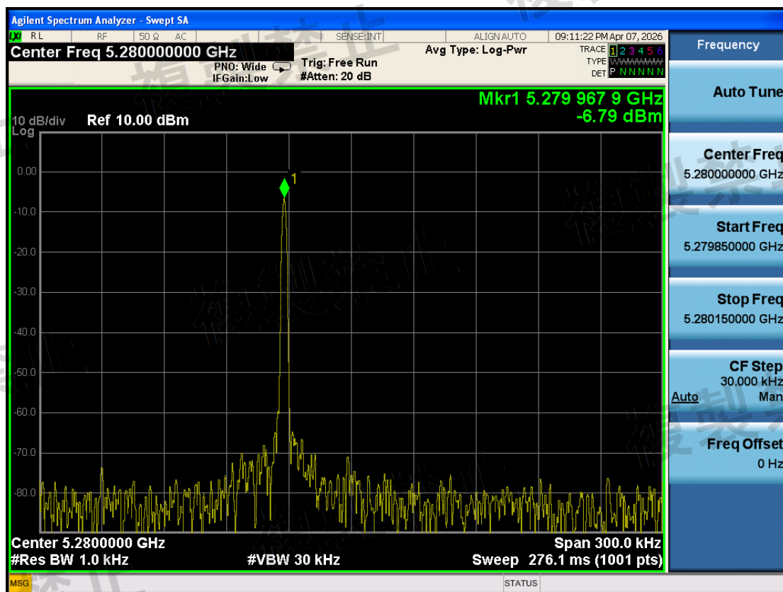
W53\Frequency Error Measurement\802.11a\5280-TX1-N
