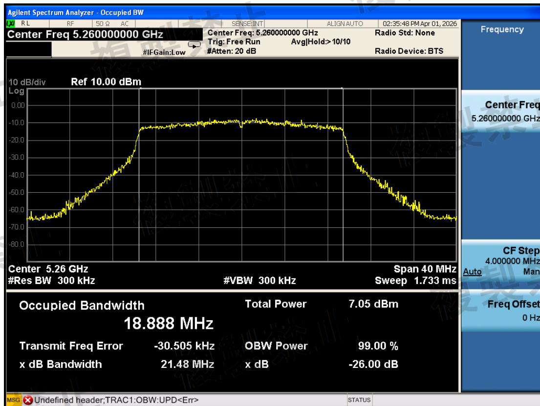
W53\Occupied Bandwidth\802.11ax HE20\5260-TX0-N
