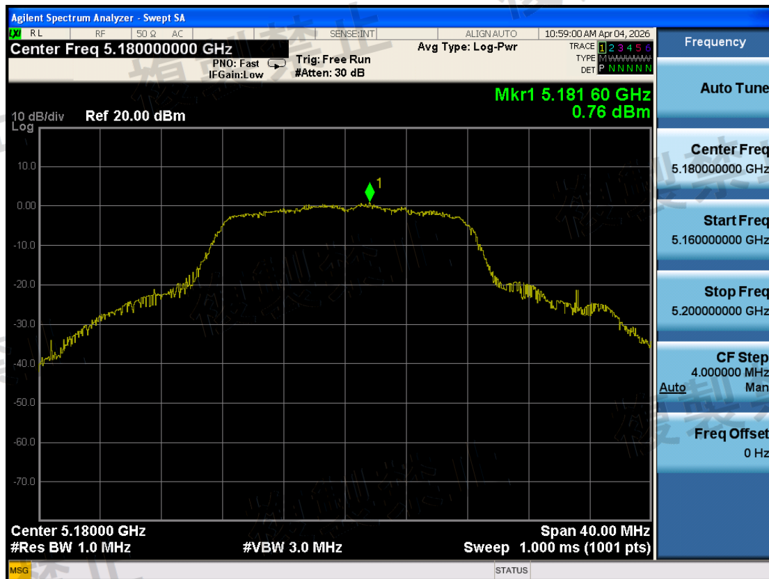
W52\Antenna Power Error\802.11a\1-5180-TX1-N
