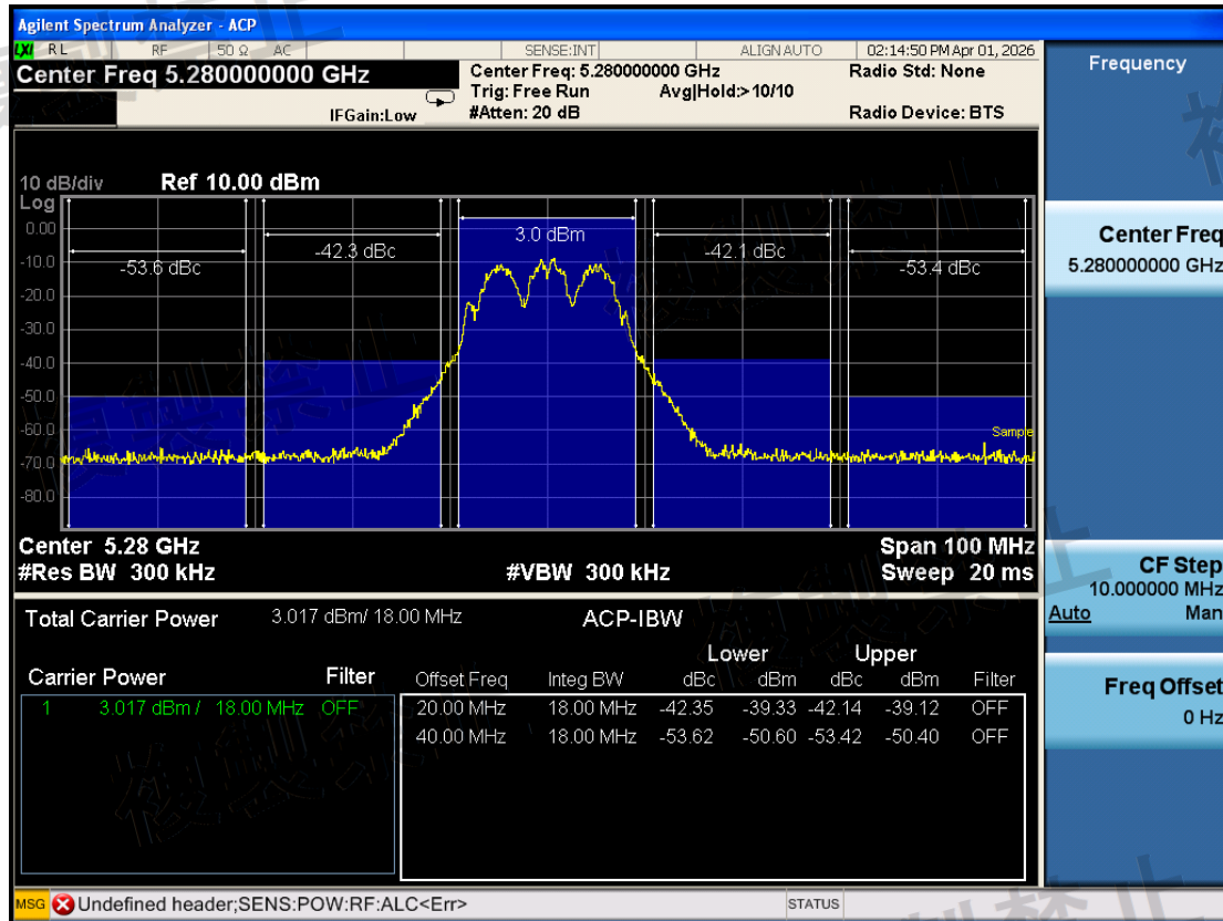
W53\Adjacent Channel Leakage Power\802.11a\5280-X-N
