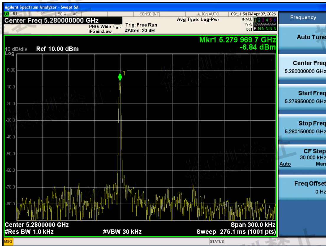
W53\Frequency Error Measurement\802.11ax HE20\5280-TX1-N
