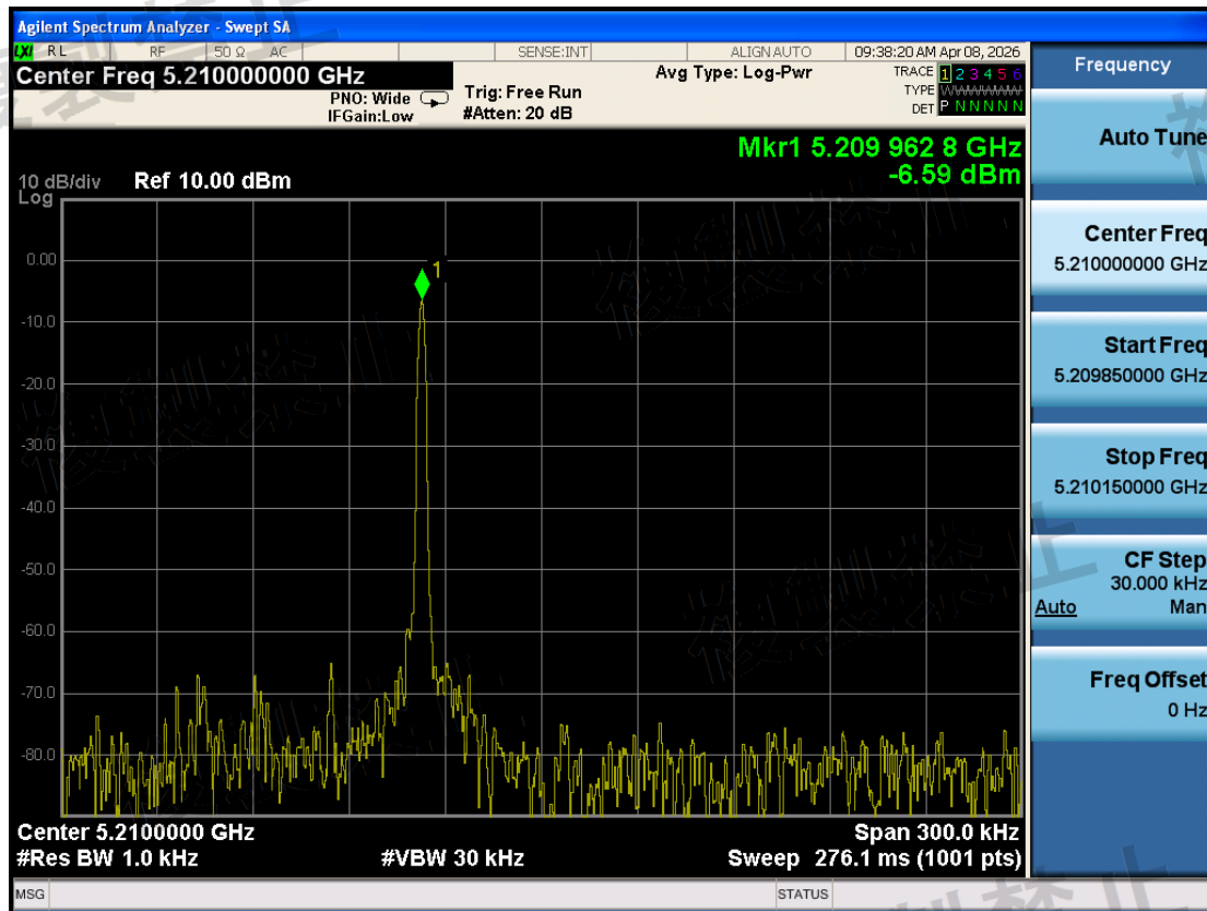
W52\Frequency Error Measurement\802.11ax HE80\5210-TX1-N
