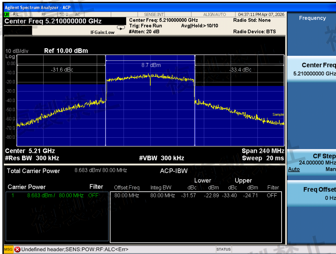
W52\Adjacent Channel Leakage Power\802.11ax HE80\5210-TX0-N
