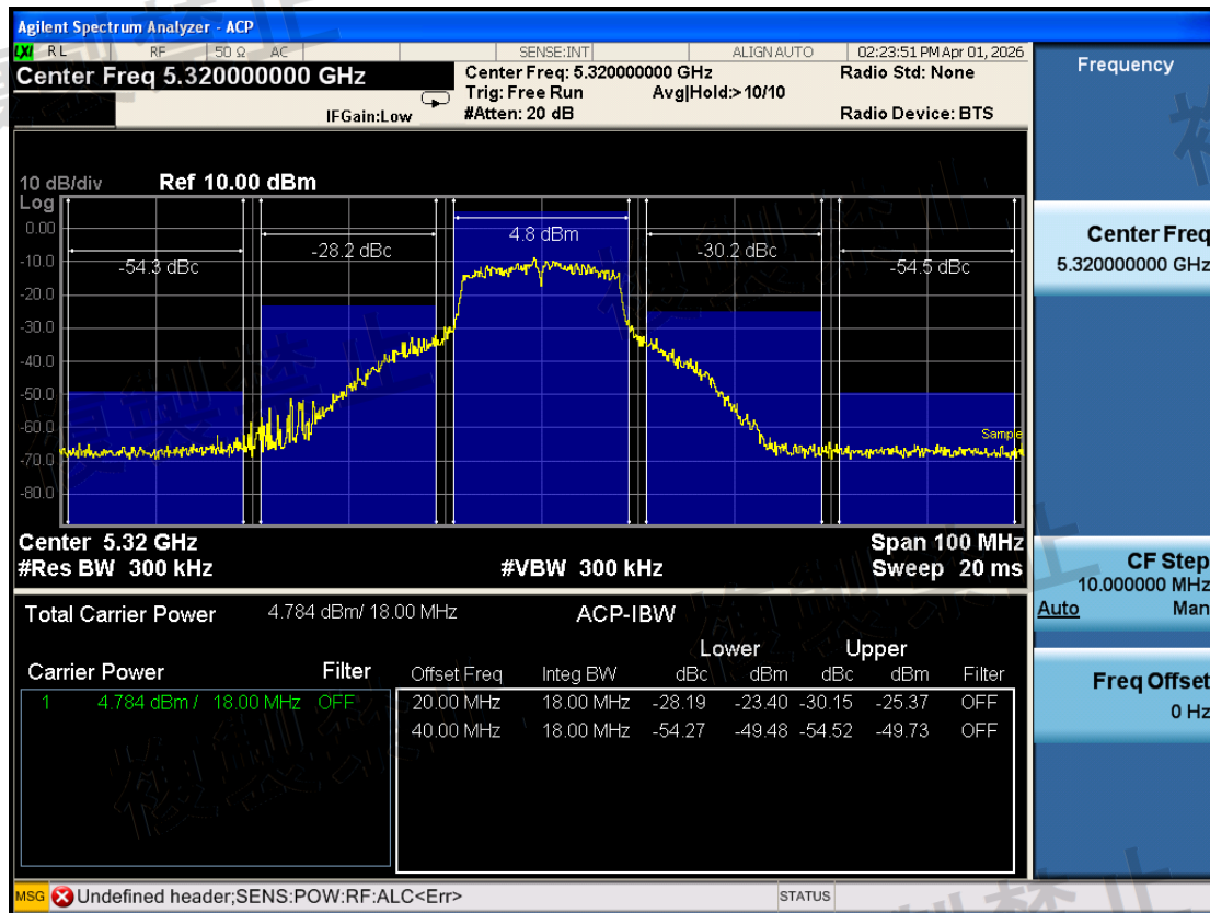
W53\Adjacent Channel Leakage Power\802.11a\5320-TX1-N
