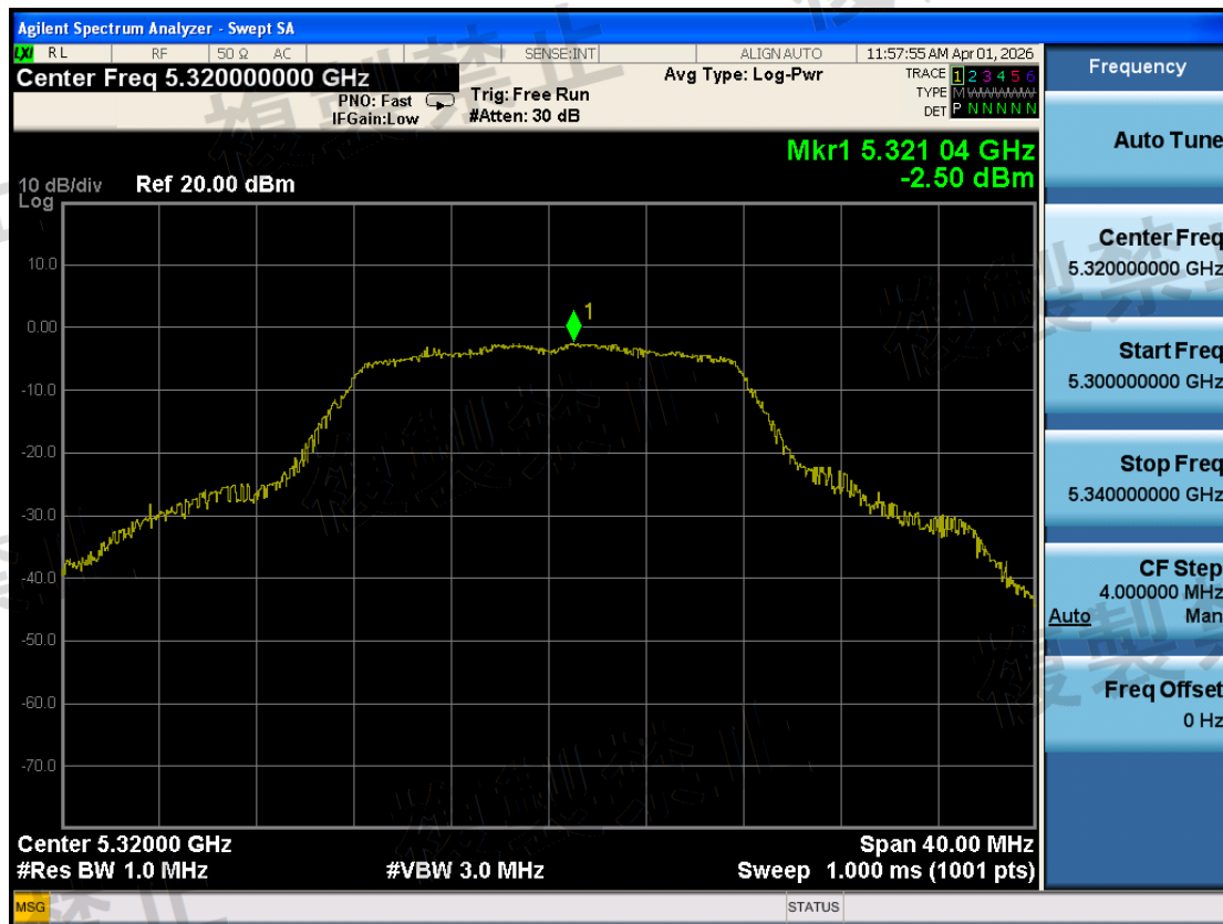
W53\Antenna Power Error\802.11a\1-5320-TX0-N
