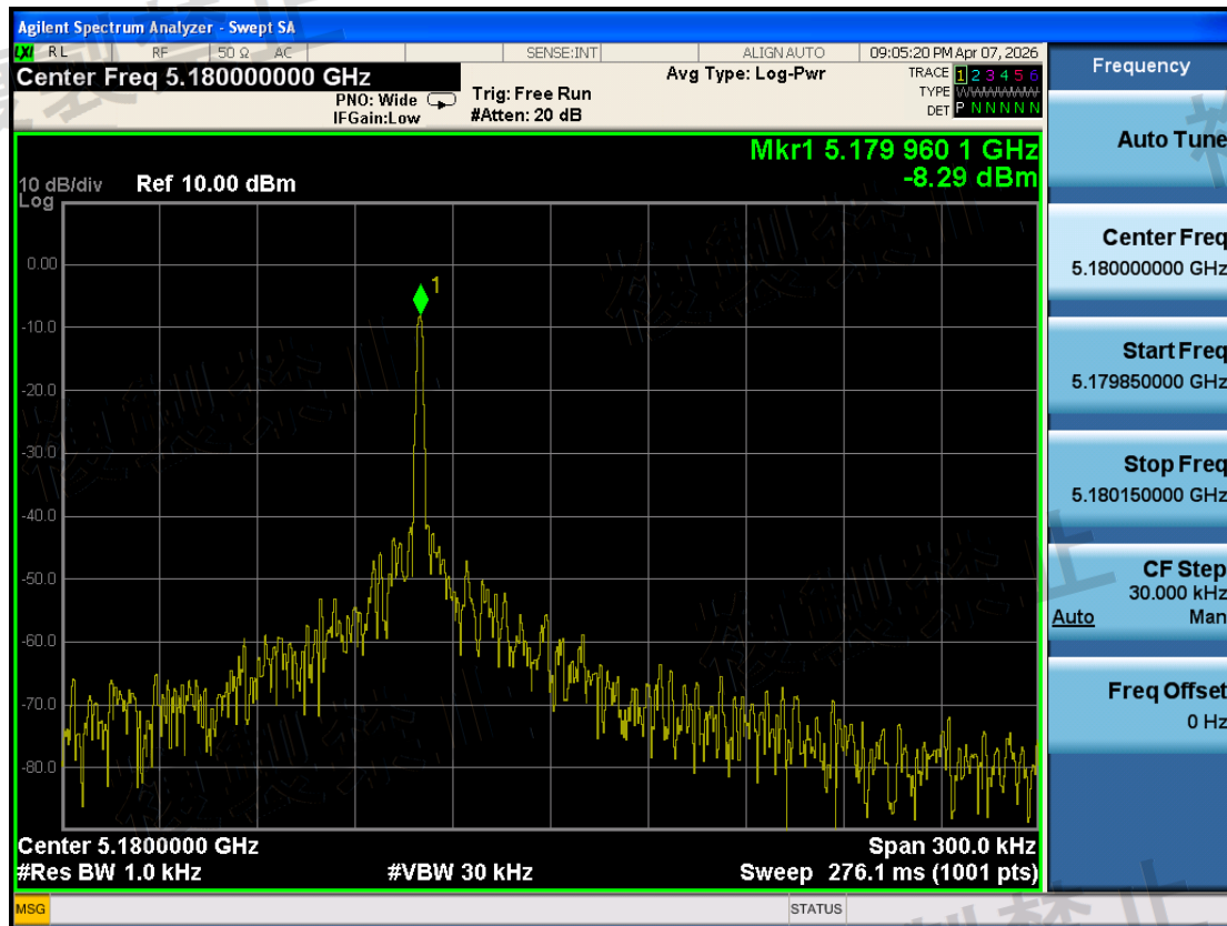
W52\Frequency Error Measurement\802.11a\5180-TX1-N
