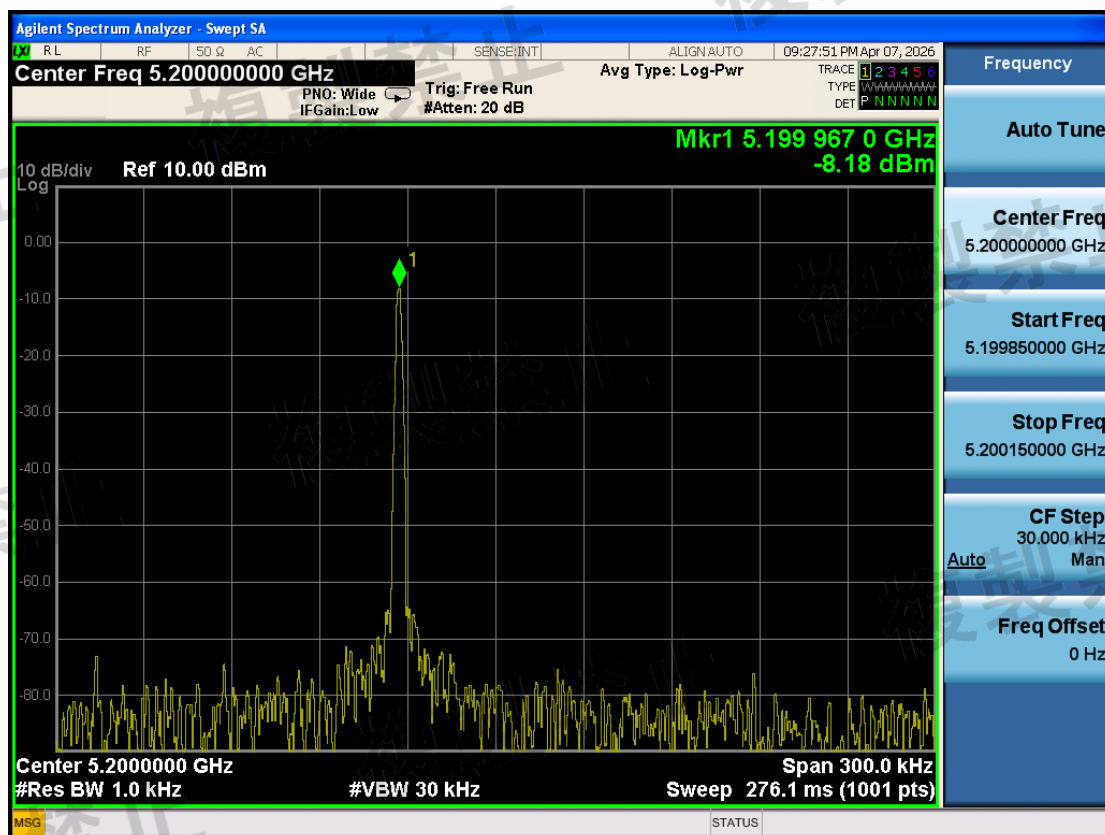
W52\Frequency Error Measurement\802.11ax HE20\5200-TX0-N
