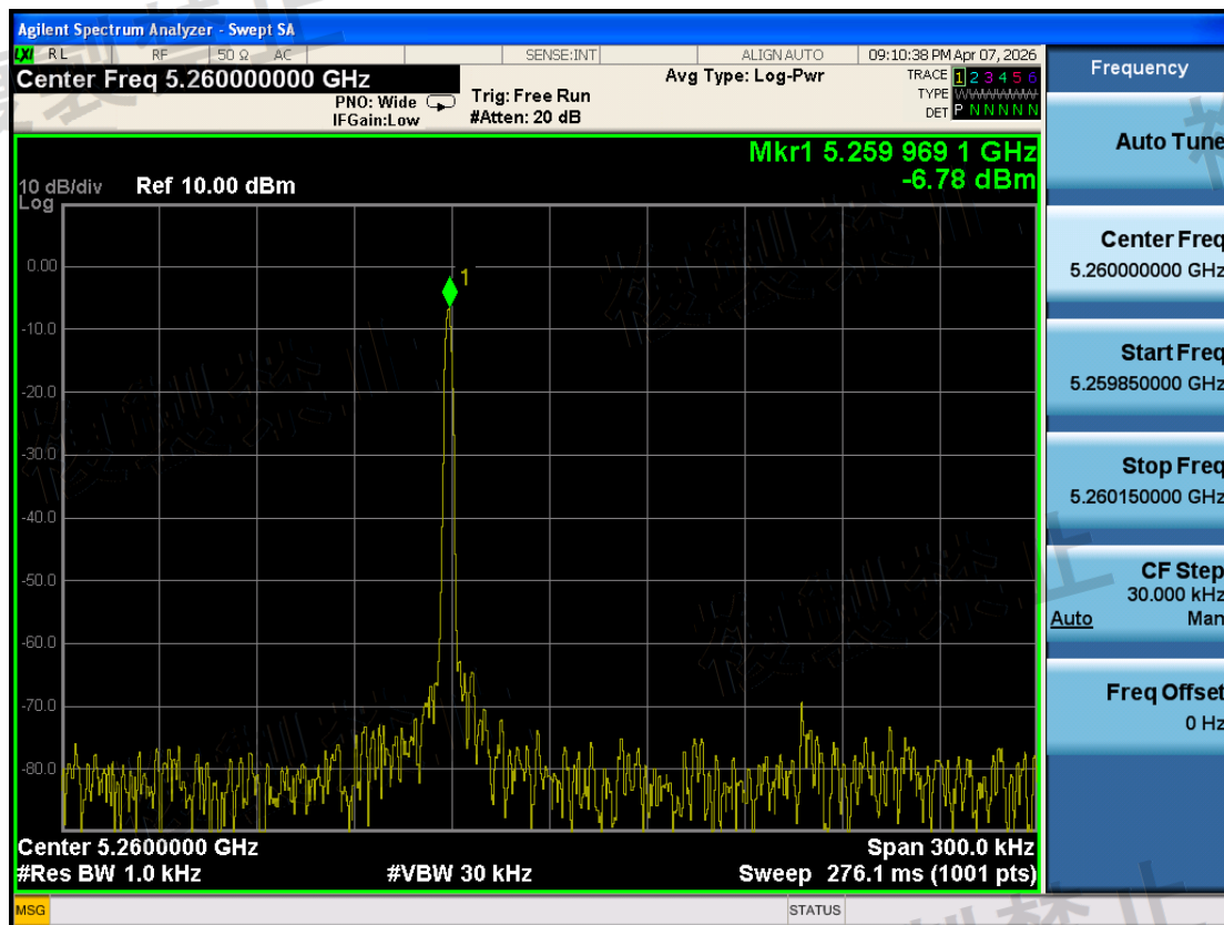
W53\Frequency Error Measurement\802.11ax HE20\5260-TX1-N
