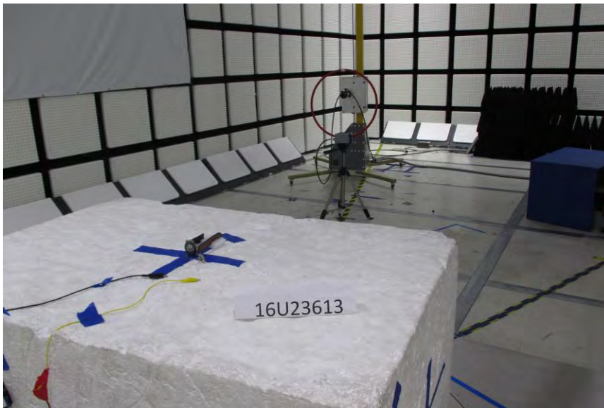
RADIATED BACK PHOTO – BELOW 30MHz
