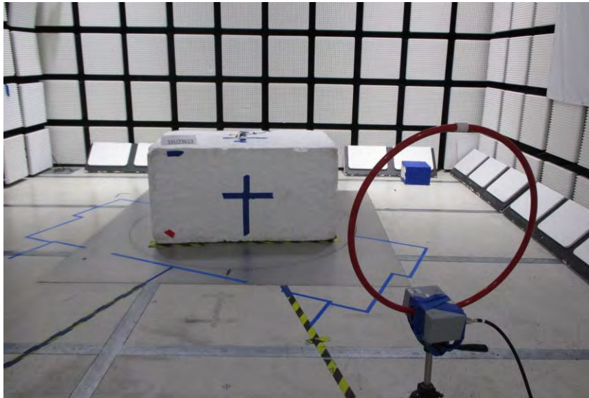
RADIATED FRONT PHOTO – BELOW 30MHz
