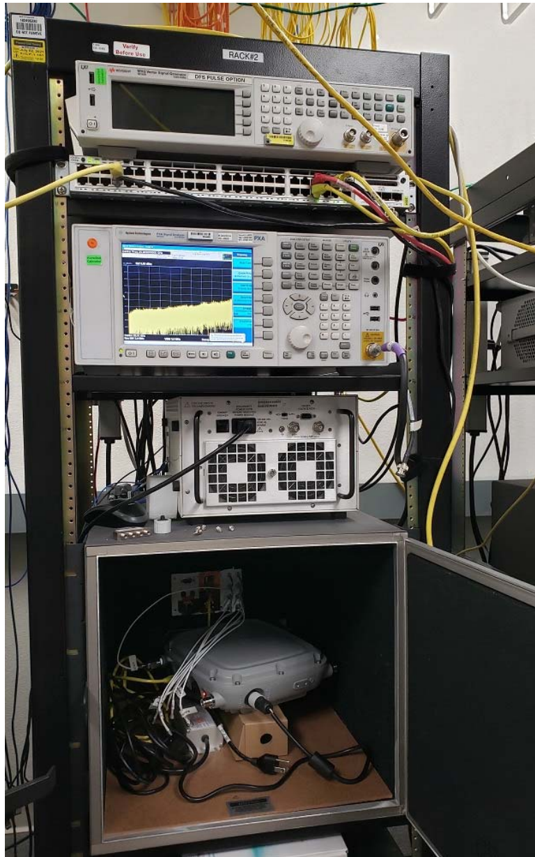
Title: Radio Conducted Test Setup – Rack 2
