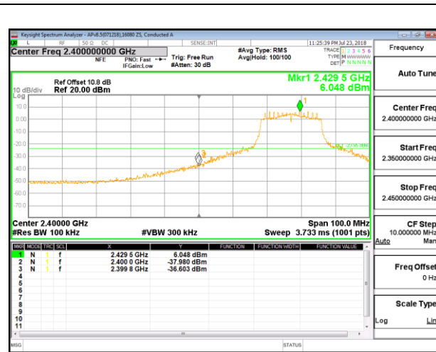
LOW CHANNEL 4 BANDEDGE
