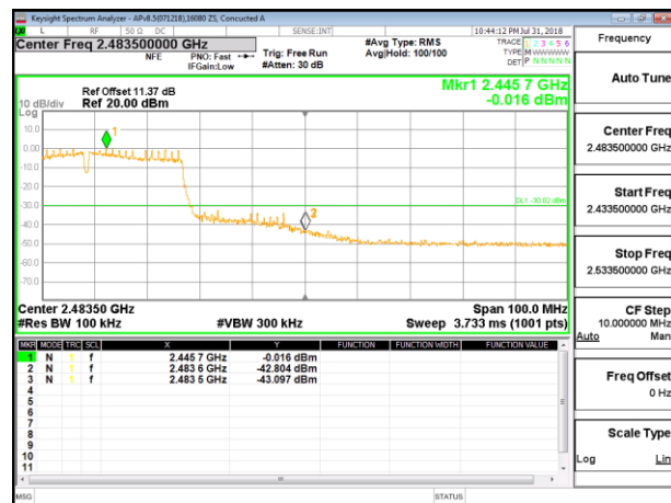
HIGH CHANNEL 7 BANDEDGE
