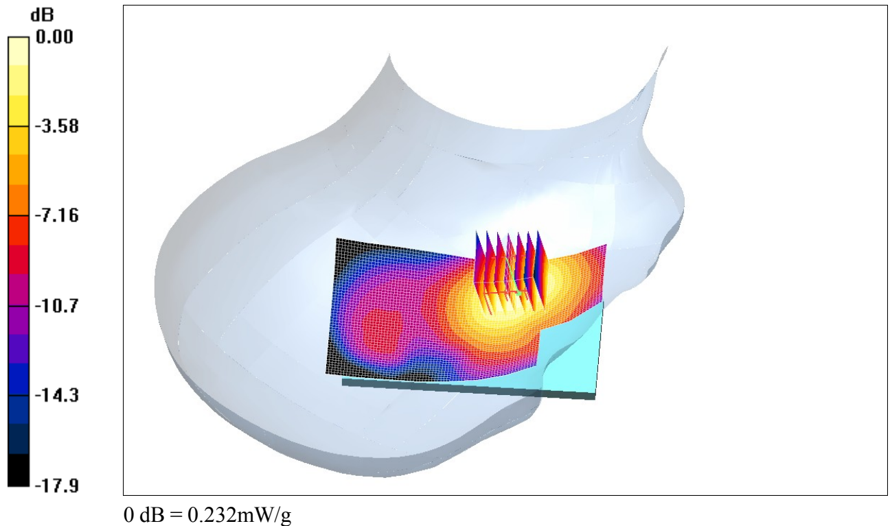
Fig. 5: SAR distribution for GSM1800 of the mobile phone with FAZUP: channel 699 (1747.6MHz), cheek position, right side
