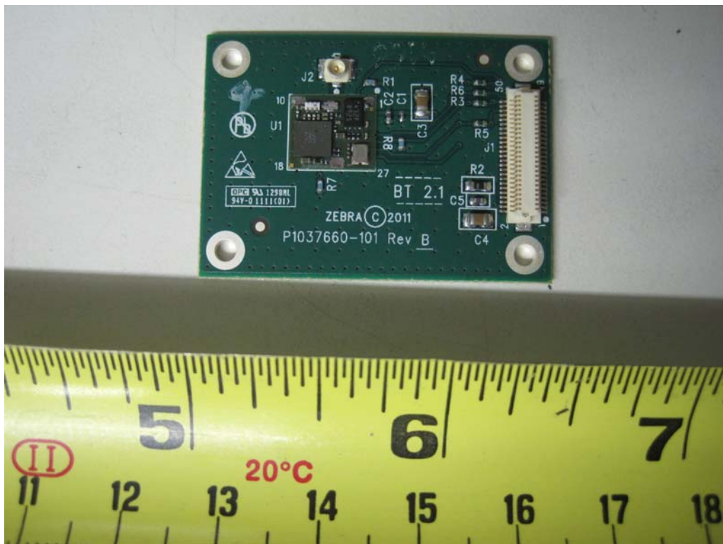
Radio Board shielding off View
