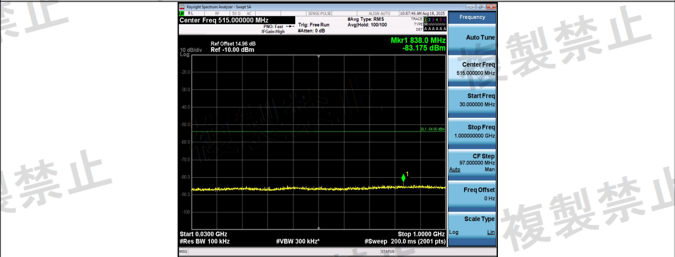
NTVN-11AX40MIMO-Ant2-5550-30~1000-PASS
