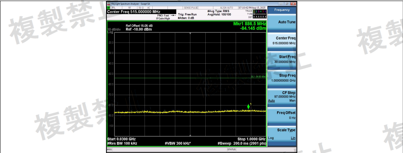
NTVN-11AX40MIMO-Ant2-5310-30~1000-PASS
