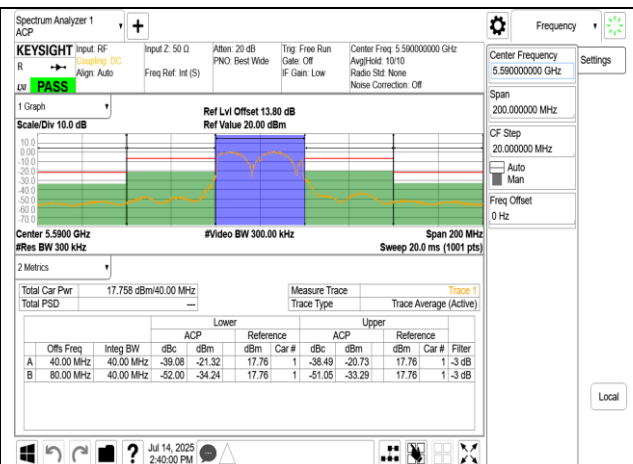
W56 802.11be 40MHz Chain0 Combine
