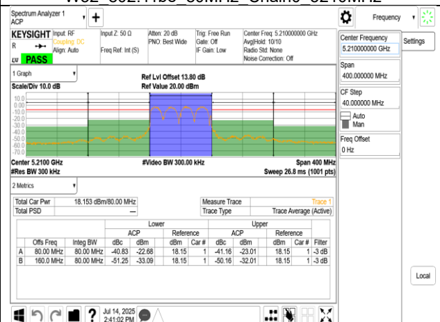
W52 802.11be 80MHz Chain0 Combine
