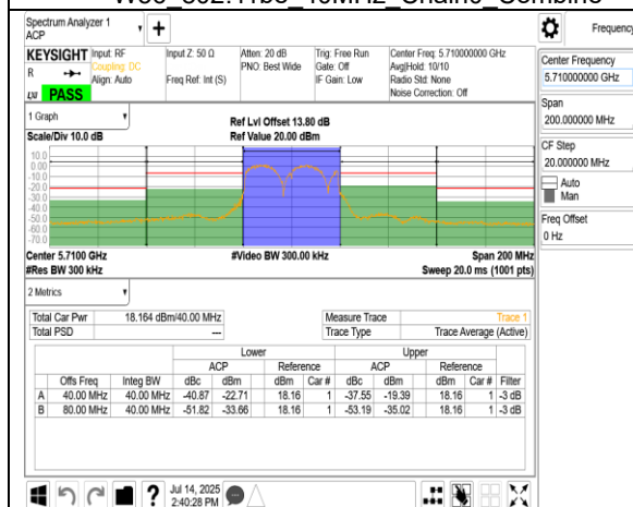
W56 802.11be 40MHz Chain0 Combine
