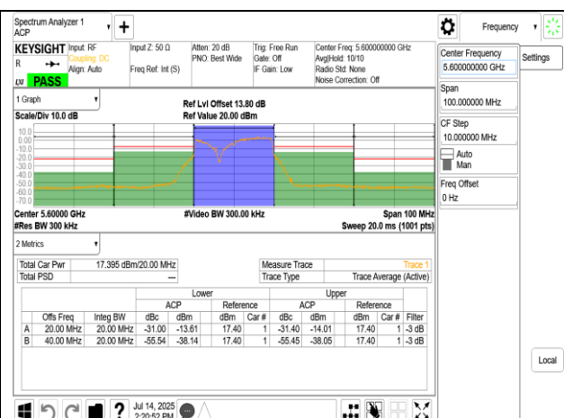
W56 802.11ax 20MHz Chain0 Combine
