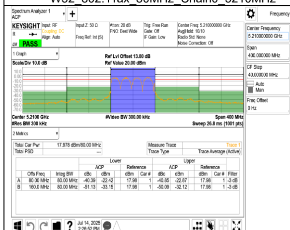
W52 802.11ax 80MHz Chain0 Combine
