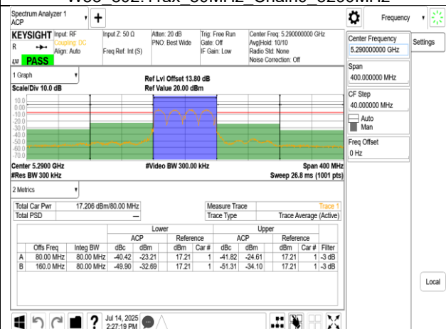
W53 802.11ax 80MHz Chain0 Combine
