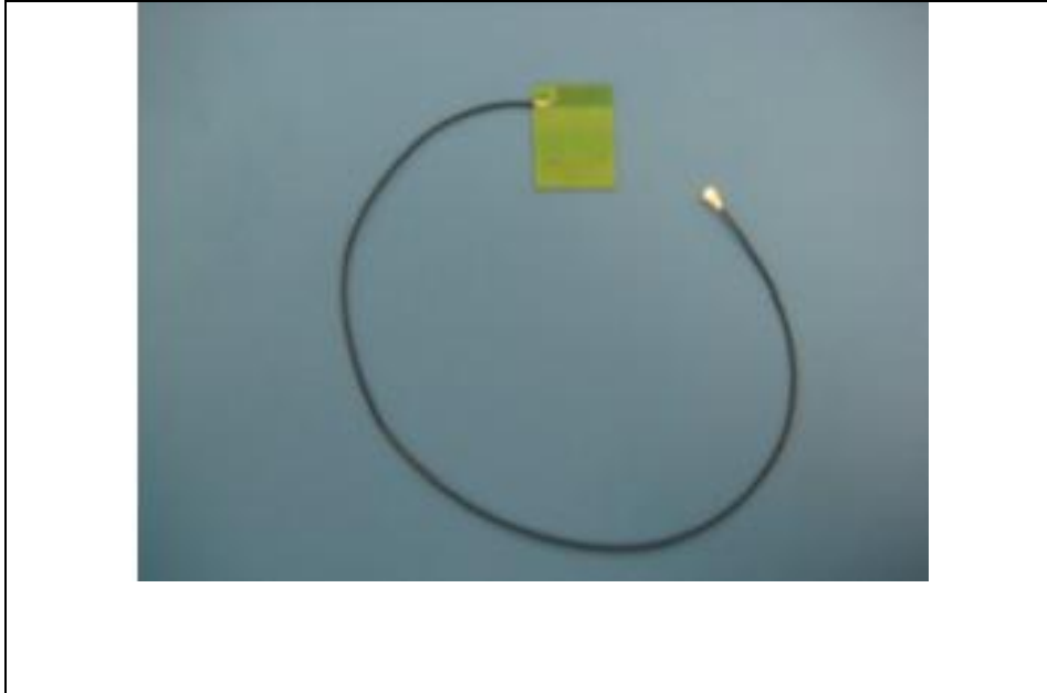
Antenna 18: Brand : Tyco / Model : TBN007 (TX1) / TBN007 (TX2 or RX2) (For WLAN & BT Used)
