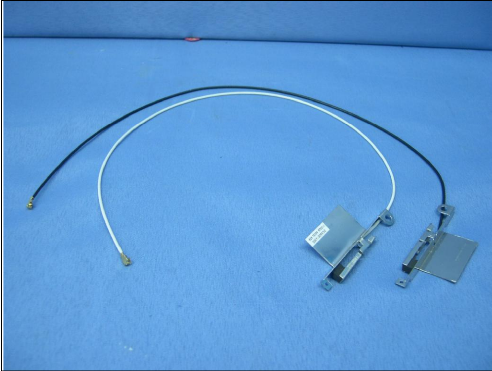
Antenna 1: Brand : WNC / Model : 81.EBJ15.005 (For WLAN & BT Used)
