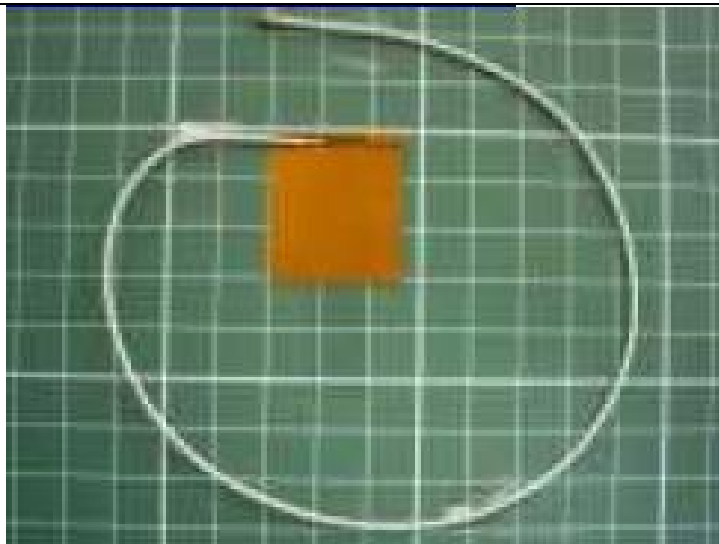
Antenna 14: Brand : Hitachi Cable / Model : HCY01 (TX1) / HCY01 (TX2) (For WLAN & BT Used)
