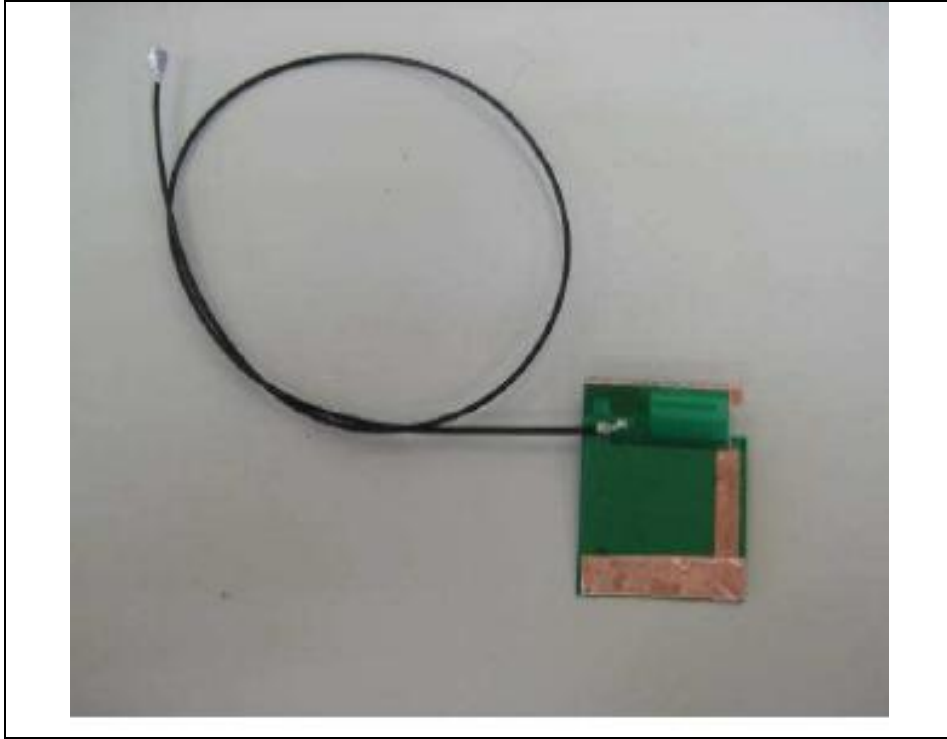
Antenna 22: Brand : Tyco / Model : TBN009 (TX1) / TBN009 (TX2 or RX2) (For WLAN & BT Used)
