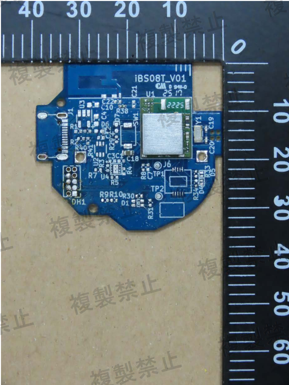
Inverted F Antenna
