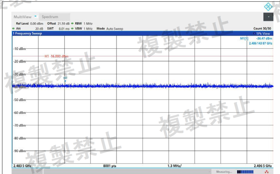
NTNV-11BE40MIMO-Ant1-2442-2483.5~2496.5-PASS
