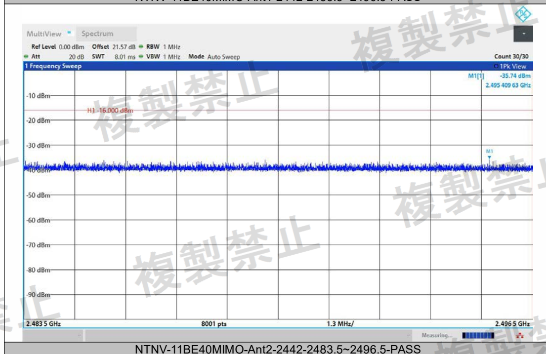
NTNV-11BE40MIMO-Ant2-2442-2483.5~2496.5-PASS
