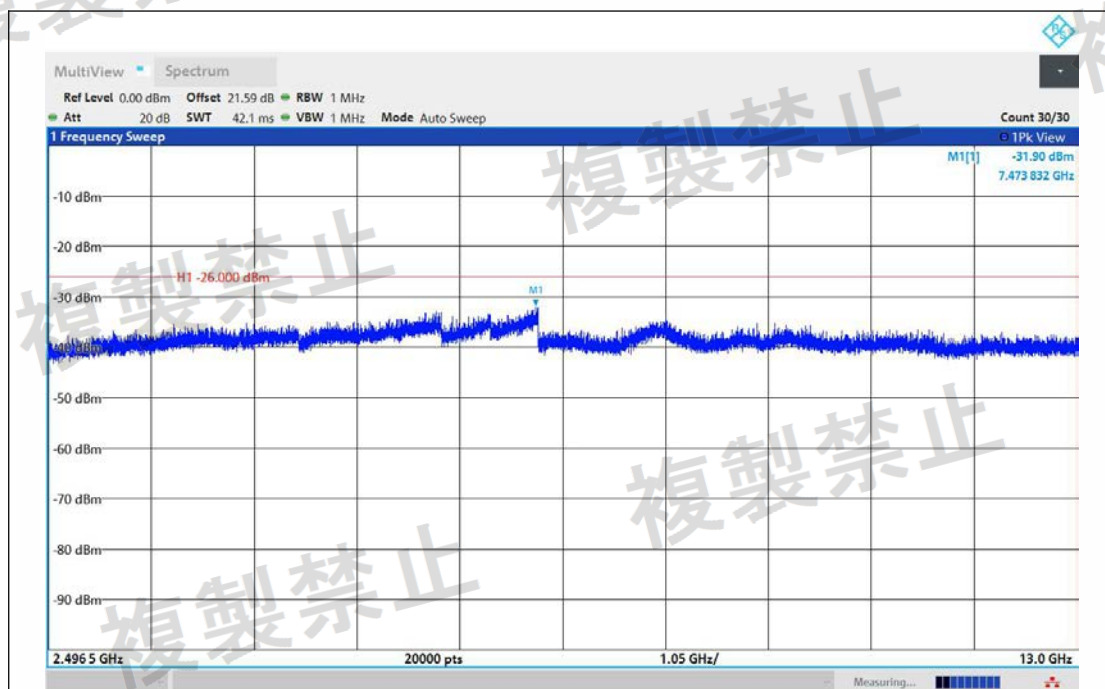
NTVN-11AX20MIMO-Ant1-2442-2496.5~13000-PASS
