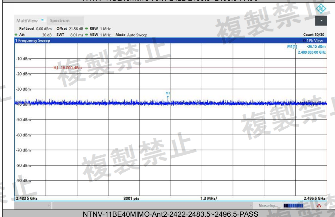
NTNV-11BE40MIMO-Ant2-2422-2483.5~2496.5-PASS
