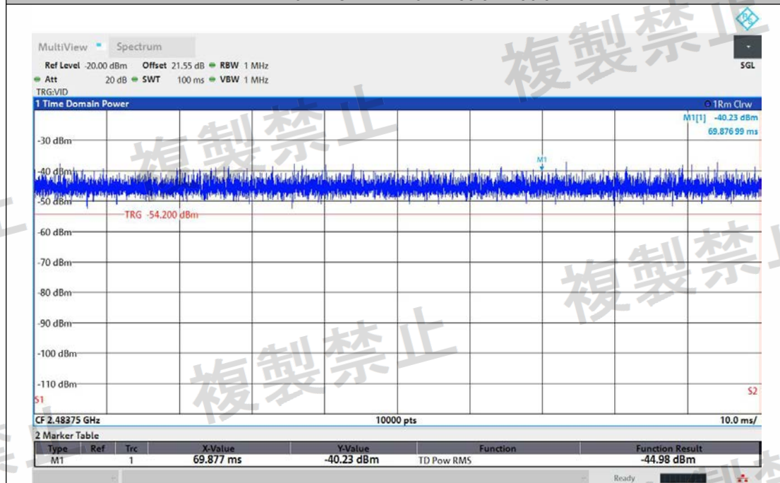
NTNV-11AX40MIMO-Ant1-2462-2483.5~2496.5-PASS
