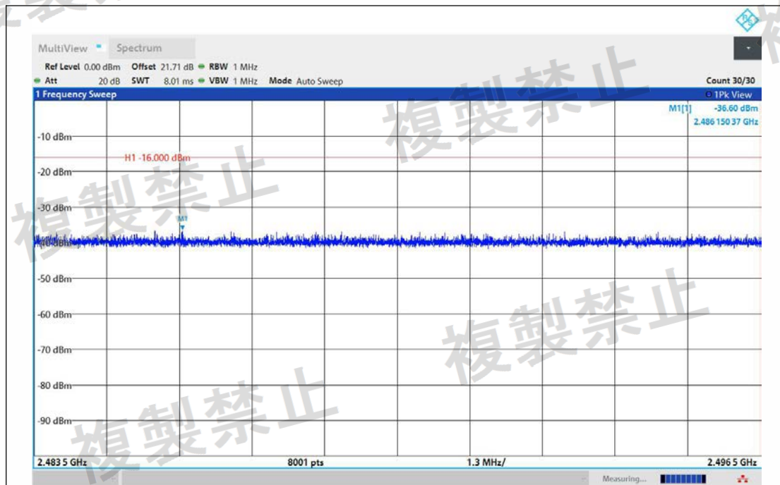
NTNV-11AX20MIMO-Ant1-2412-2483.5~2496.5-PASS
