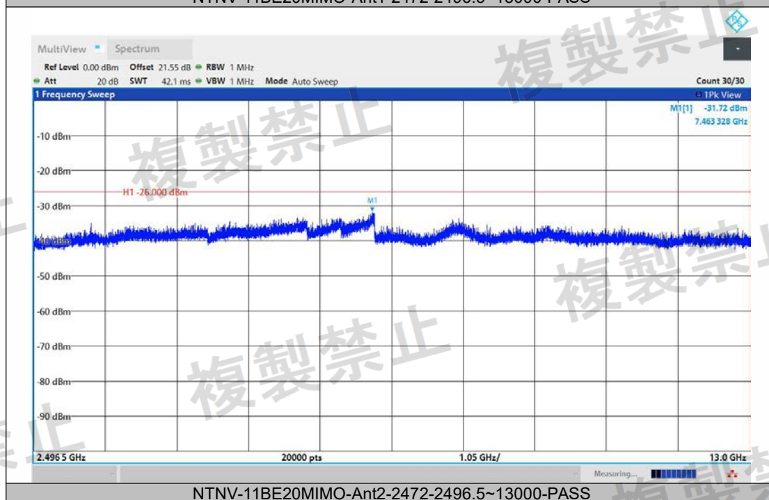
NTVN-11BE20MIMO-Ant1-2472-2496.5~13000-PASS
