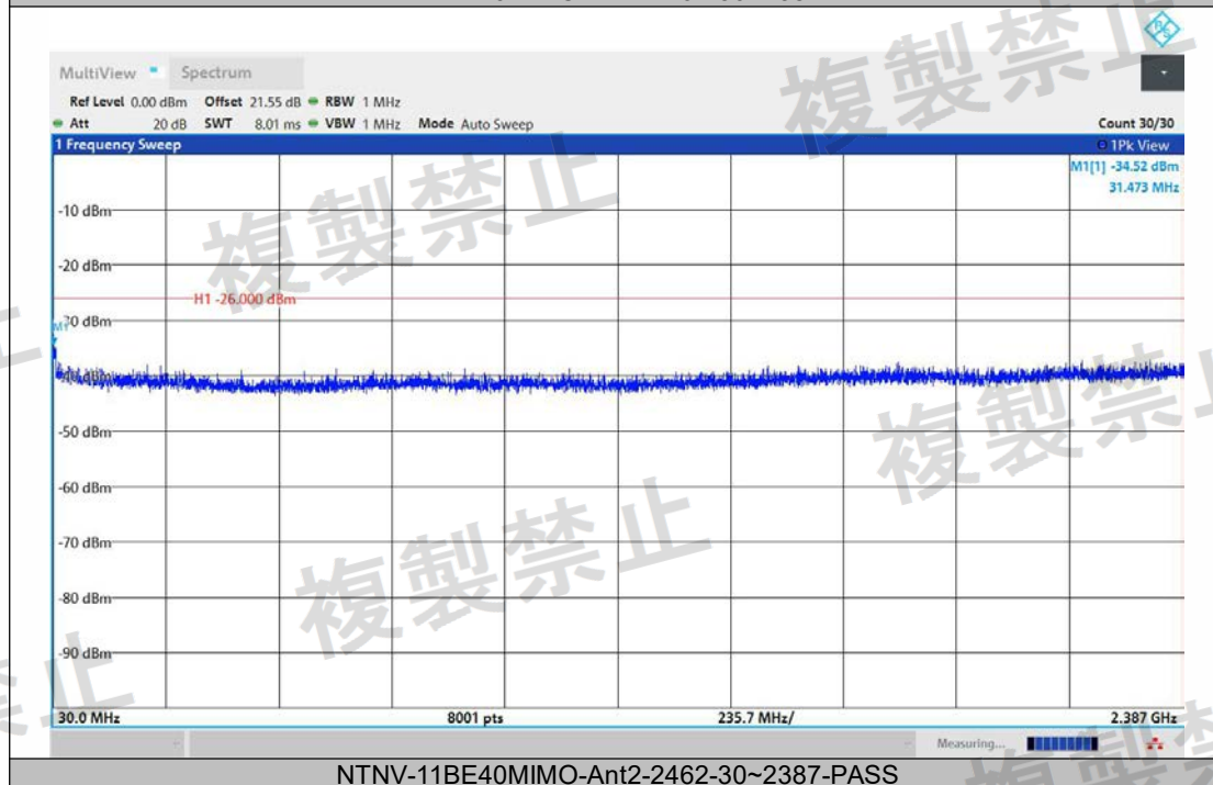
NTNV-11BE40MIMO-Ant2-2462-30~2387-PASS
