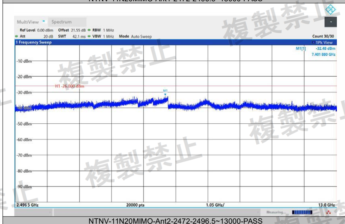
NTNV-11N20MIMO-Ant1-2472-2496.5~13000-PASS
