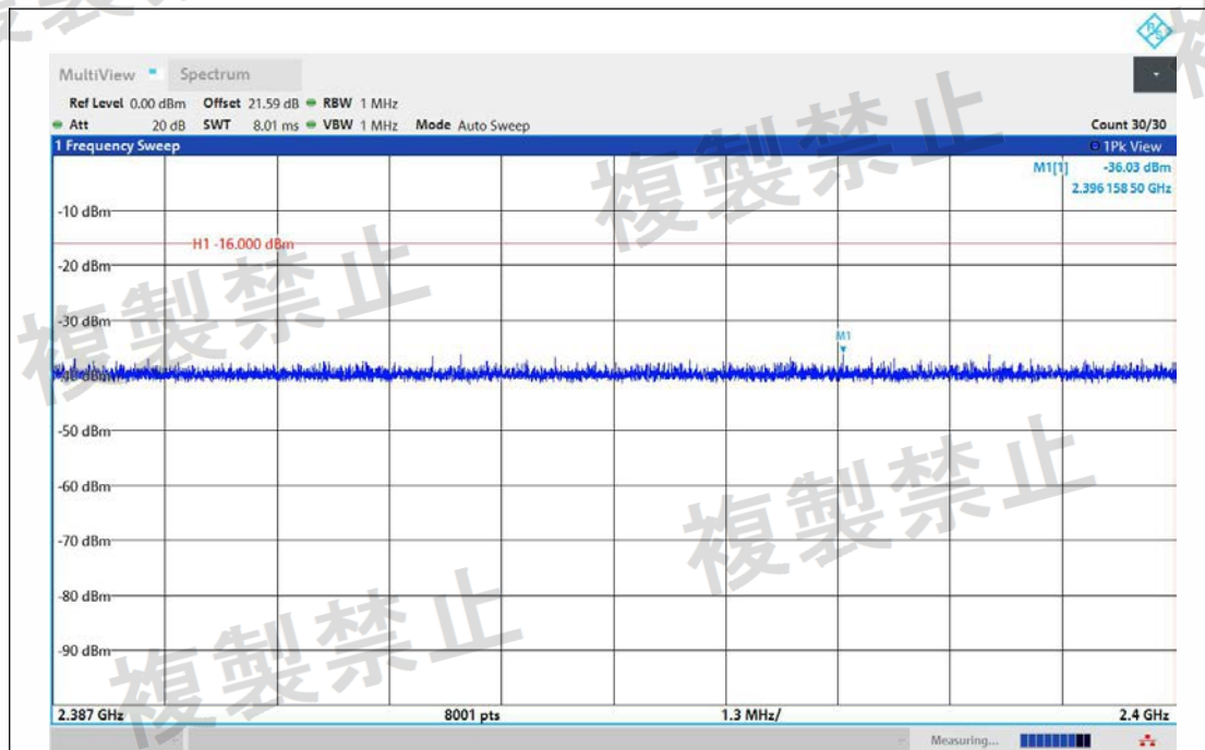
NTVN-11N40MIMO-Ant1-2442-2387~2400-PASS
