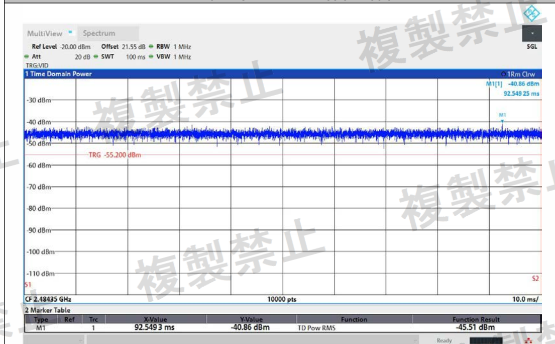
NTNV-11AX20MIMO-Ant1-2472-2483.5~2496.5-PASS
