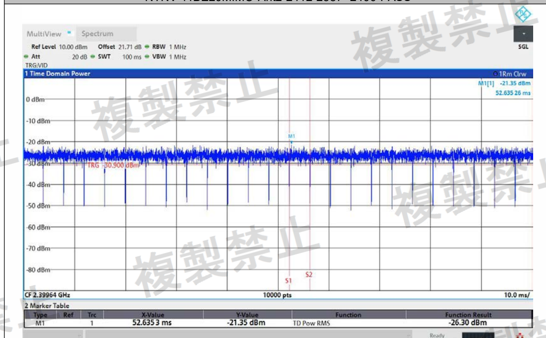
NTNV-11BE20MIMO-Ant2-2412-2387~2400-PASS
