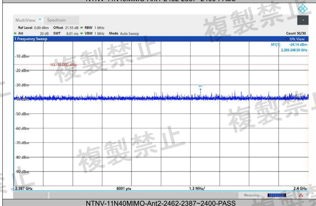
NTNV-11N40MIMO-Ant2-2462-2387~2400-PASS
