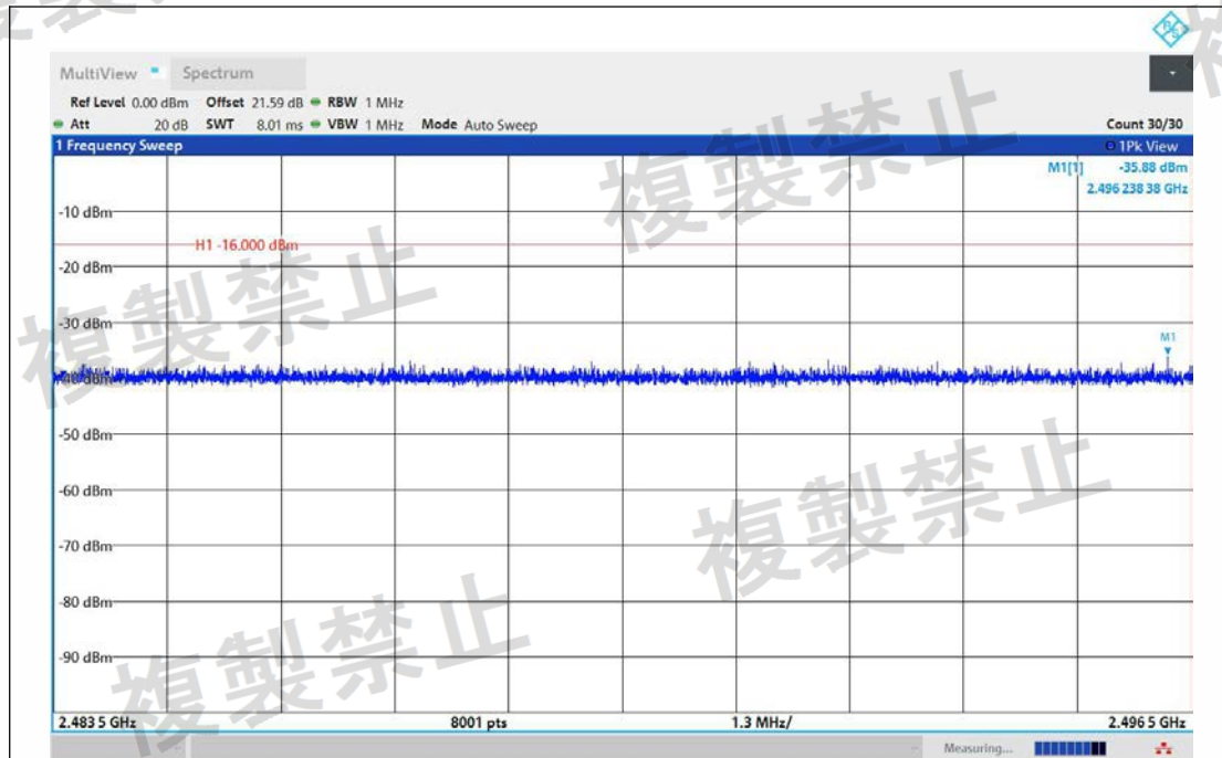
NTNV-11N20MIMO-Ant1-2442-2483.5~2496.5-PASS
