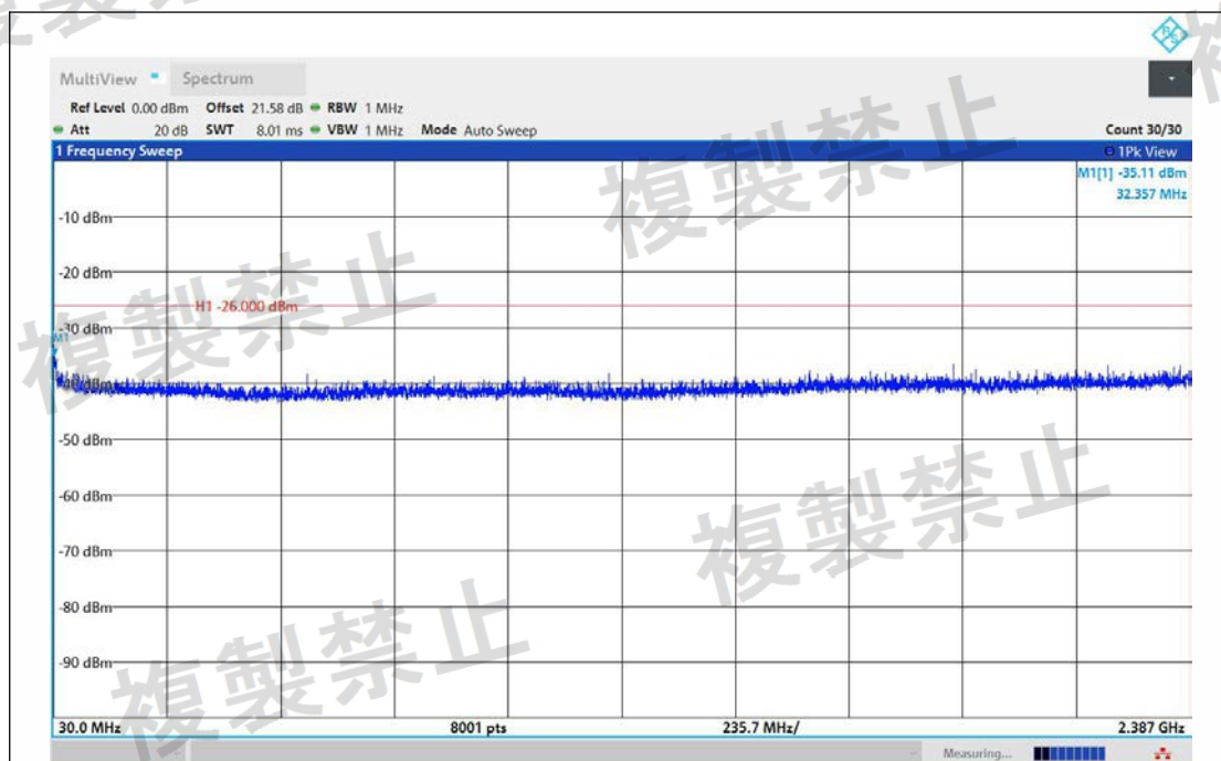
NTNV-11N40MIMO-Ant1-2462-30~2387-PASS
