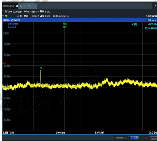
NTVN-11AX20SISO-Ant3-5180-5266.7~26000-P ASS
