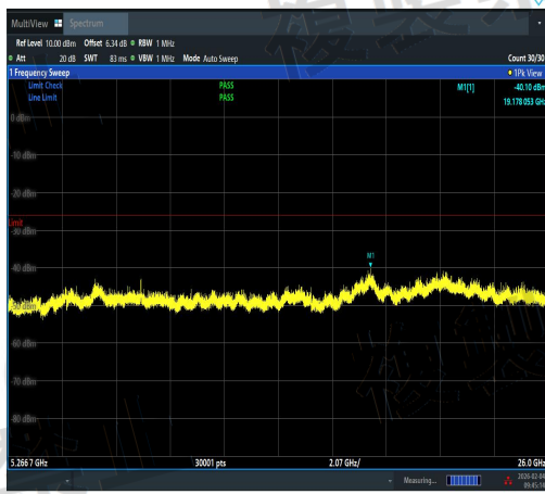
NTVN-11AC20MIMO-Ant3-5180-5260~5266.7-P ASS
