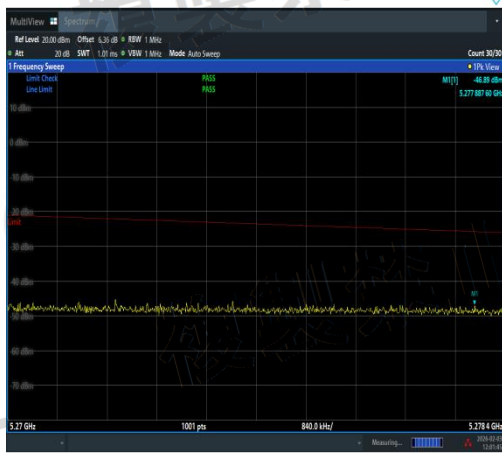
NTNV-11AC40SISO-Ant1-5230-5270~5278.4-PA
