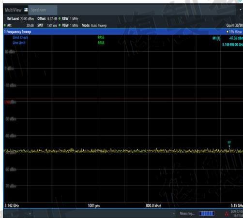
NTNV-11AC20SISO-Ant2-5240-5142~5150-PASS
