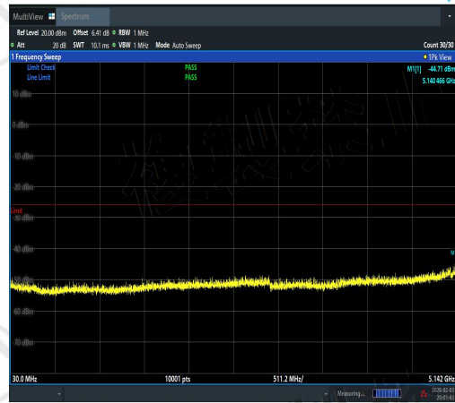
NTVN-11AX20SISO-Ant3-5220-30~5142-PASS
