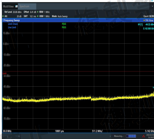
NTNV-11AC20SISO-Ant3-5220-30~5142-PASS
