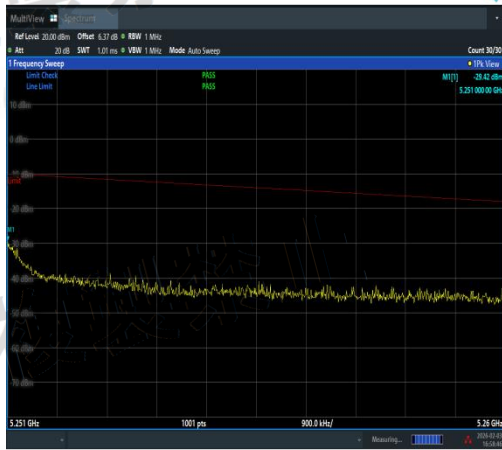
NTNV-11AC20SISO-Ant2-5240-5251~5260-PAS
