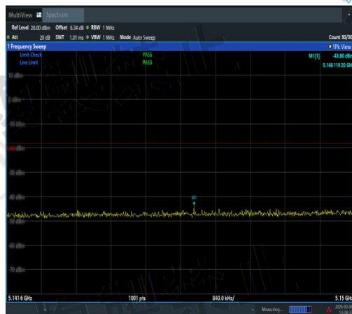
NTNV-11N40MIMO-Ant2-5190-5141.6~5150-PA SS
