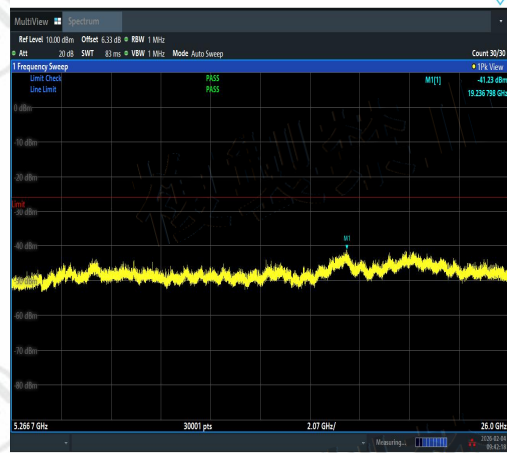
NTVN-11AC20MIMO-Ant1-5180-5266.7~26000-P PASS
