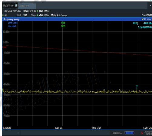
NTNV-11AC40SISO-Ant3-5190-5250~5251-PAS
