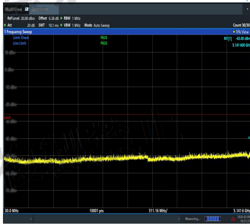
NTNV-11AC40MIMO-Ant3-5190-30~5141.6-PAS S
