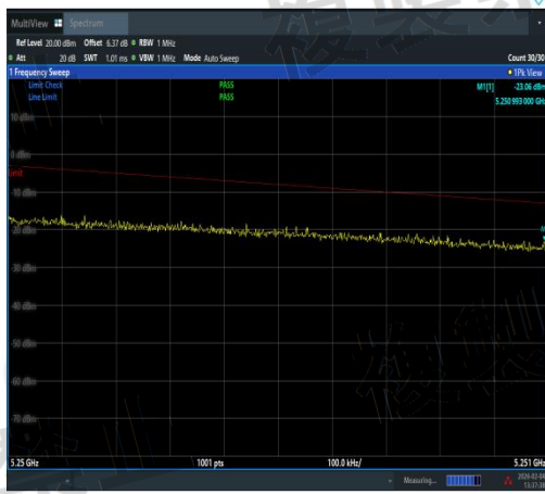
NTVN-11N40MIMO-Ant1-5230-5250~5251-See table below
