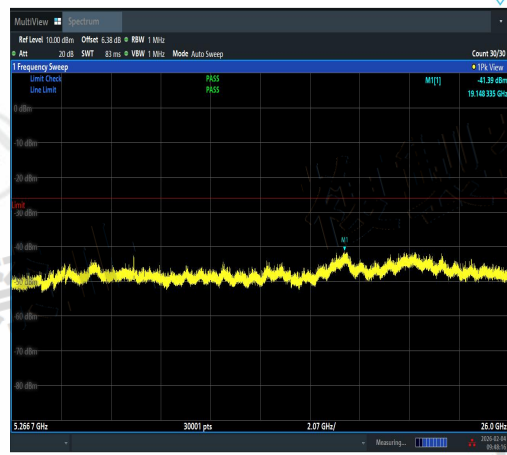
NTVN-11AC20MIMO-Ant1-5180-5266.7~26000-P PASS
