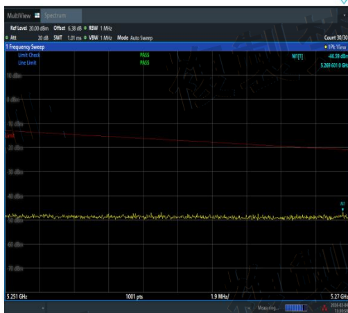
NTVN-11N40MIMO-Ant3-5190-5251~5270-PASS
