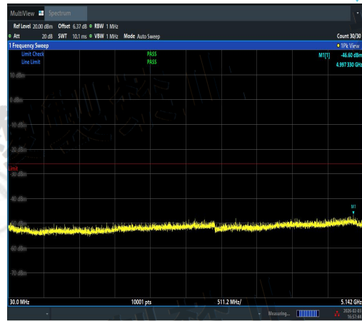
NTNV-11AC20SISO-Ant2-5240-30~5142-PASS
