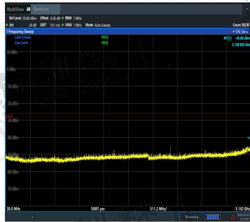
NTVN-11AX20SISO-Ant1-5220-30~5142-PASS
