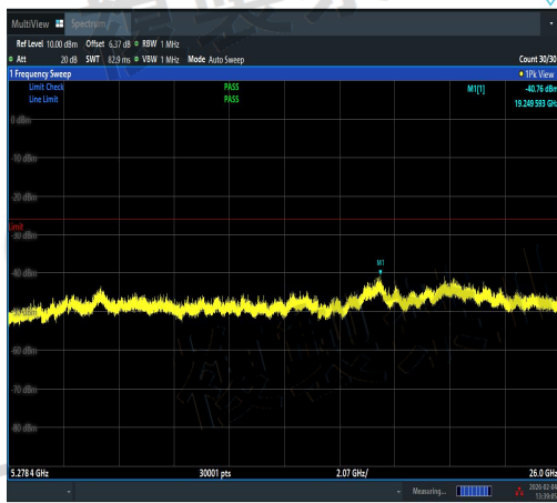
NTVN-11N40MIMO-Ant2-5230-5278.4~26000-P ASS
