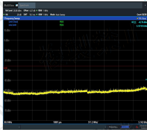
NTNV-11AC20SISO-Ant2-5220-30~5142-PASS
