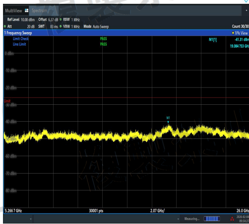
NTVN-11AC20MIMO-Ant2-5220-5266.7~26000- PASS
