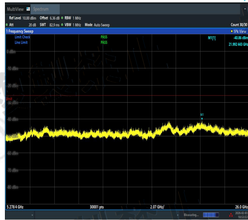
NTNV-11N40SISO-Ant1-5230-5278.4~26000-PA
