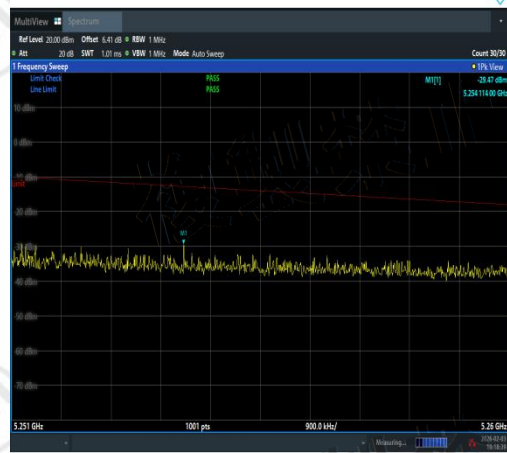
NTNV-11AC20SISO-Ant3-5220-5251~5260-PAS
