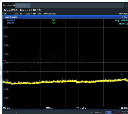
NTNV-11N40MIMO-Ant2-5190-30~5141.6-PASS
