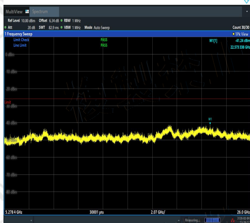
NTVN-11N40MIMO-Ant2-5190-5278.4~26000-P
