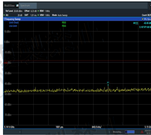
NTNV-11AC40MIMO-Ant1-5190-5141.6~5150-P ASS
