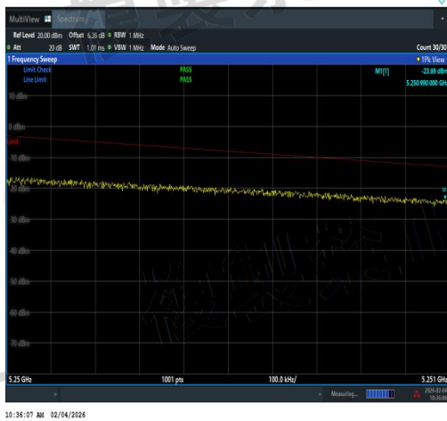
NTVN-11AC40MIMO-Ant1-5230-5250~5251-See table below
