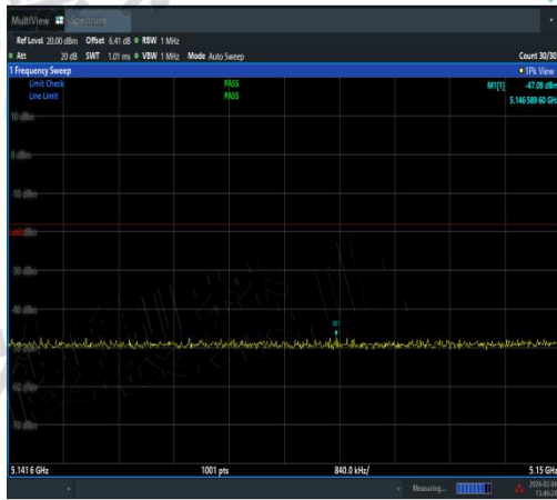
NTVN-11N40MIMO-Ant3-5230-5141.6~5150-PA SS
