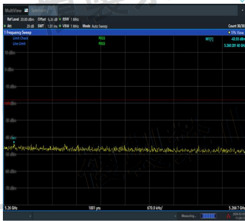
NTNV-11AC20SISO-Ant1-5240-5260~5266.7-PA
