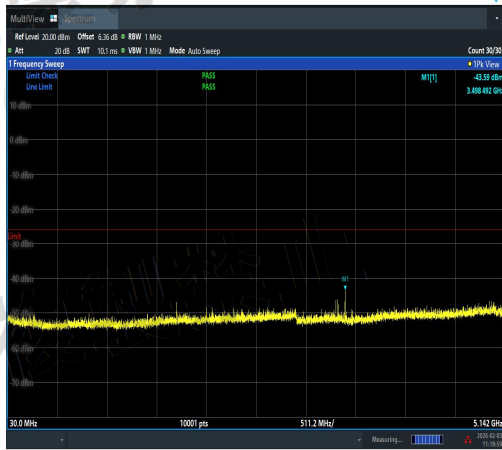
NTNV-11AC20SISO-Ant1-5240-30~5142-PASS
