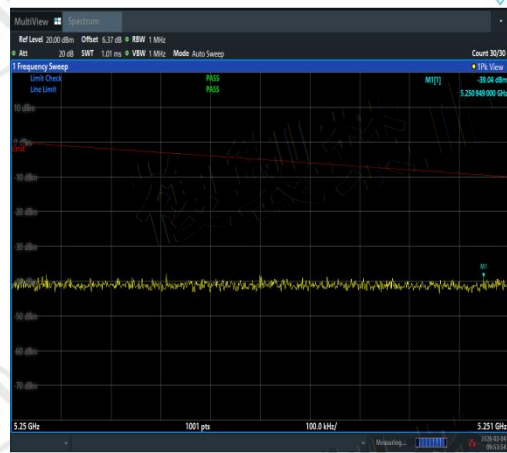
NTNV-11AC20MIMO-Ant2-5220-5250~5251-PAS
