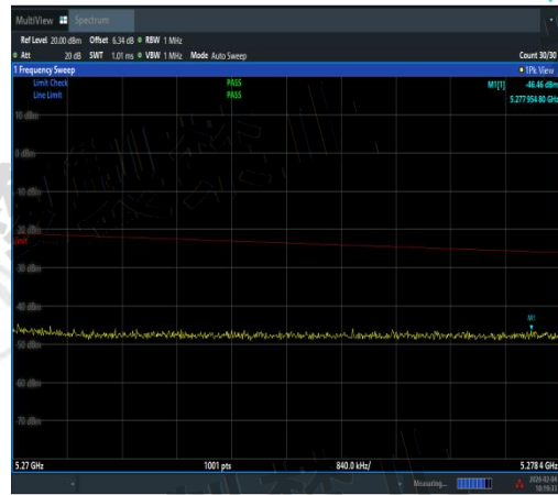
NTNV-11AC40MIMO-Ant2-5190-5270~5278.4-P ASS
