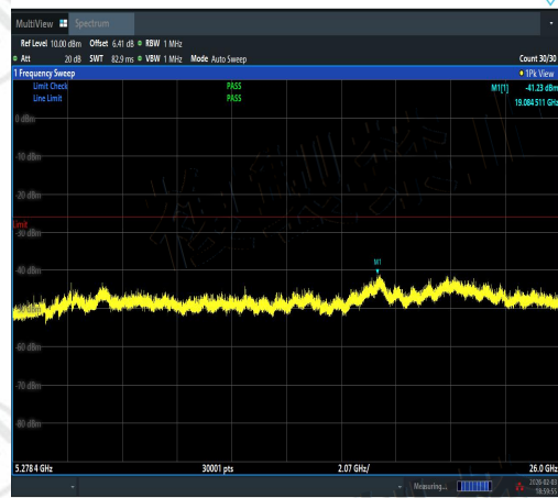
NTNV-11N40SISO-Ant3-5230-5278.4~26000-PA
