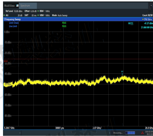
NTVN-11AC20MIMO-Ant1-5220-5266.7~26000- PASS
