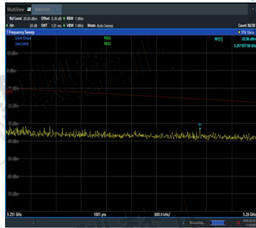
NTNV-11AC20SISO-Ant1-5220-5251~5260-PAS
