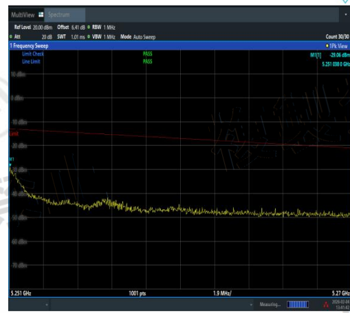
NTVN-11N40MIMO-Ant3-5230-5250~5251-See table below
