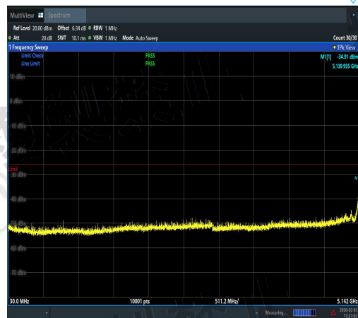
NTNV-11AX20SISO-Ant2-5180-30~5142-PASS
