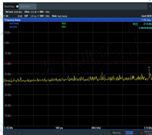
NTNV-11AX20SISO-Ant1-5180-5142~5150-PASS
