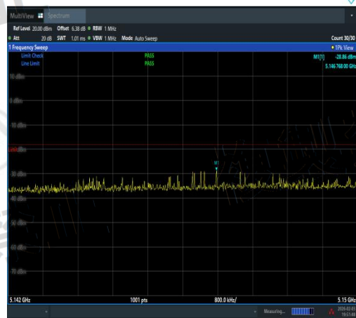
NTNV-11AX20SISO-Ant3-5180-5142~5150-PASS
