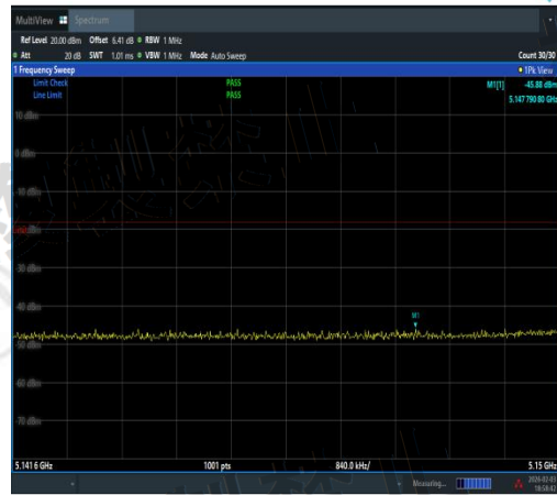
NTVN-11N40SISO-Ant3-5230-5141.6~5150-PAS
