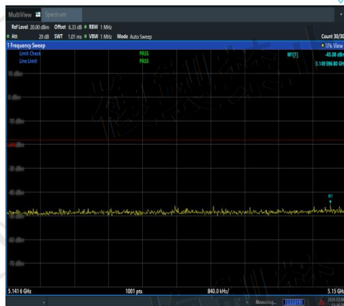
NTNV-11N40MIMO-Ant1-5190-5141.6~5150-PA SS
