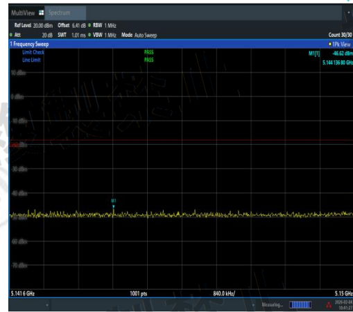
NTVN-11AC40MIMO-Ant3-5230-5141.6~5150-P ASS
