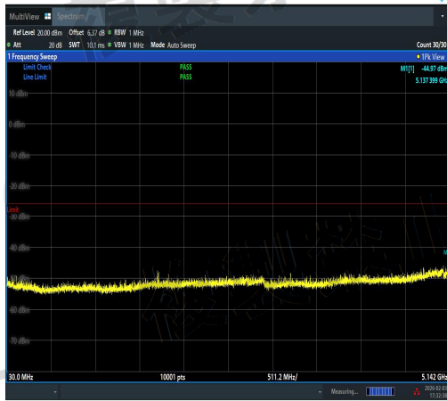
NTVN-11AX20SISO-Ant2-5220-30~5142-PASS
