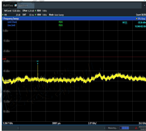
NTNV-11AC20SISO-Ant2-5180-5266.7~26000-P ASS
