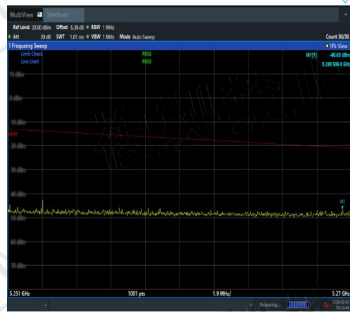
NTNV-11AC40SISO-Ant3-5190-5251~5270-PAS
