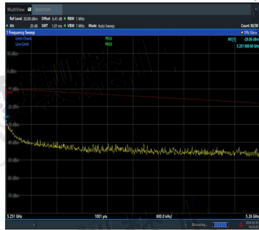
NTNV-11AC20SISO-Ant3-5240-5251~5260-PAS
