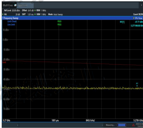
NTVN-11N40MIMO-Ant3-5230-5270~5278.4-PA SS
