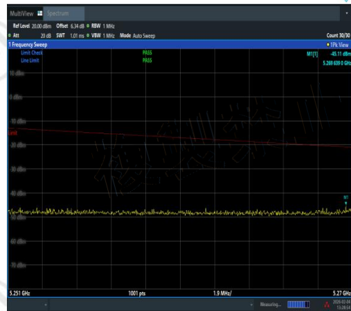
NTVN-11N40MIMO-Ant2-5190-5251~5270-PASS
