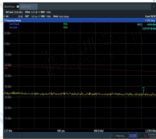
NTNV-11AC40SISO-Ant2-5230-5270~5278.4-PA
