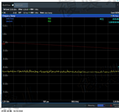
NTNV-11AX20SISO-Ant1-5180-5251~5260-PAS S
