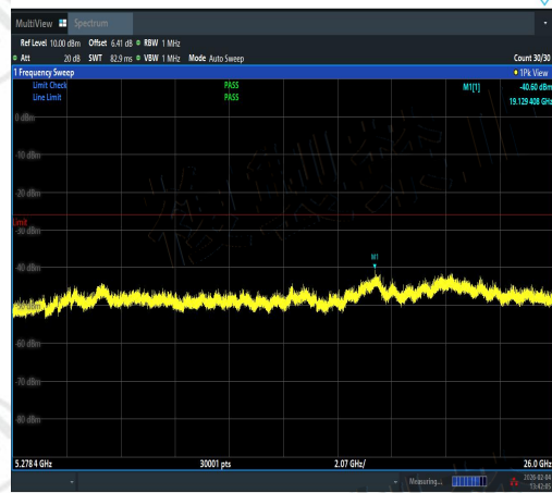
NTVN-11N40MIMO-Ant3-5230-5278.4~26000-P ASS
