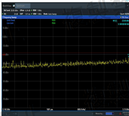
NTNV-11AX20SISO-Ant2-5180-5142~5150-See
