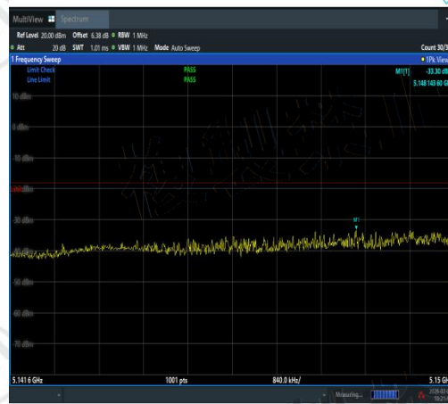
NTNV-11AC40MIMO-Ant3-5190-5141.6~5150-P ASS
