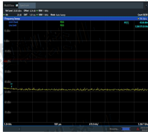
NTVN-11AC20MIMO-Ant2-5180-5260~5266.7-P ASS
