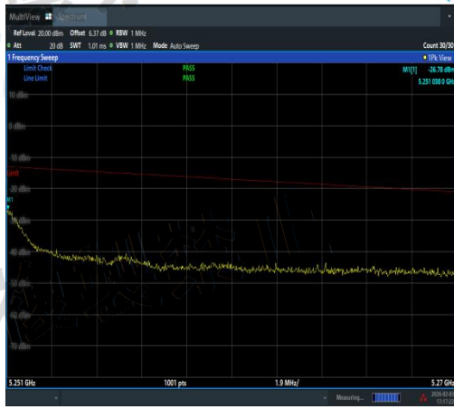
NTNV-11AC40SISO-Ant2-5230-5251~5270-PAS
