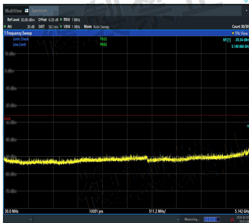
NTNV-11AX20SISO-Ant3-5180-30~5142-PASS
