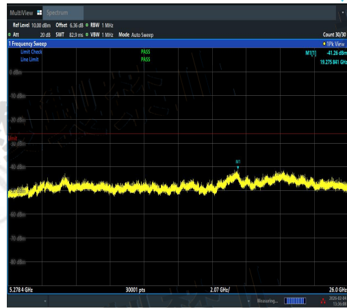
NTVN-11N40MIMO-Ant1-5230-5278.4~26000-P ASS
