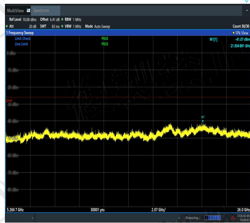
NTVN-11AC20MIMO-Ant3-5220-5266.7~26000- PASS
