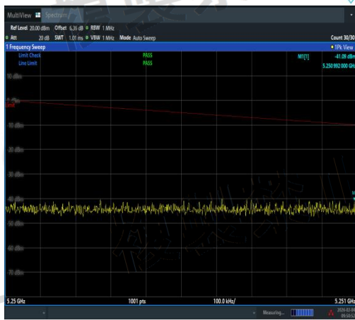
NTNV-11AC20MIMO-Ant1-5220-5250~5251-PAS
