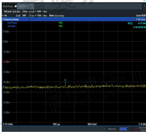
NTNV-11AC40MIMO-Ant2-5190-5141.6~5150-P ASS
