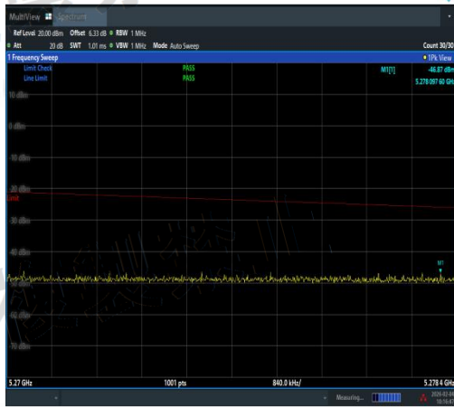
NTNV-11AC40MIMO-Ant1-5190-5270~5278.4-P ASS
