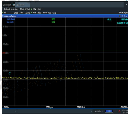
NTVN-11AC20MIMO-Ant1-5180-5260~5266.7-P ASS
