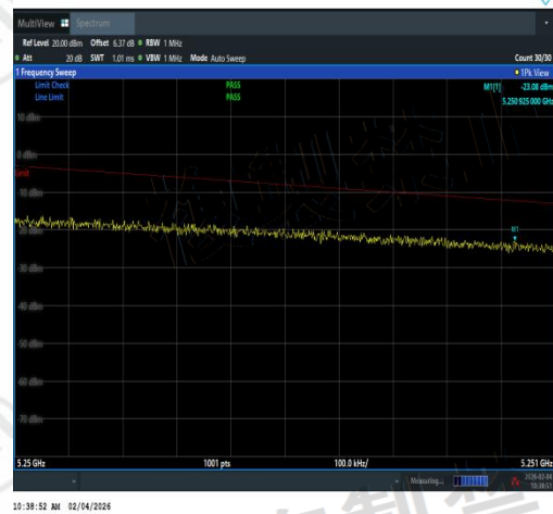
NTVN-11AC40MIMO-Ant2-5230-5250~5251-See table below
