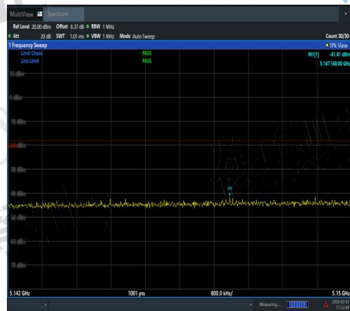
NTVN-11AX20SISO-Ant2-5220-5142~5150-PAS
