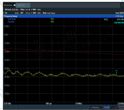
NTNV-11AC80MIMO-Ant3-5210-5251~5290-PAS
