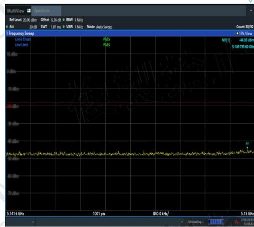
NTVN-11AC40SISO-Ant1-5230-5141.6~5150-PA
