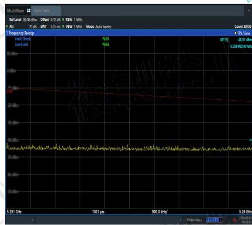
NTNV-11AC20SISO-Ant1-5180-5251~5260-PAS
