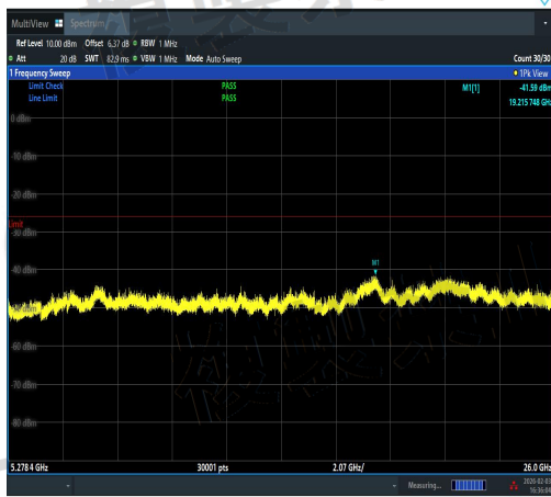
NTNV-11N40SISO-Ant2-5230-5278.4~26000-PA
