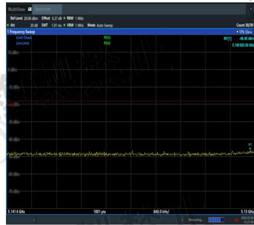
NTVN-11N40MIMO-Ant2-5230-5141.6~5150-PA SS
