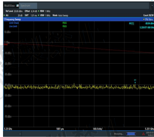
NTNV-11AC20SISO-Ant2-5180-5250~5251-PAS
