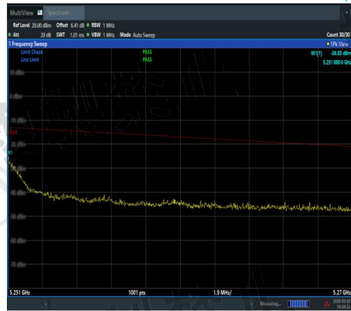
NTNV-11AC40SISO-Ant3-5230-5251~5270-PAS
