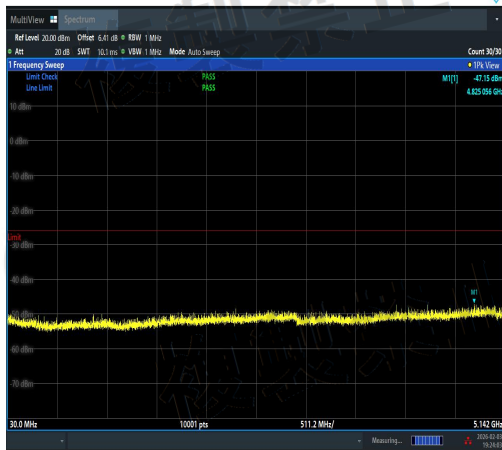
NTNV-11AC20SISO-Ant3-5240-30~5142-PASS
