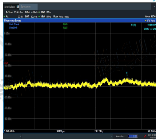
NTNV-11AC40MIMO-Ant1-5190-5278.4~26000-P PASS
