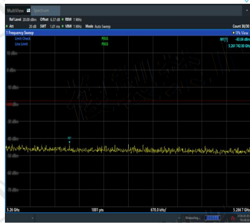
NTNV-11AC20SISO-Ant2-5240-5260~5266.7-PA
