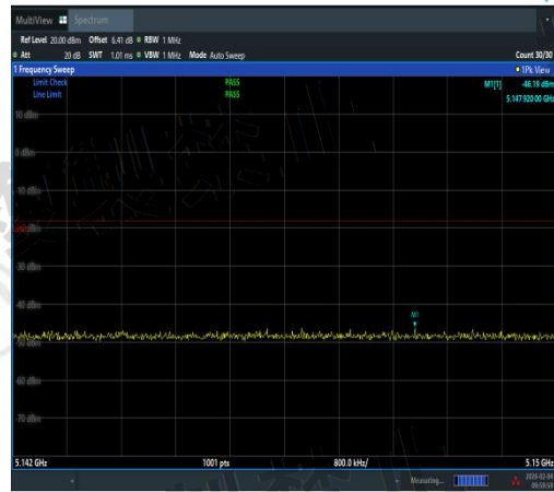
NTNV-11AC20MIMO-Ant3-5220-5142~5150-PAS
