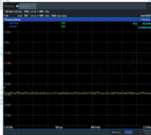
NTNV-11AC20SISO-Ant3-5240-5142~5150-PASS
