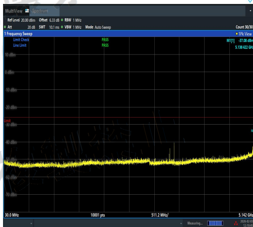
NTNV-11AX20SISO-Ant1-5180-30~5142-PASS
