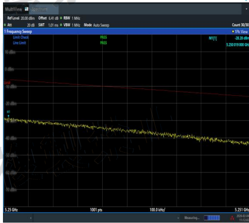
NTNV-11AC80MIMO-Ant3-5210-5250~5251-PAS
