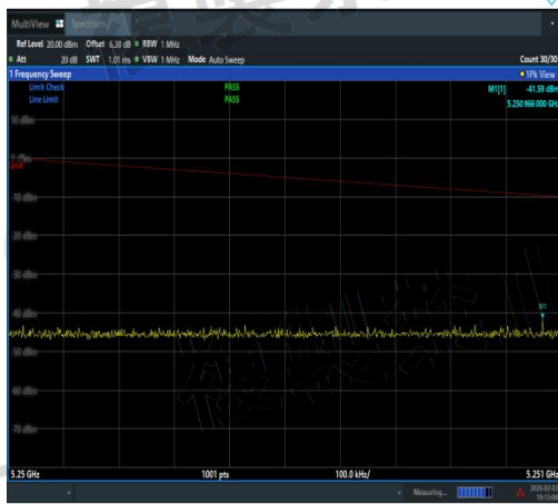
NTNV-11AC20SISO-Ant3-5180-5250~5251-PAS
