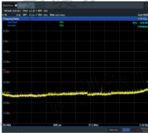
NTNV-11AC20SISO-Ant1-5220-30~5142-PASS
