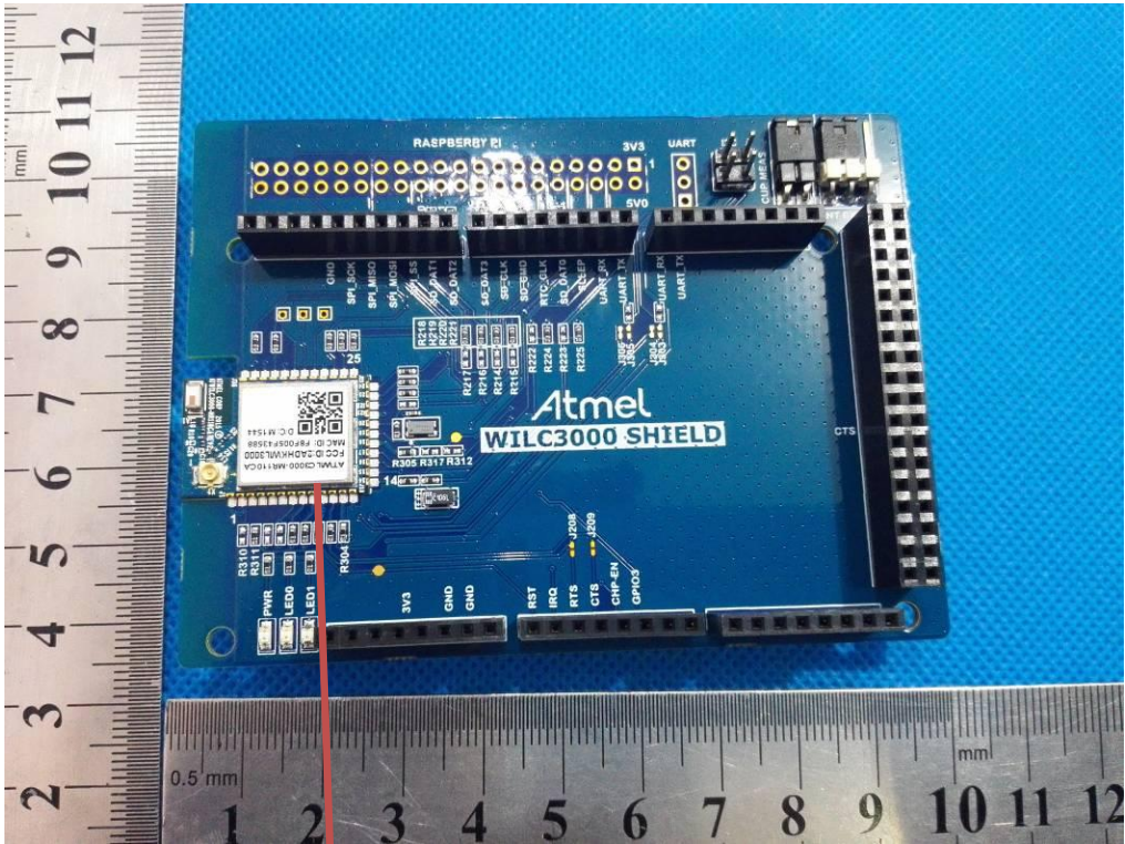
Photo 1: Module appearance
