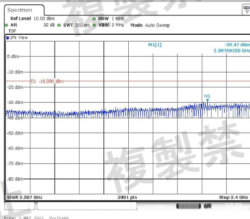
NTNV-11B-Ant1-2412-2387~2400-PASS
