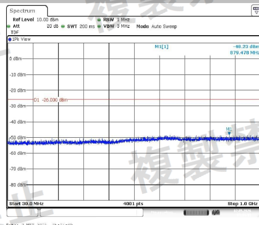
NTNV-11B-Ant1-2442-30~1000-PASS
