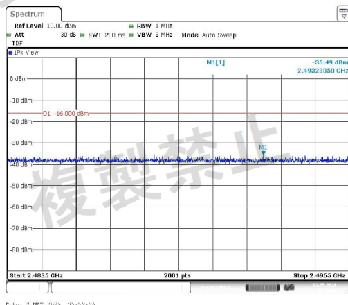
NTNV-11G-Ant1-2412-2483.5~2496.5-PASS
