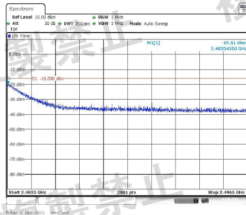
NTNV-11N20SISO-Ant1-2472-2483.5~2496.5-PASS
