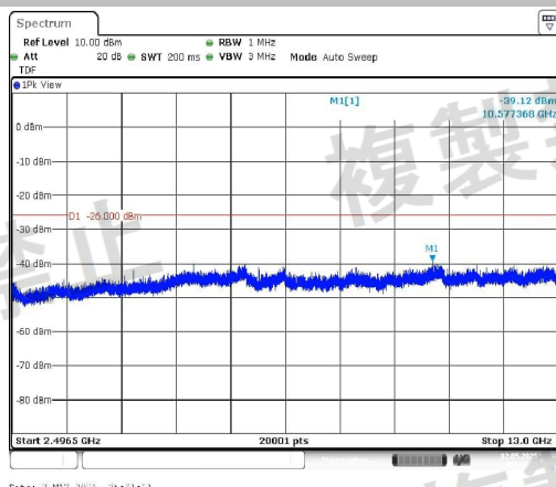
NTNV-11B-Ant1-2412-2496.5~13000-PASS
