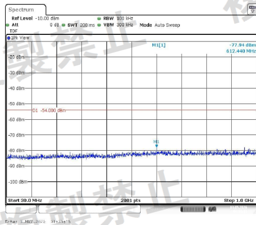
NTNV-11G-Ant1-2442-30~1000-PASS
