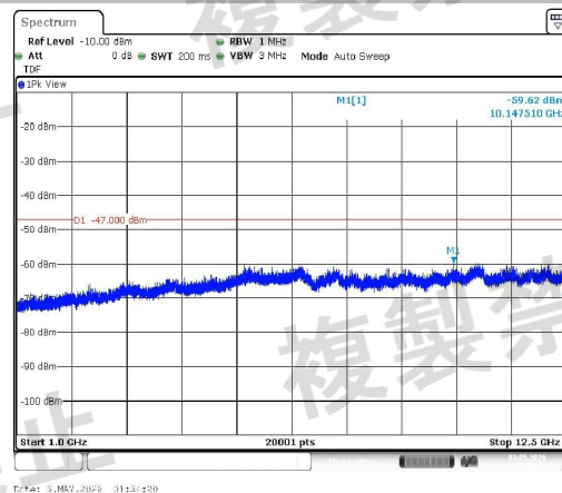
NTVN-11B-Ant1-2472-1000~12500-PASS
