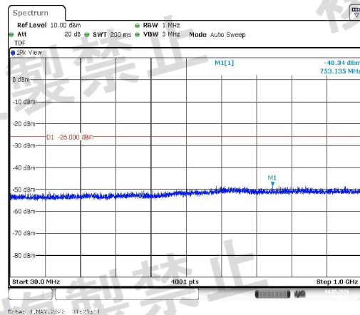
NTNV-11G-Ant1-2472-30~1000-PASS
