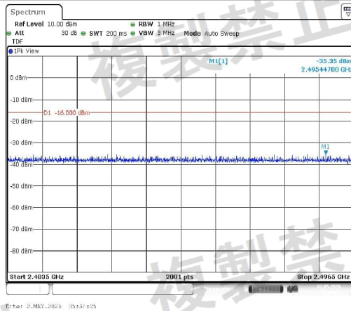
NTNV-11B-Ant1-2442-2483.5~2496.5-PASS
