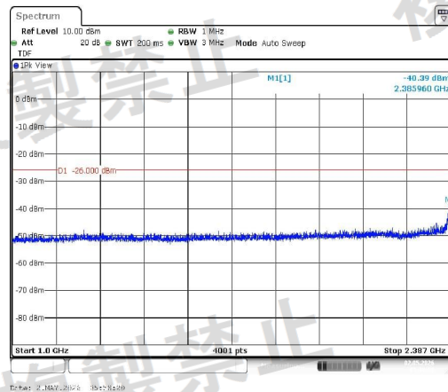
NTNV-11N20SISO-Ant1-2412-1000~2387-PASS
