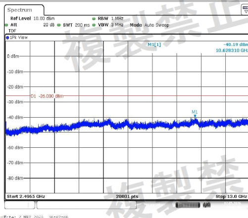
NTNV-11N20SISO-Ant1-2472-2496.5~13000-PASS
