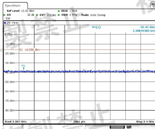
NTNV-11N20SISO-Ant1-2442-2387~2400-PASS
