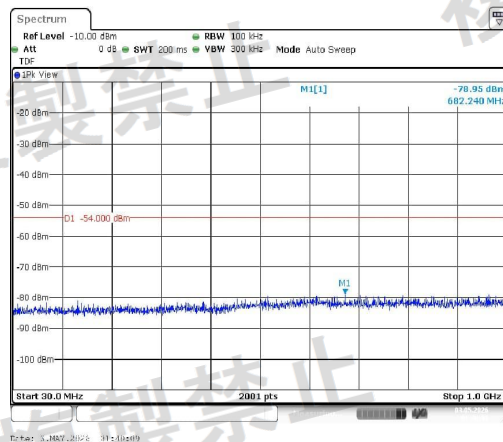
NTNV-11N20SISO-Ant1-2442-30~1000-PASS
