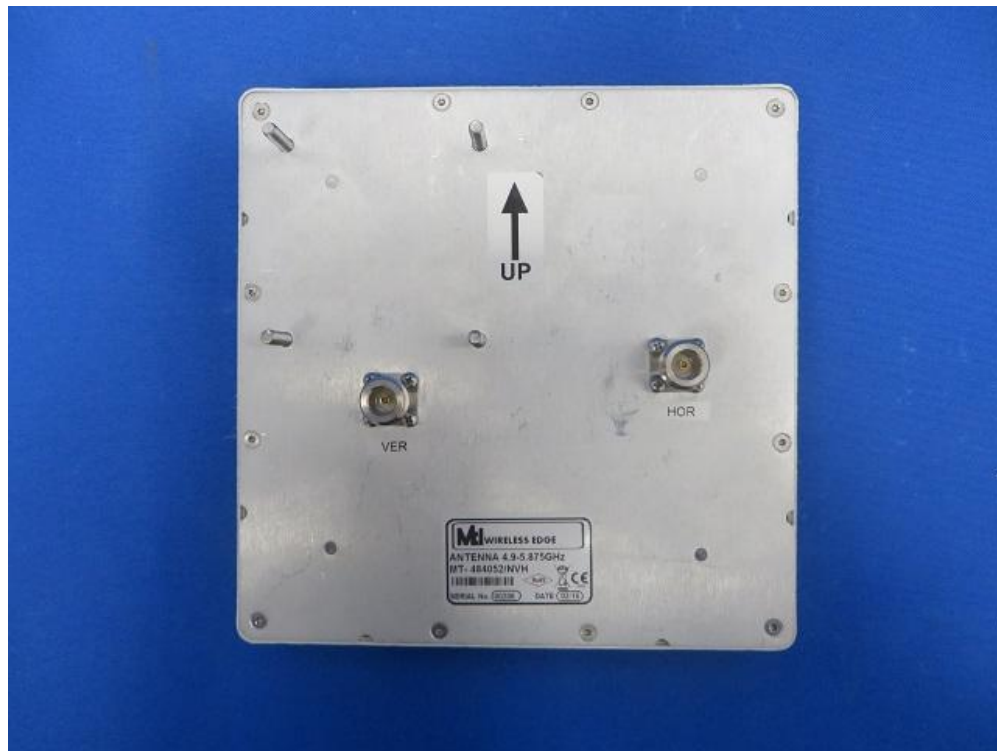
(17) EUT Photo (MT-484052/NVH)
