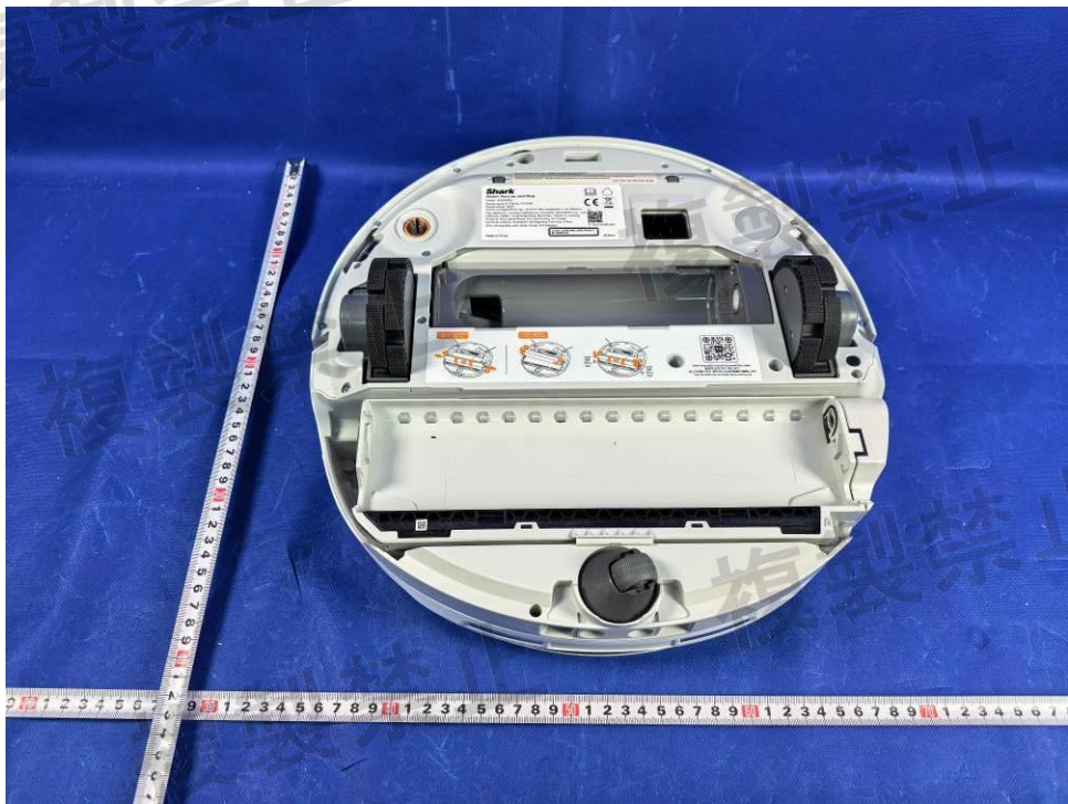
Figure 8. Overall view
