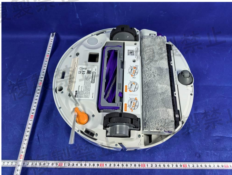
Figure 6. Overall view
