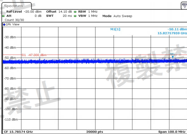
NTNV-11N20-Ant1-5260-1000~26000-PASS
