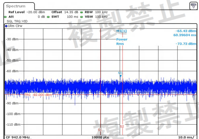
NTNV-11N20-Ant1-5320-30~1000-PASS
