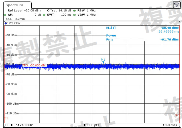
NTNV-11A-Ant2-5300-1000~26000-PASS
