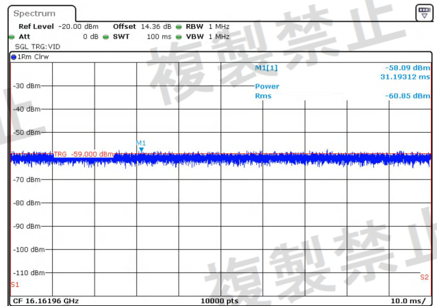
NTNV-11N20-Ant2-5320-1000~26000-PASS
