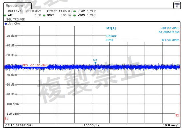
NTNV-11N20MIMO-Ant1-5300-1000~26000-PASS
