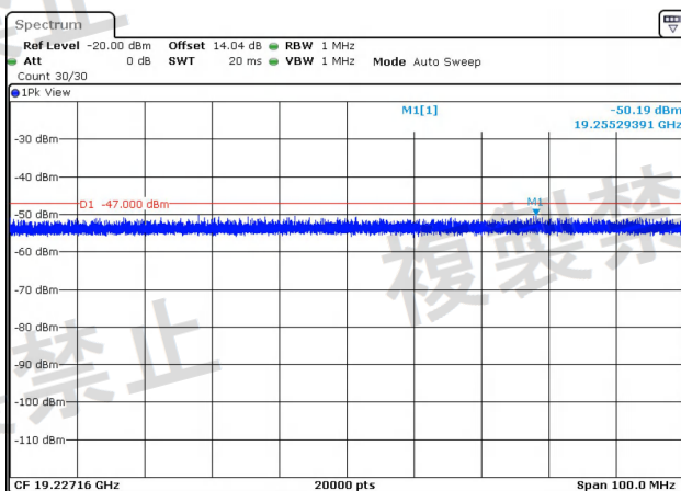
NTNV-11N20MIMO-Ant2-5260-1000~26000-PASS
