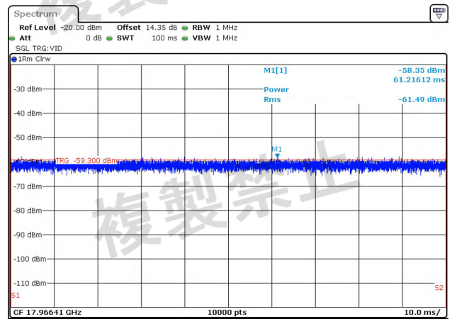
NTNV-11N20-Ant2-5320-1000~26000-PASS
