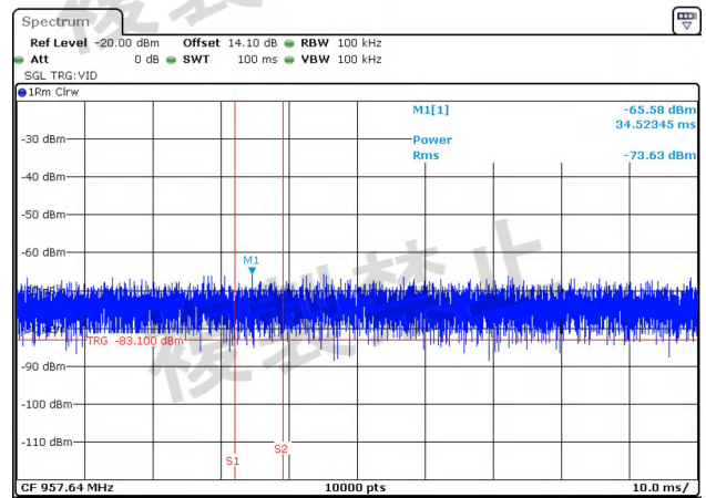
NTNV-11N20-Ant2-5300-30~1000-PASS
