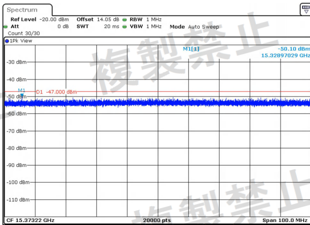
NTNV-11N20MIMO-Ant1-5300-1000~26000-PASS
