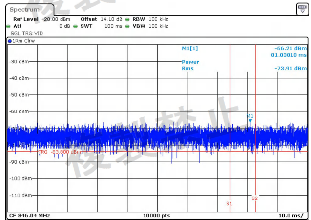
NTNV-11N20MIMO-Ant2-5300-30~1000-PASS
