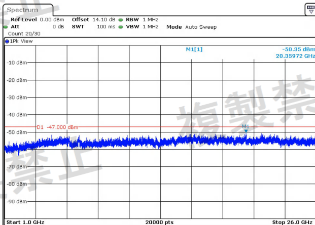
NTNV-11AC40-Ant1-5310-1000~26000-See table below
