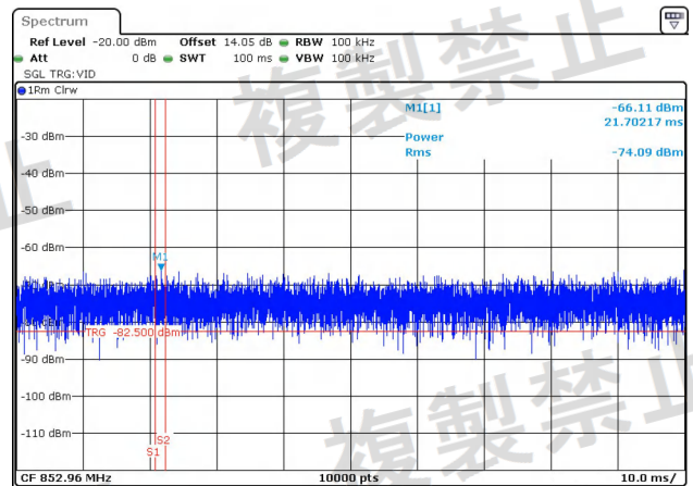
NTNV-11N20-Ant2-5300-30~1000-PASS
