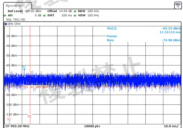
NTNV-11N20MIMO-Ant1-5260-30~1000-PASS
