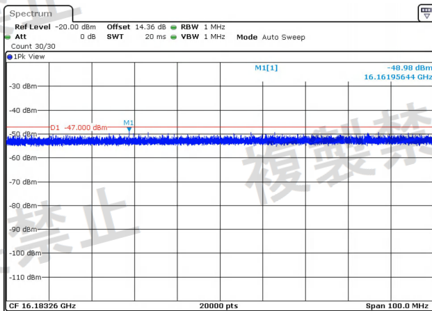
NTNV-11N20-Ant2-5320-1000~26000-PASS
