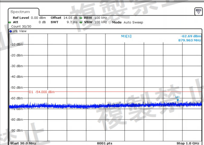
NTNV-11AC40MIMO-Ant2-5310-30~1000-See table below
