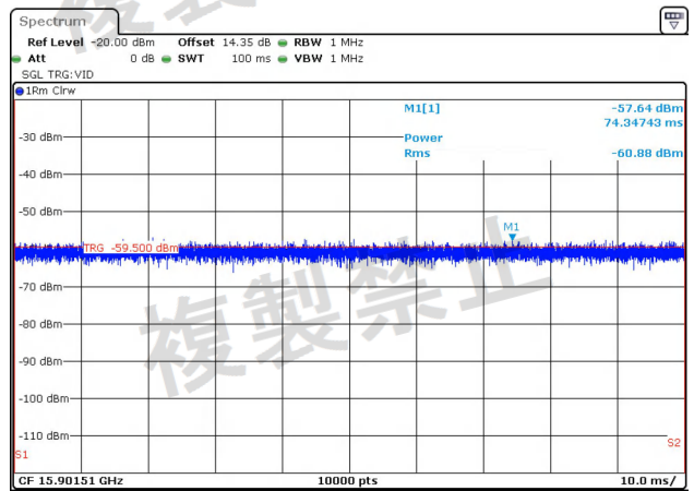
NTNV-11A-Ant2-5320-1000~26000-PASS
