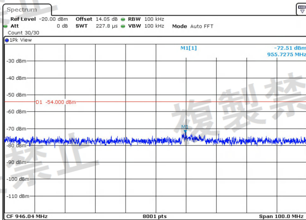
NTNV-11N20MIMO-Ant2-5300-30~1000-PASS
