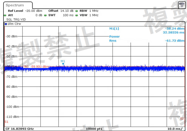
NTNV-11N20-Ant2-5300-1000~26000-PASS
