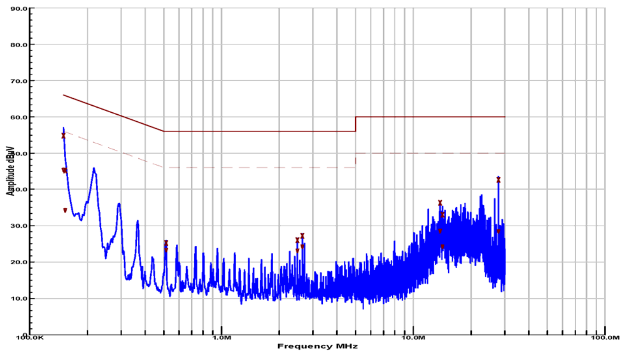
Neutral (中性線)
