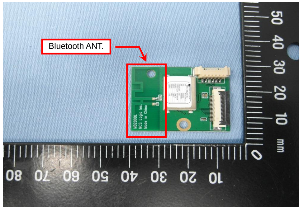
EUT Photo (1)
