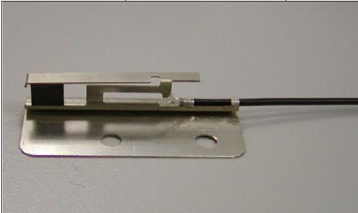
PIFA Antenna (Brand name: WNC, Model No.: 504993-001)
