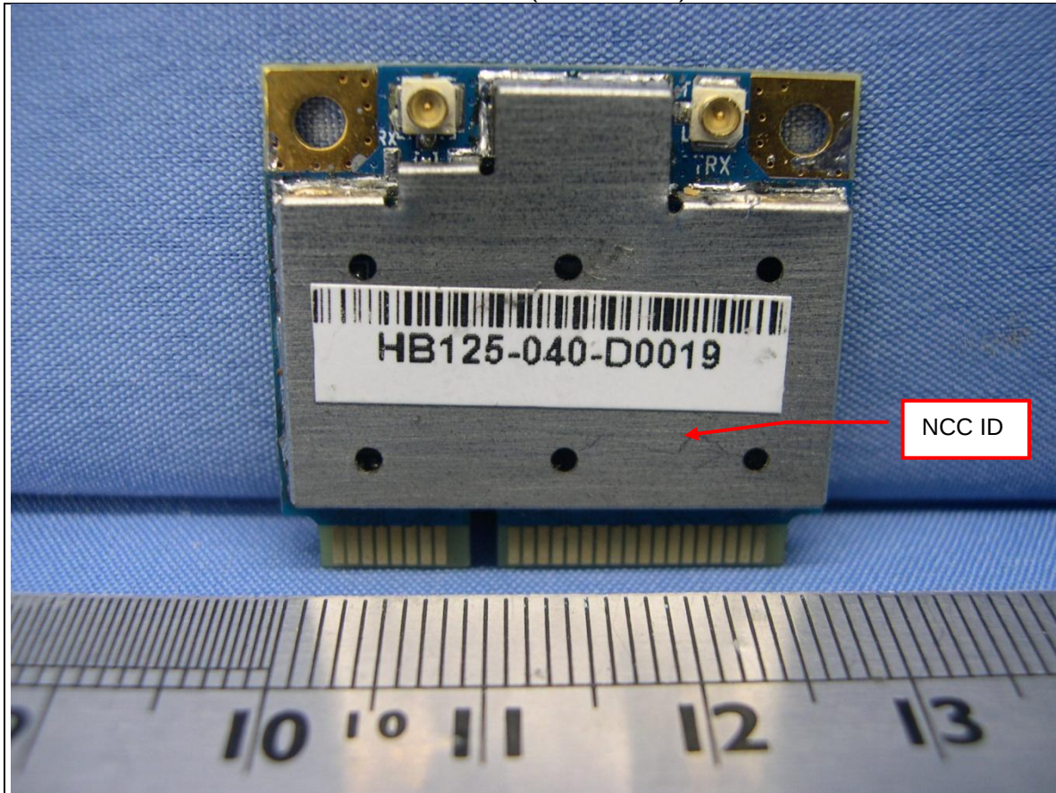
EUT <Version B(Dual antenna)>
