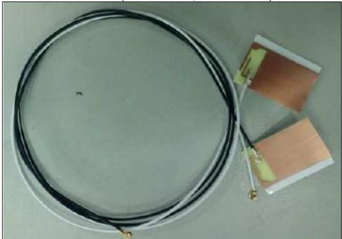
PIFA Antenna (Brand name: ACON, Model No.: ACTA-01)
