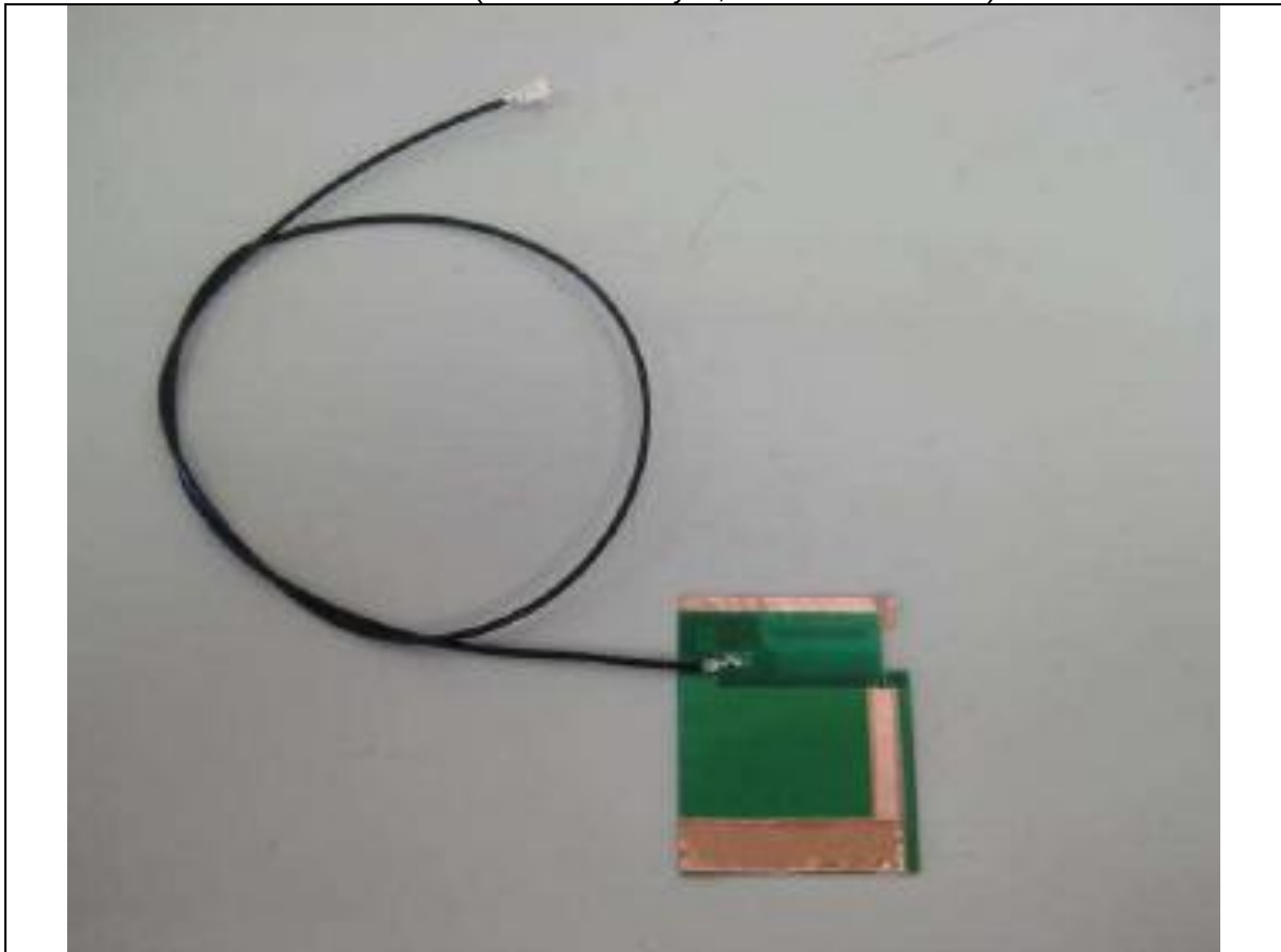
PIFA Antenna (Brand name: Tyco, Model No.: TBN010)
