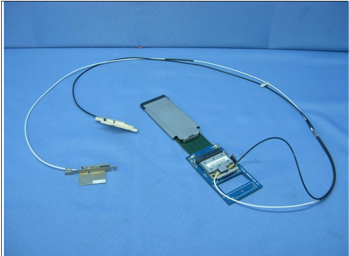
廠牌: AIRETOS, 型號: AEH-AR9485 EUT with PIFA antenna and Test Tool
