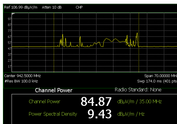
Fig. A3.f 900 MHz band, Average: 84,87 dBμV/m k.o.m. 0,018 V/m
