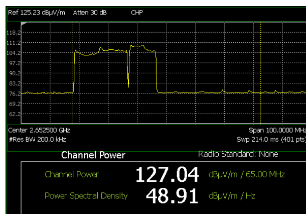
Fig. A3.l 2,6 GHz band, Average: 127,04 dBμV/m k.o.m. 2,25 V/m
