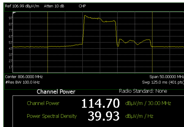
Fig. A3.d 800 MHz band, Average: 114,70 dBμV/m k.o.m. 0,51 V/m
