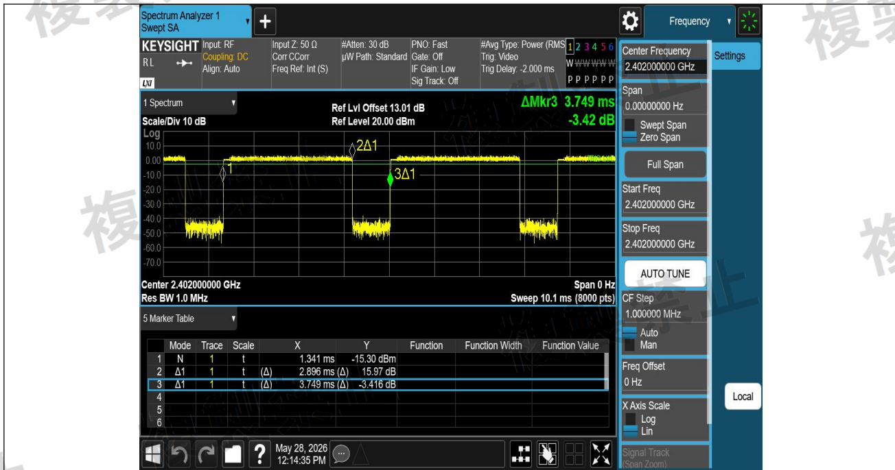
NTNV-3DH5-Ant1-2402
