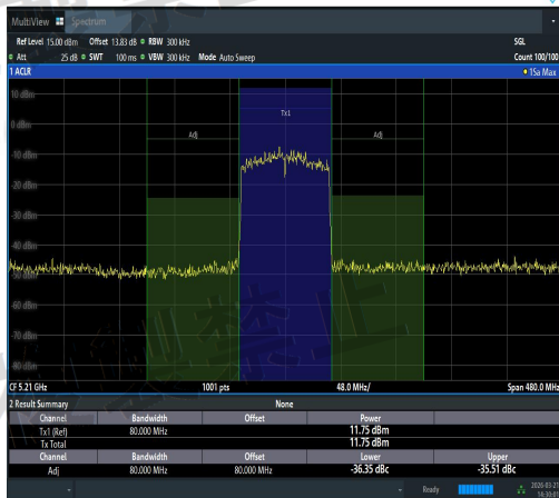
NTVN-11AC80MIMO-Ant1-5210-PASS
