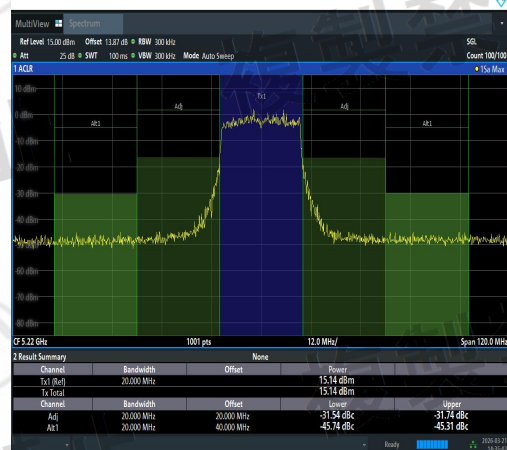
NTVN-11AX20MIMO-Ant3-5220-PASS
