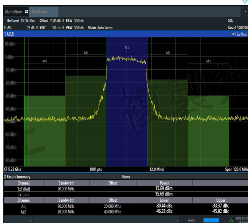
NTVN-11AX20MIMO-Ant2-5220-PASS
