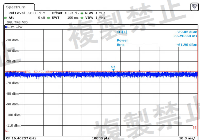
NTNV-11N20-Ant1-5180-1000~26000-PASS
