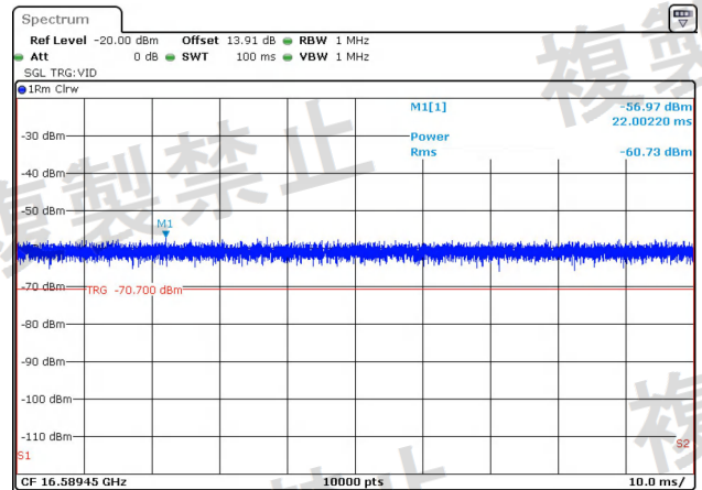
NTNV-11N20MIMO-Ant2-5180-1000~26000-PASS
