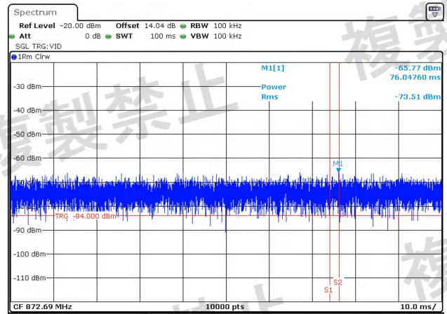
NTNV-11N20MIMO-Ant2-5240-30~1000-PASS
