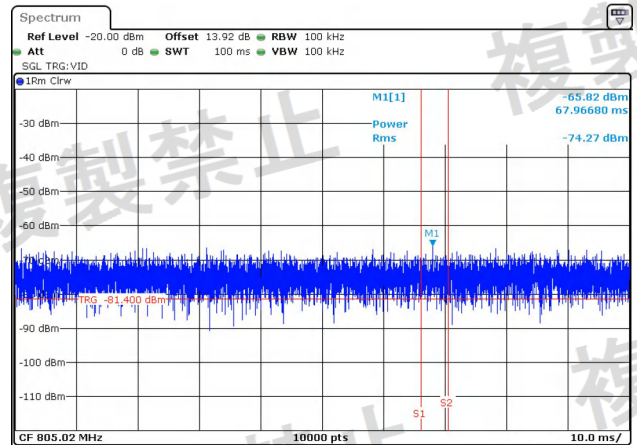
NTNV-11N20MIMO-Ant1-5200-30~1000-PASS
