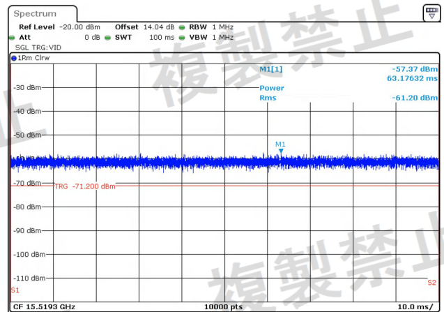
NTNV-11N20MIMO-Ant2-5240-1000~26000-PASS
