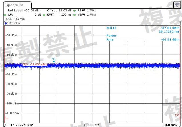
NTNV-11N20-Ant2-5200-1000~26000-PASS
