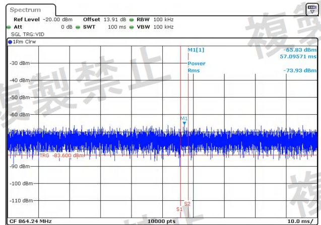
NTNV-11N20-Ant2-5180-30~1000-PASS
