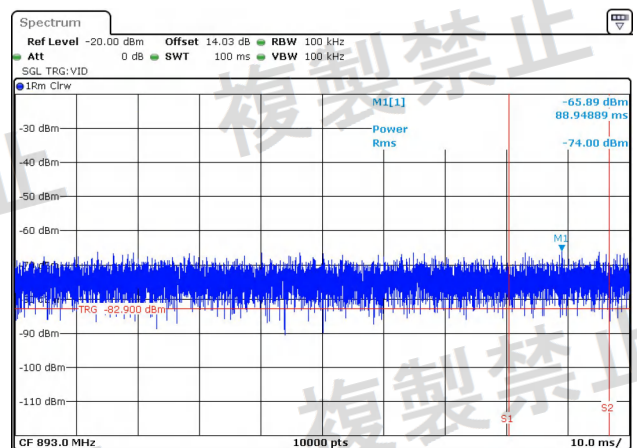
NTNV-11N20MIMO-Ant1-5200-30~1000-PASS
