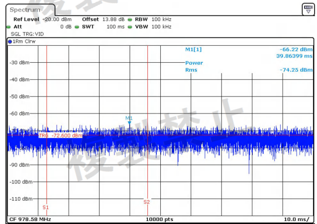
NTNV-11N20MIMO-Ant1-5180-30~1000-PASS
