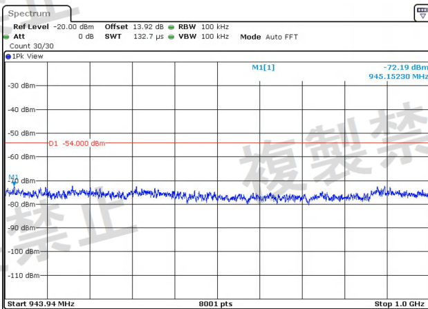
NTNV-11A-Ant2-5200-30~1000-PASS
