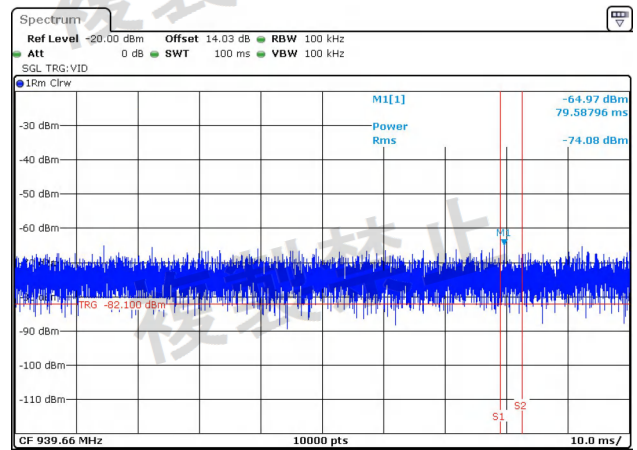
NTNV-11A-Ant2-5200-30~1000-PASS
