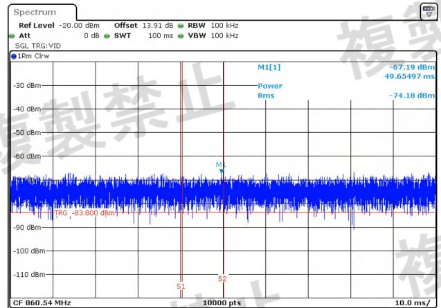
NTNV-11N20MIMO-Ant2-5180-30~1000-PASS
