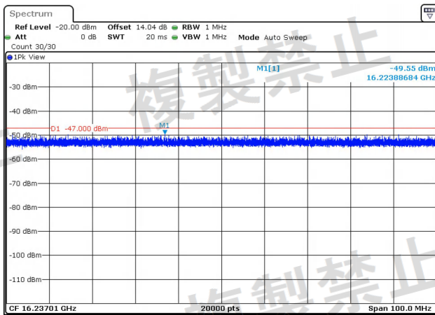
NTNV-11N20-Ant2-5240-1000~26000-PASS
