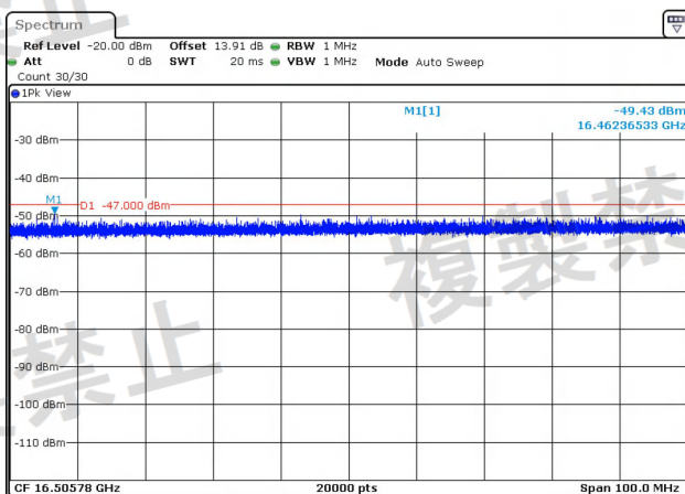
NTNV-11N20-Ant1-5180-1000~26000-PASS
