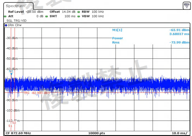
NTNV-11N20MIMO-Ant2-5240-30~1000-PASS
