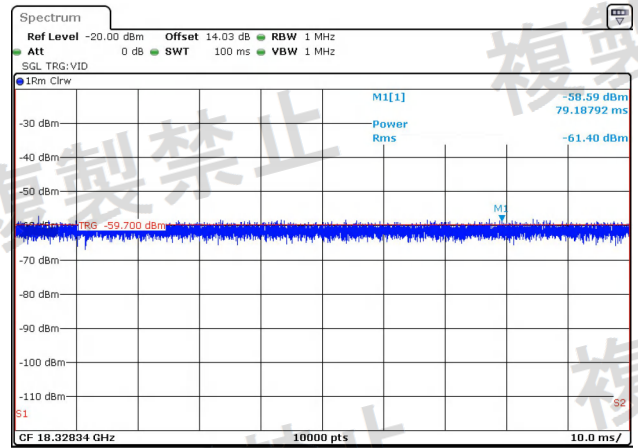
NTNV-11A-Ant2-5200-1000~26000-PASS
