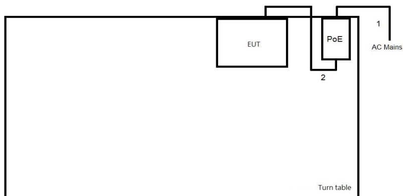
Test Setup Diagram – AC Line Conducted Emission Test – PoE mode - TX
