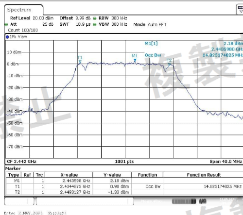
NTVN-11G-Ant1-2442-PASS
