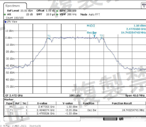
NTVN-11G-Ant1-2472-PASS
