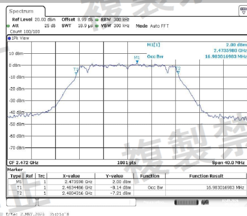
NTVN-11G-Ant1-2472-PASS
