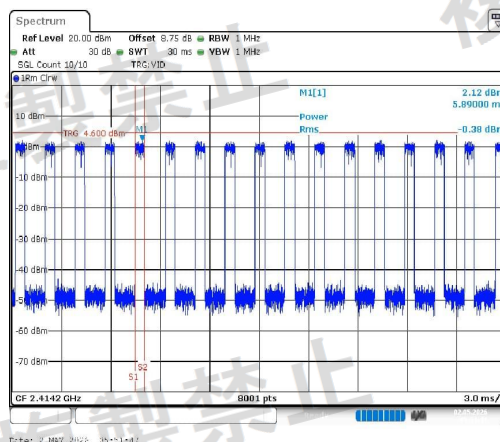
NTNV-11G-Ant1-2412-PASS
