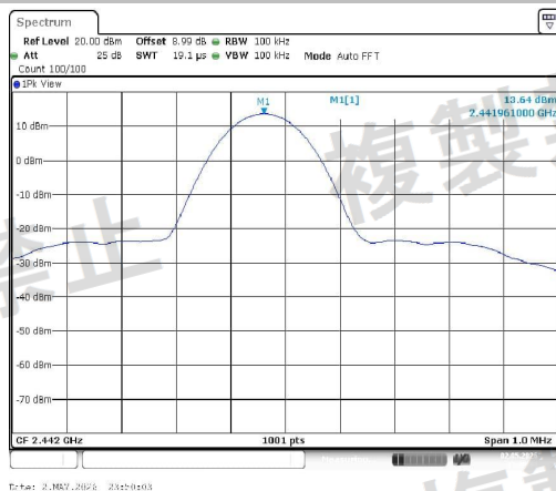
NTVN-11G-Ant1-2442-PASS
