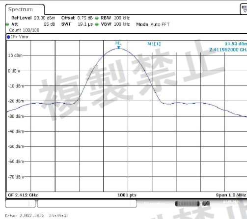
NTVN-11G-Ant1-2412-PASS
