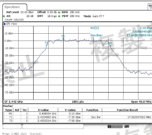
NTVN-11G-Ant1-2442-PASS
