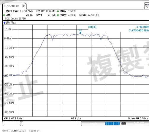
NTNV-11N20SISO-Ant1-2472-PASS
