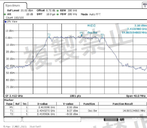
NTVN-11G-Ant1-2412-PASS
