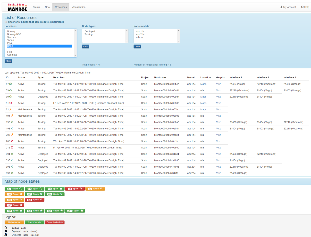
Figure 14: Status of the MONROE nodes. The screen capture shows all types of nodes in Spain. The green approval sign (“thumbs-up”) close to the node IDs indicates that this node is capable of executing experiments. Clicking on the “Location” link for a node opens a Google Maps page showing the location of the node. Finally, the bottom part of the screen shows a “map” of nodes that allows users and MONROE administrators to quickly identify available (and problematic) nodes in the platform.
