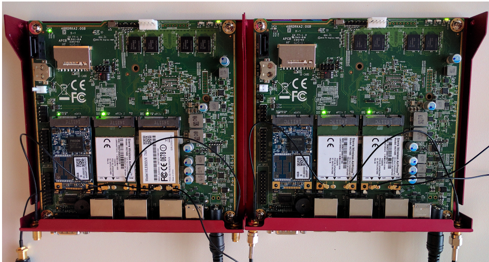
Figure 1: System design. Left: Tail node with one LTE Cat6 modem and one WiFi adaptor. Right: Head node with two LTE Cat6 modems.
