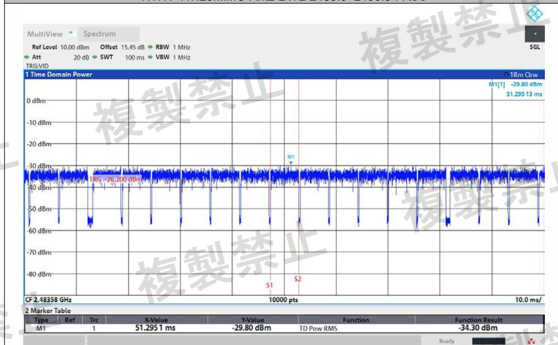
NTNV-11N20MIMO-Ant2-2472-2483.5~2496.5-PASS
