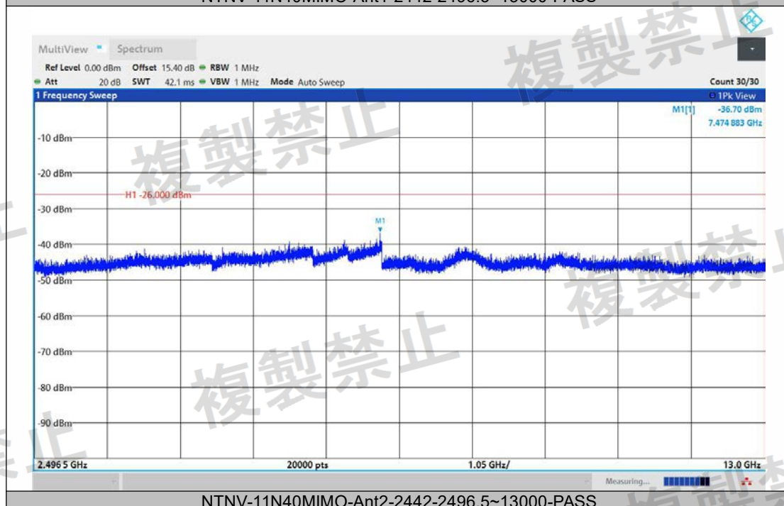
NTNV-11N40MIMO-Ant2-2442-2496.5~13000-PASS
