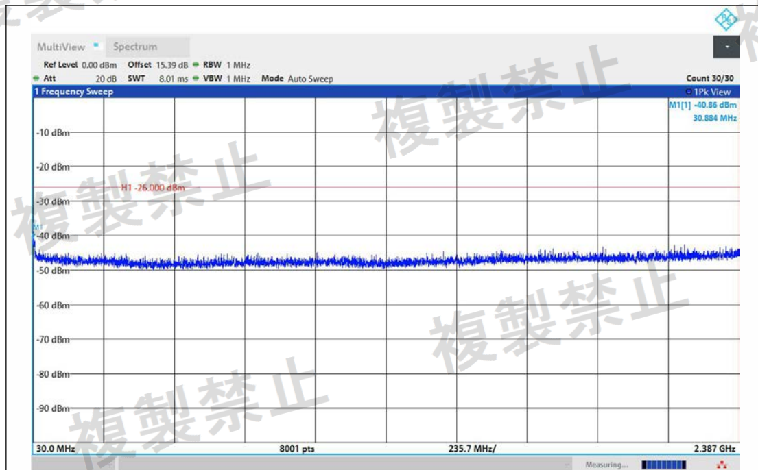
NTNV-11N40MIMO-Ant1-2442-30~2387-PASS
