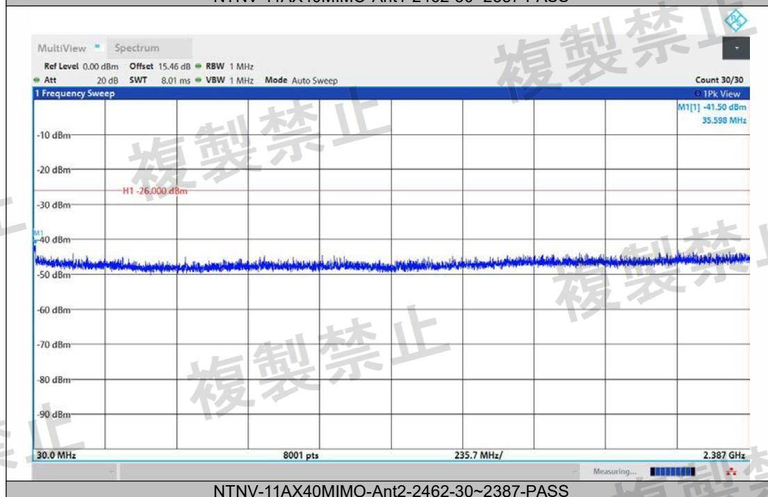
NTVN-11AX40MIMO-Ant2-2462-30~2387-PASS
