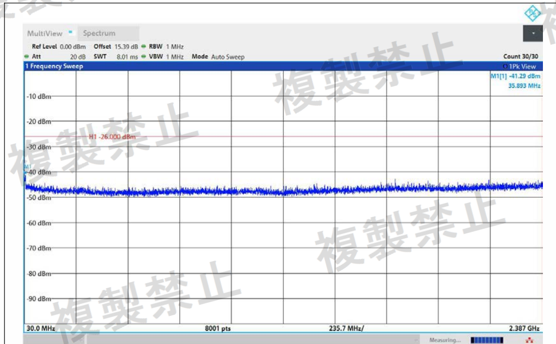
NTNV-11AX20MIMO-Ant1-2442-30~2387-PASS
