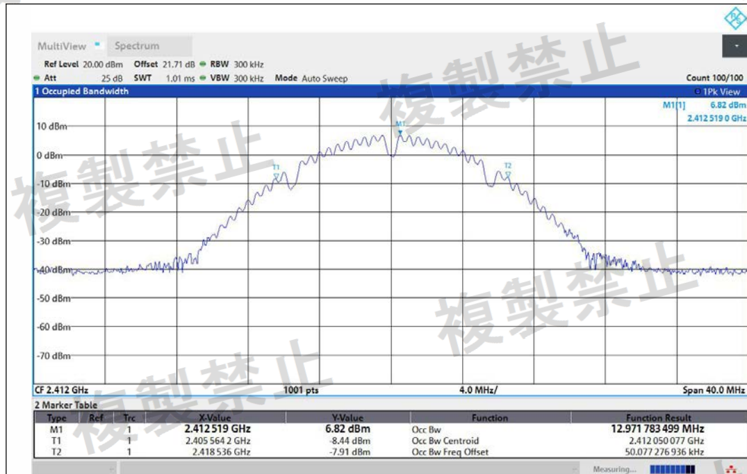
NTNV-11B-Ant1-2412-PASS
