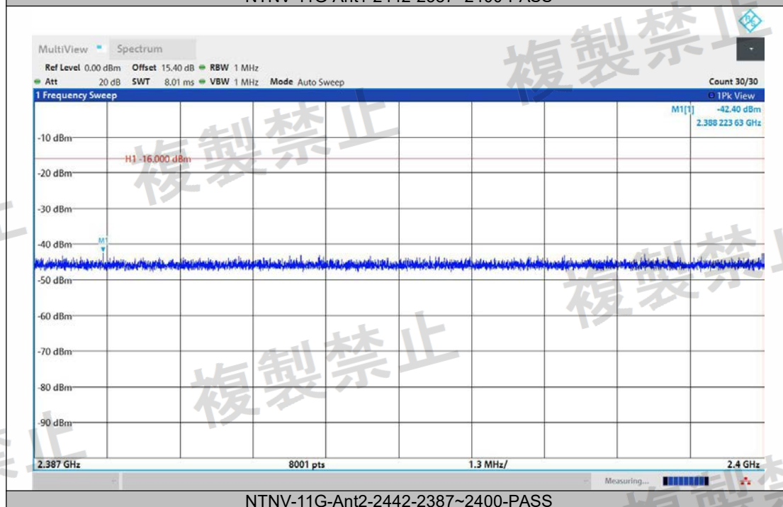
NTNV-11G-Ant2-2442-2387~2400-PASS
