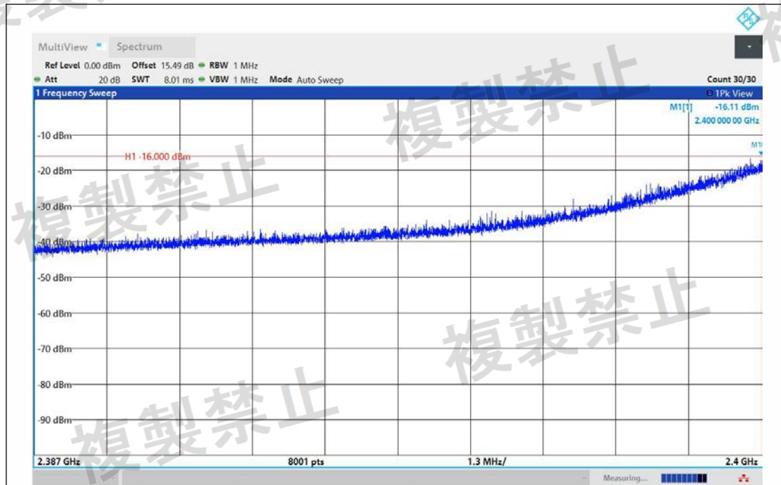
NTNV-11AX20MIMO-Ant1-2412-2387~2400-See table below
