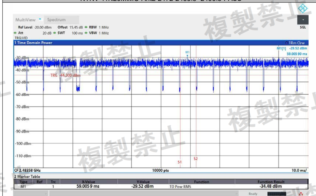
NTNV-11N20MIMO-Ant2-2472-2483.5~2496.5-PASS
