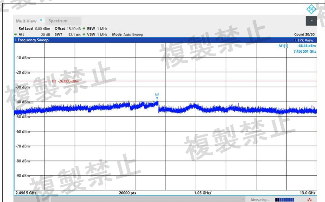
NTNV-11B-Ant1-2412-2496.5~13000-PASS
