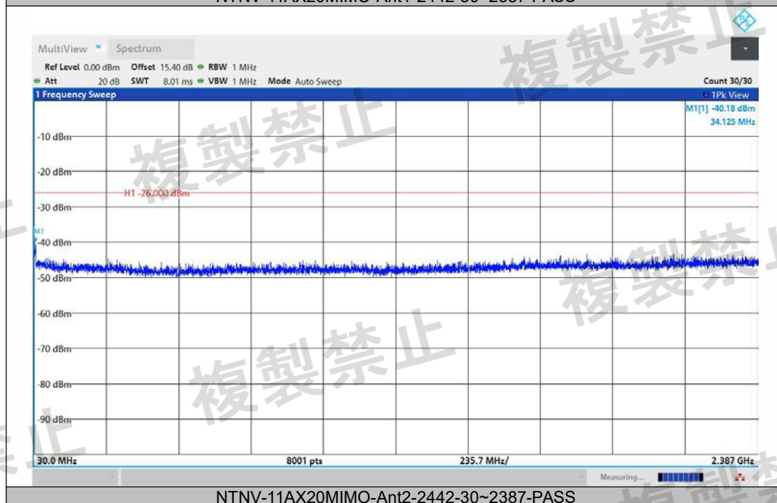
NTNV-11AX20MIMO-Ant2-2442-30~2387-PASS
