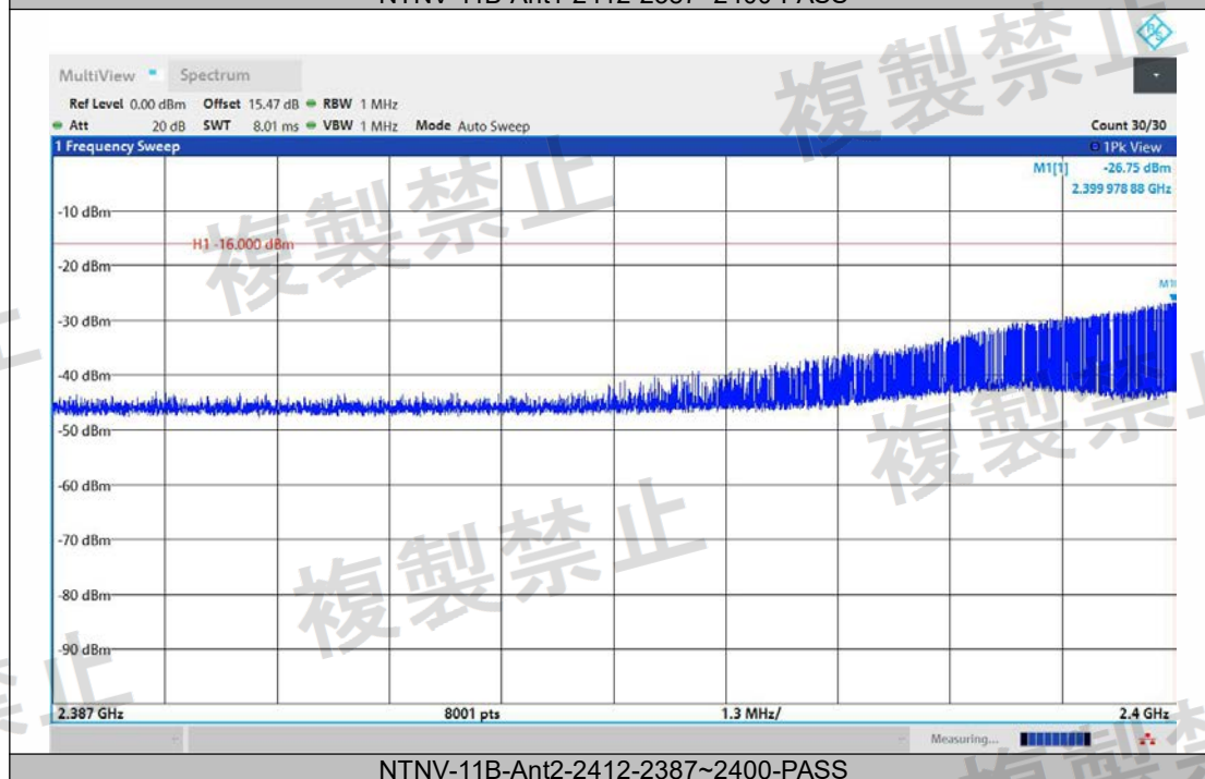
NTNV-11B-Ant2-2412-2387~2400-PASS
