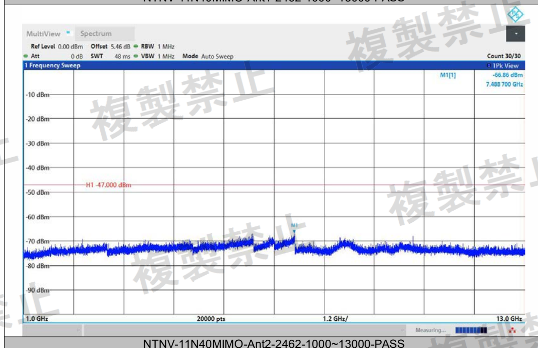
NTNV-11N40MIMO-Ant2-2462-1000~13000-PASS
