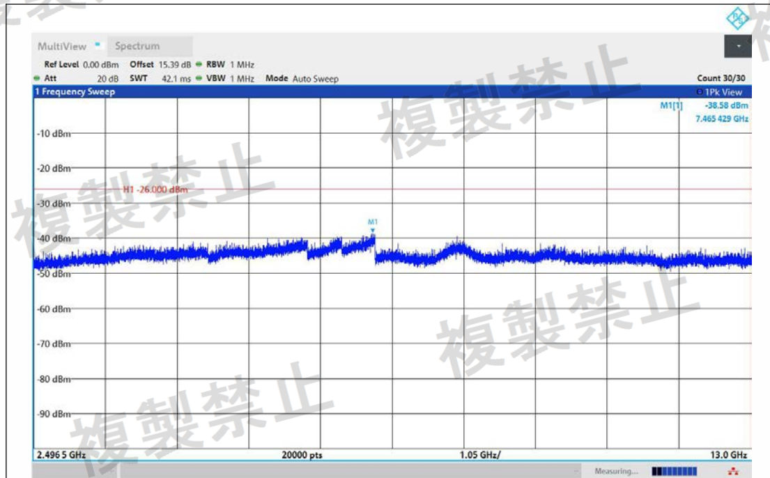
NTNV-11B-Ant1-2442-2496.5~13000-PASS
