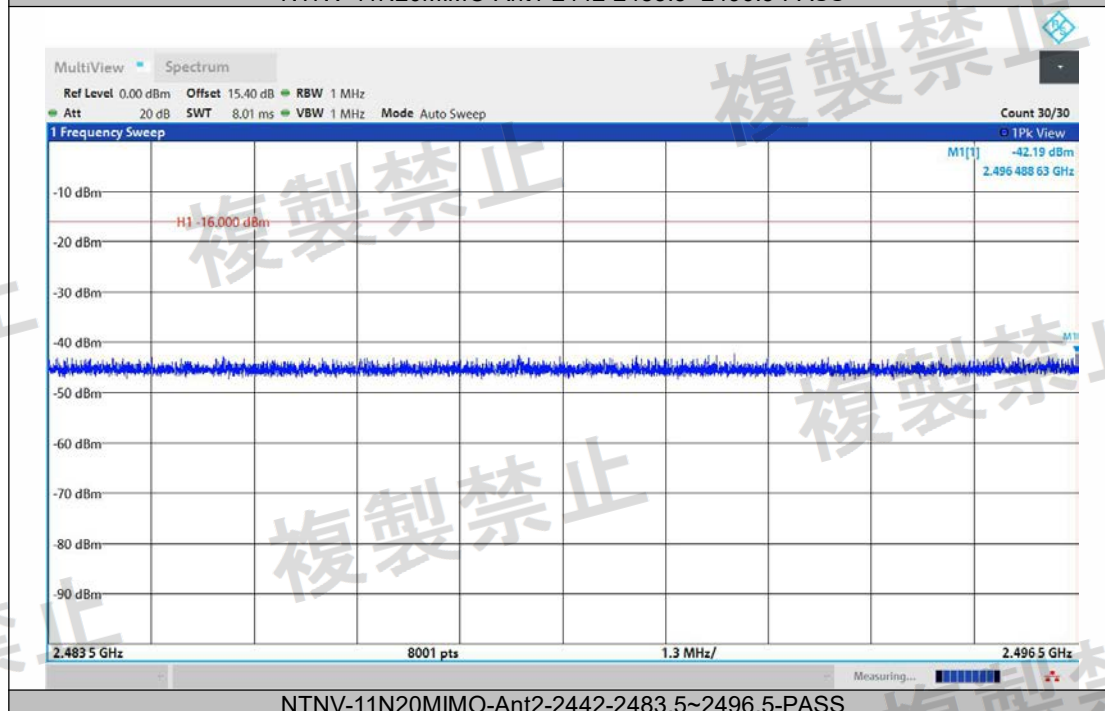
NTNV-11N20MIMO-Ant2-2442-2483.5~2496.5-PASS
