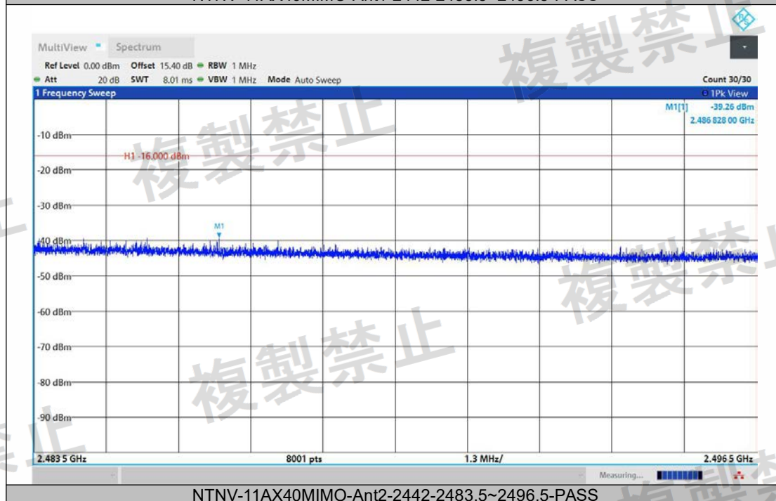
NTNV-11AX40MIMO-Ant2-2442-2483.5~2496.5-PASS
