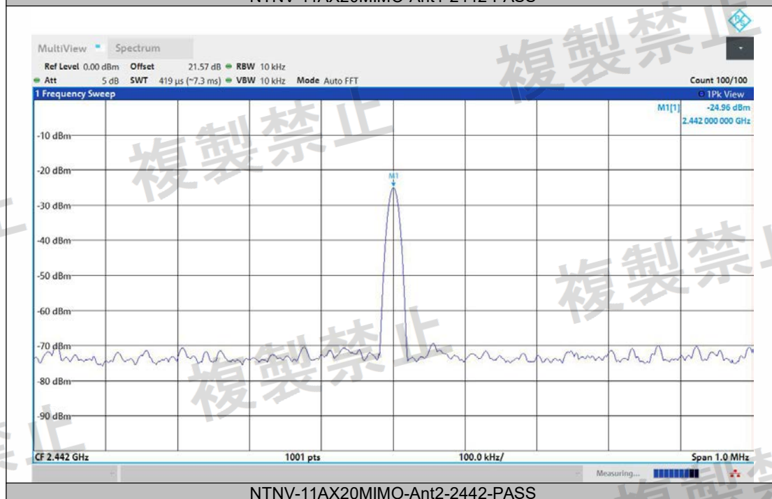
NTNV-11AX20MIMO-Ant2-2442-PASS
