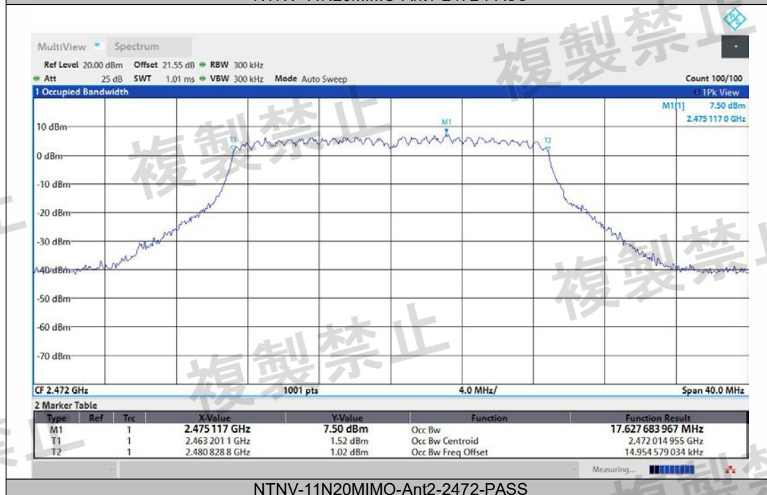
NTNV-11N20MIMO-Ant2-2472-PASS
