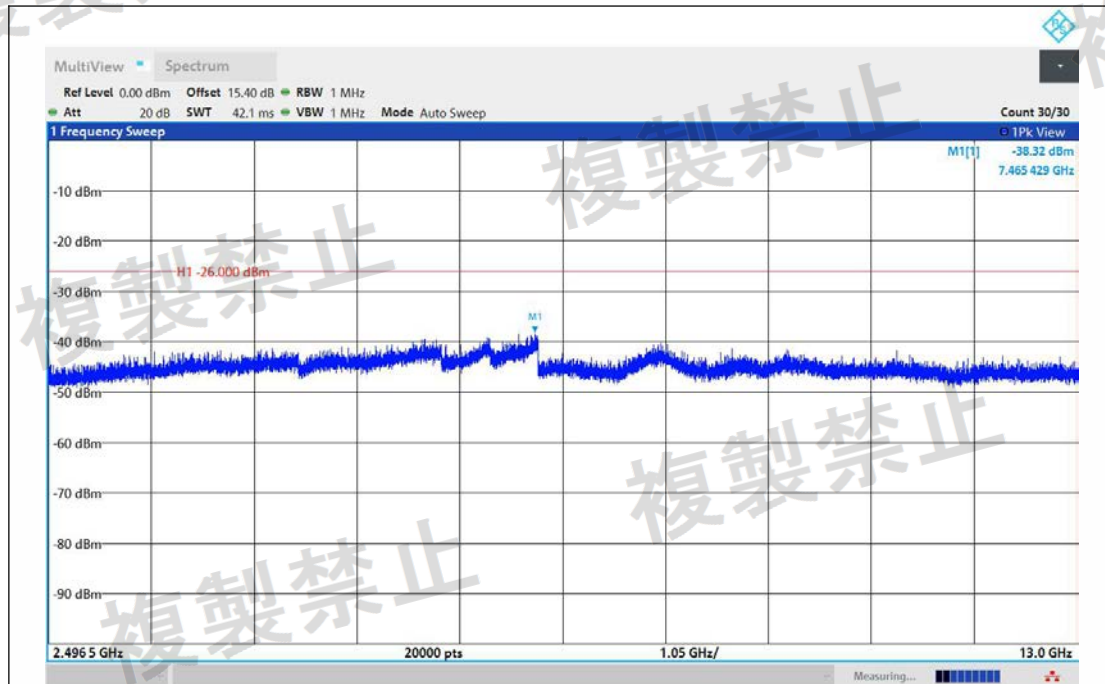
NTNV-11AX40MIMO-Ant1-2422-2496.5~13000-PASS
