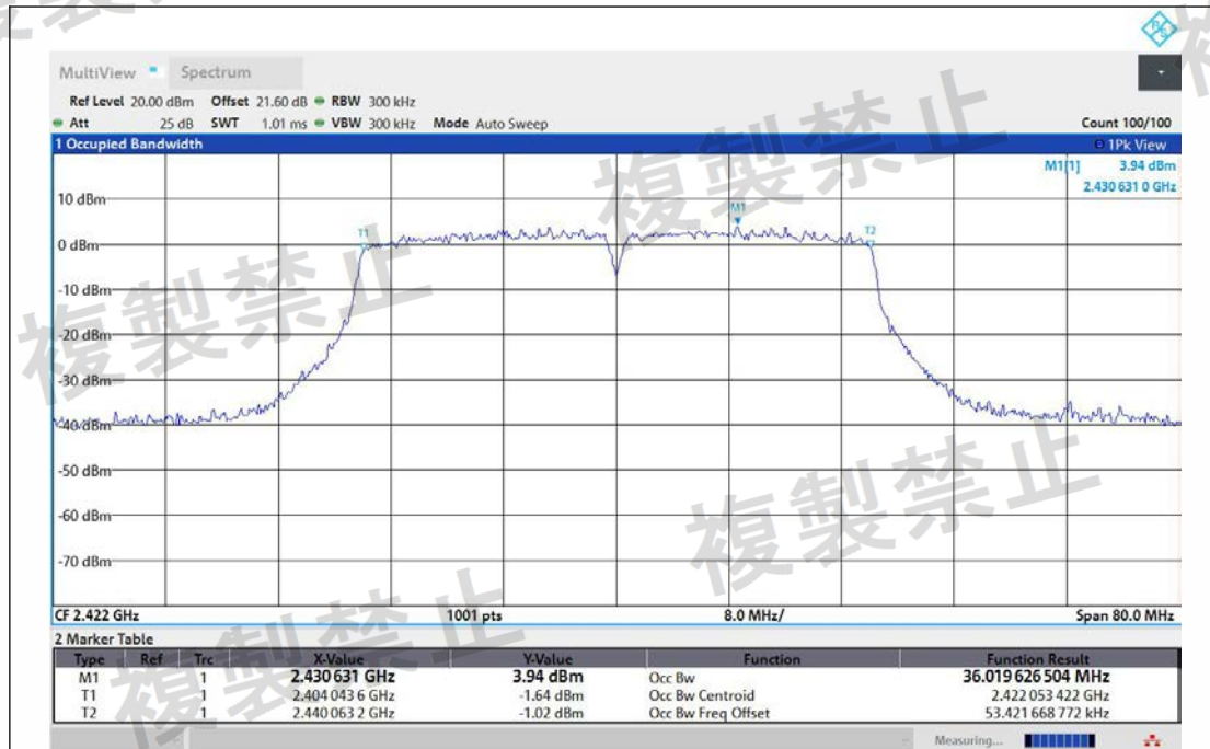
NTNV-11N40MIMO-Ant1-2422-PASS
