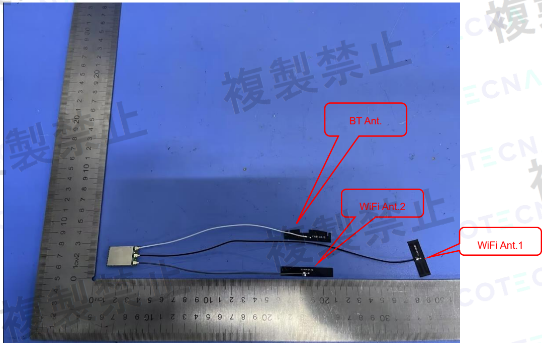
Photo 2 Appearance of EUT with Antenna(XINGHE)
