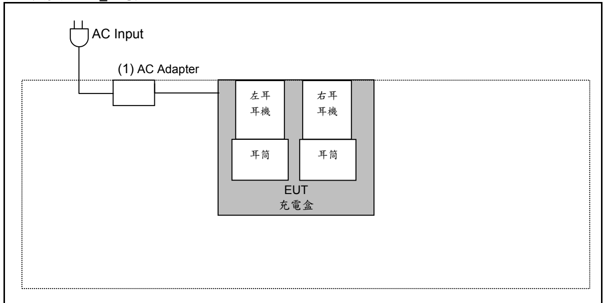
輻射干擾測試配置_充電盒 Below 1 GHz
