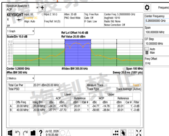
W53 802.11n 20MHz Chain0 Combine
