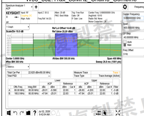
W56 802.11ax 80MHz Chain0 Combine
