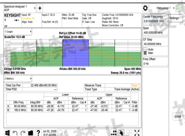
W56 802.11ax 80MHz Chain0 Combine
