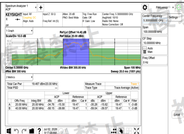
W53 802.11n 20MHz Chain0 Combine
