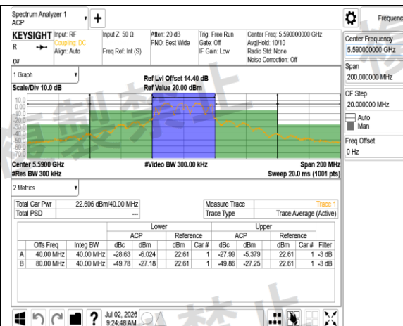
W56 802.11n 40MHz Chain0 Combine
