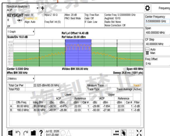
W56 802.11ax 80MHz Chain0 Combine
