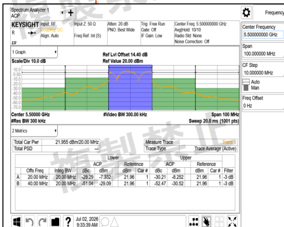
W56 802.11ax 20MHz Chain0 Combine
