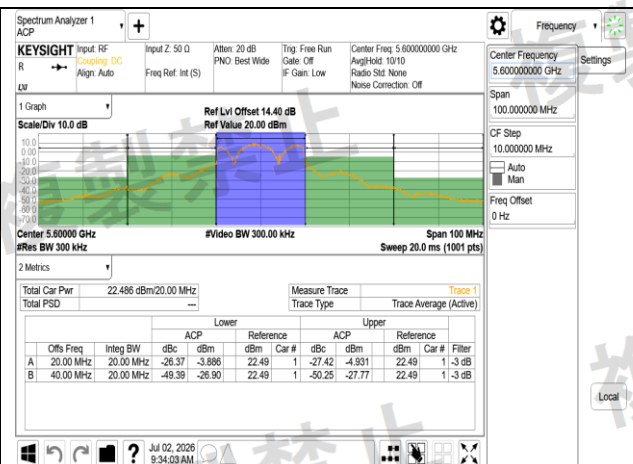
W56 802.11ax 20MHz Chain0 Combine
