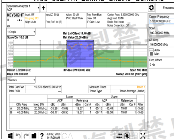
W53 802.11n 20MHz Chain0 Combine
