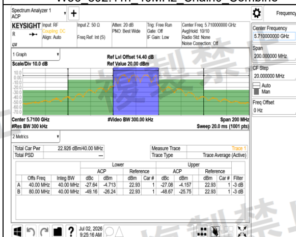
W56 802.11n 40MHz Chain0 Combine
