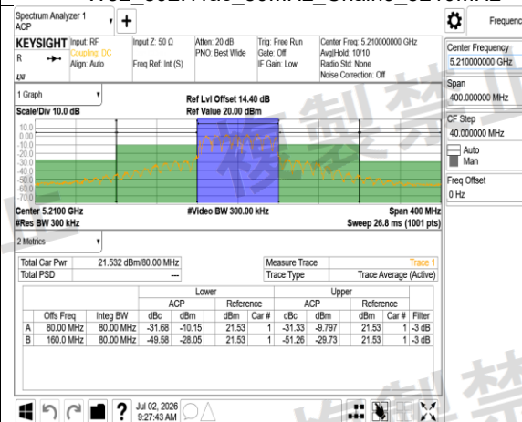
W52 802.11ac 80MHz Chain0 Combine
