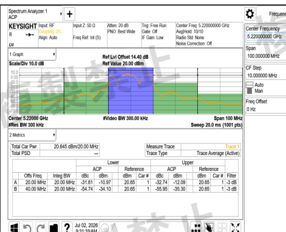
W52 802.11ax 20MHz Chain0 Combine
