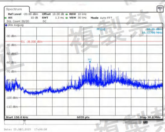
0.15-30.0_new Band 3 15MHz/1747.5/Mid QPSK 30@37
