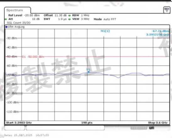
3590.3-3600.0_new Band 3 15MHz/1747.5/Mid QPSK 30@8
