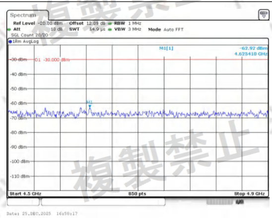
4500.0-4900.0_new Band 3 15MHz/1747.5/Mid QPSK 30@8
