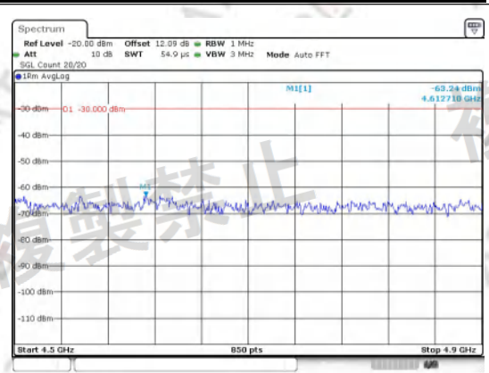
4500.0-4900.0_new Band 3 15MHz/1717.5/Low QPSK 30@0
