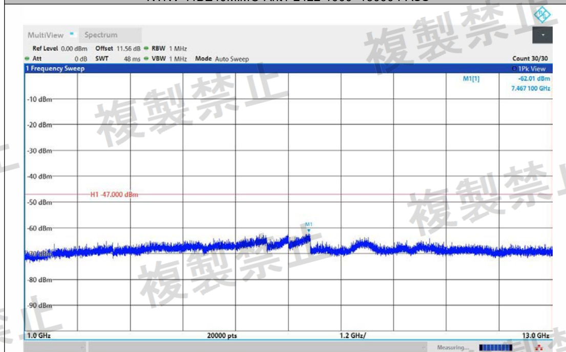
NTNV-11BE40MIMO-Ant2-2422-1000~13000-PASS
