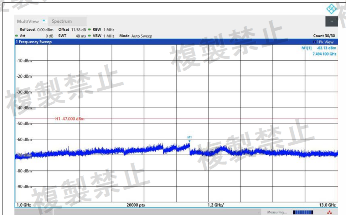
NTVN-11G-Ant1-2472-1000~13000-PASS
