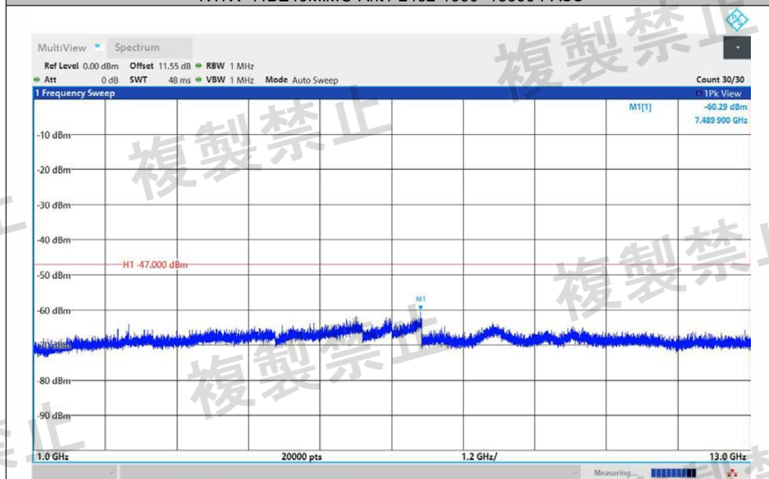
NTNV-11BE40MIMO-Ant2-2462-1000~13000-PASS
