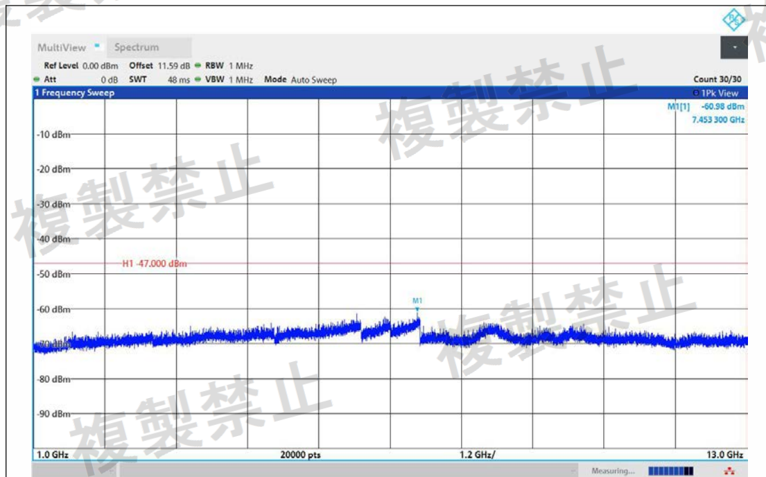
NTVN-11G-Ant1-2442-1000~13000-PASS
