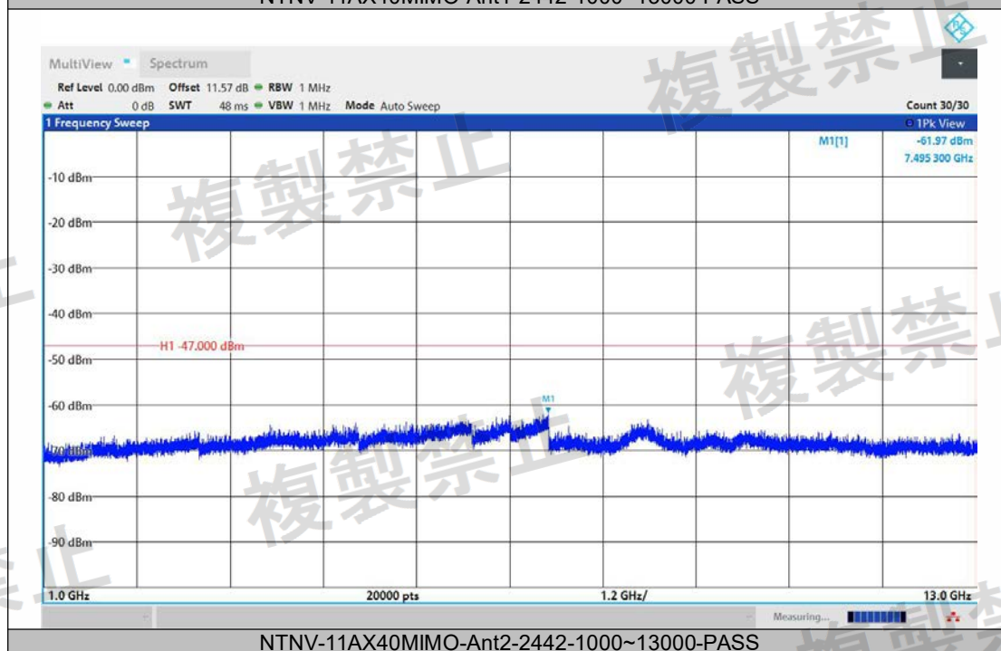
NTNV-11AX40MIMO-Ant1-2442-1000~13000-PASS
