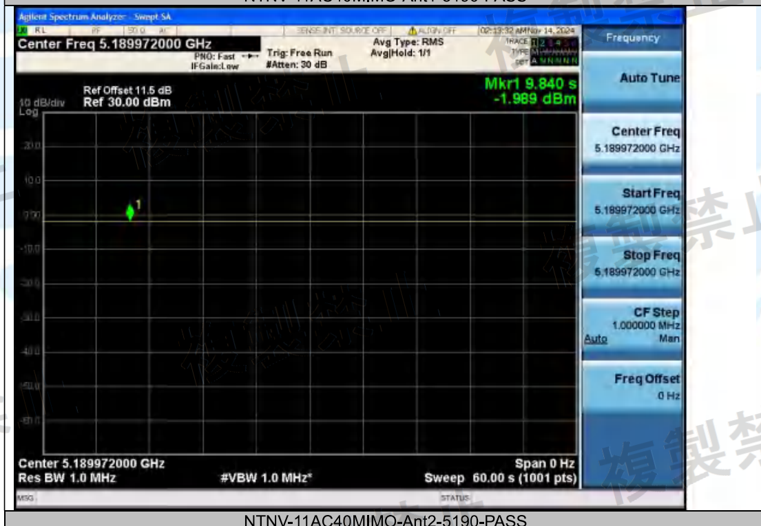
NTNV-11AC40MIMO-Ant2-5190-PASS
