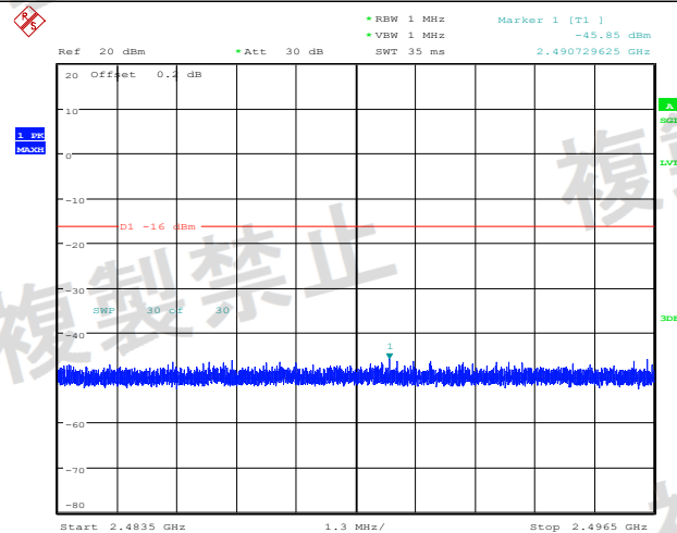
NTNV_11B_Ant1_2412_2483.5~2496.5
