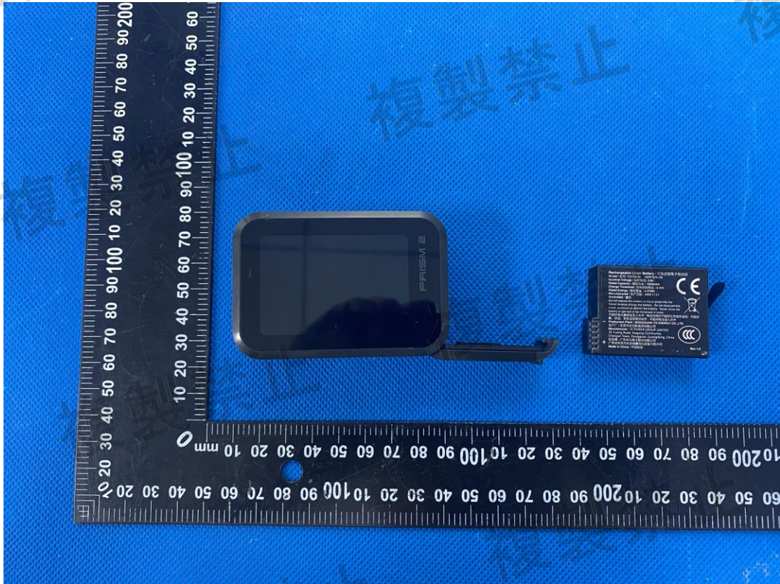
Photo 2 -Camera
