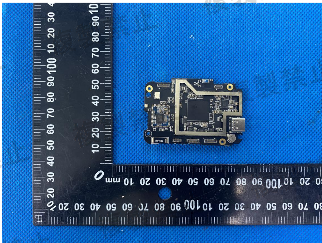
Photo 6 -Camera
