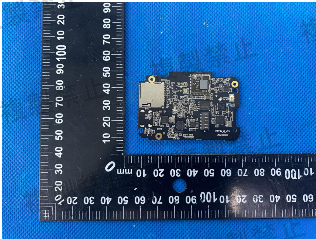
Photo 8 -Camera
