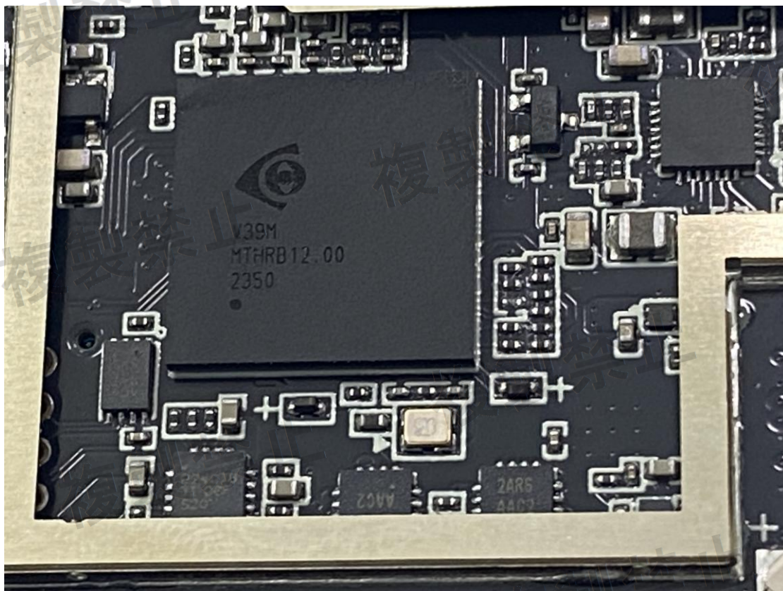
Photo 10 -Camera
