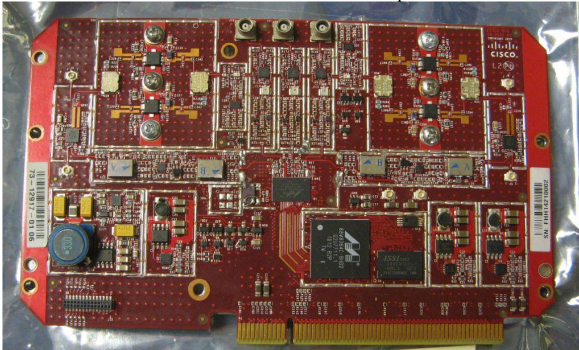
2.4GHz Radio Module Unshielded Bottom
