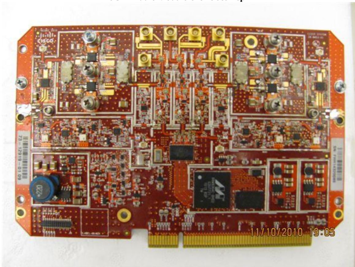
5GHz Radio Module Unshielded Bottom
