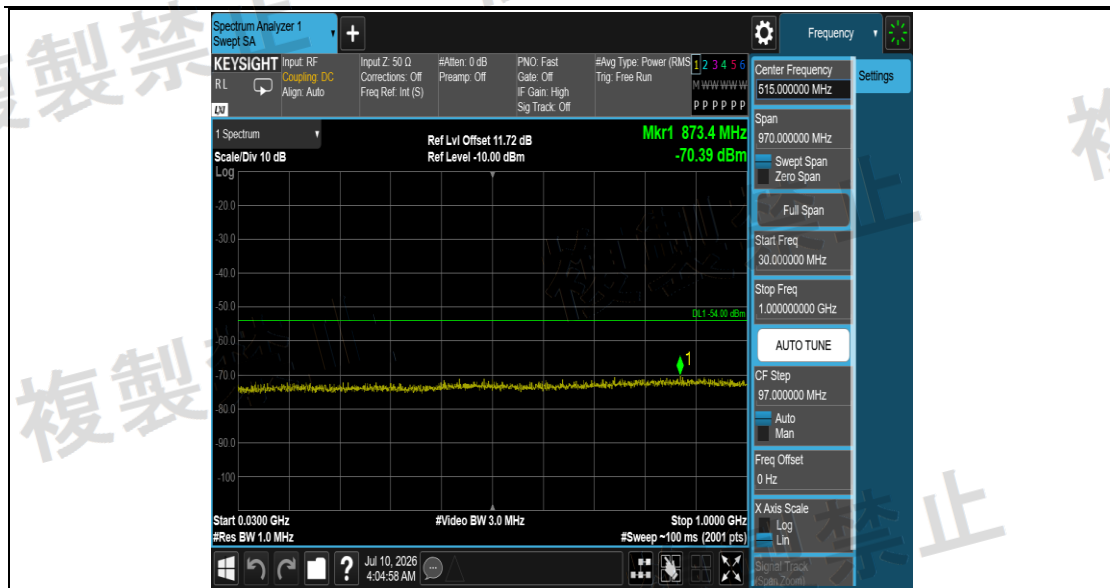
NTNV_BLE_1M_Ant1_2440_30~1000
